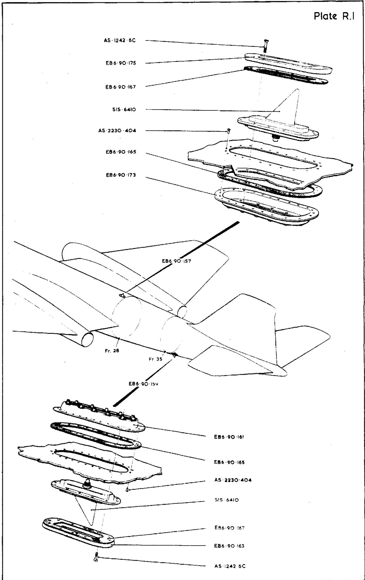
I.F.F. AERIAL INSTALLATION
