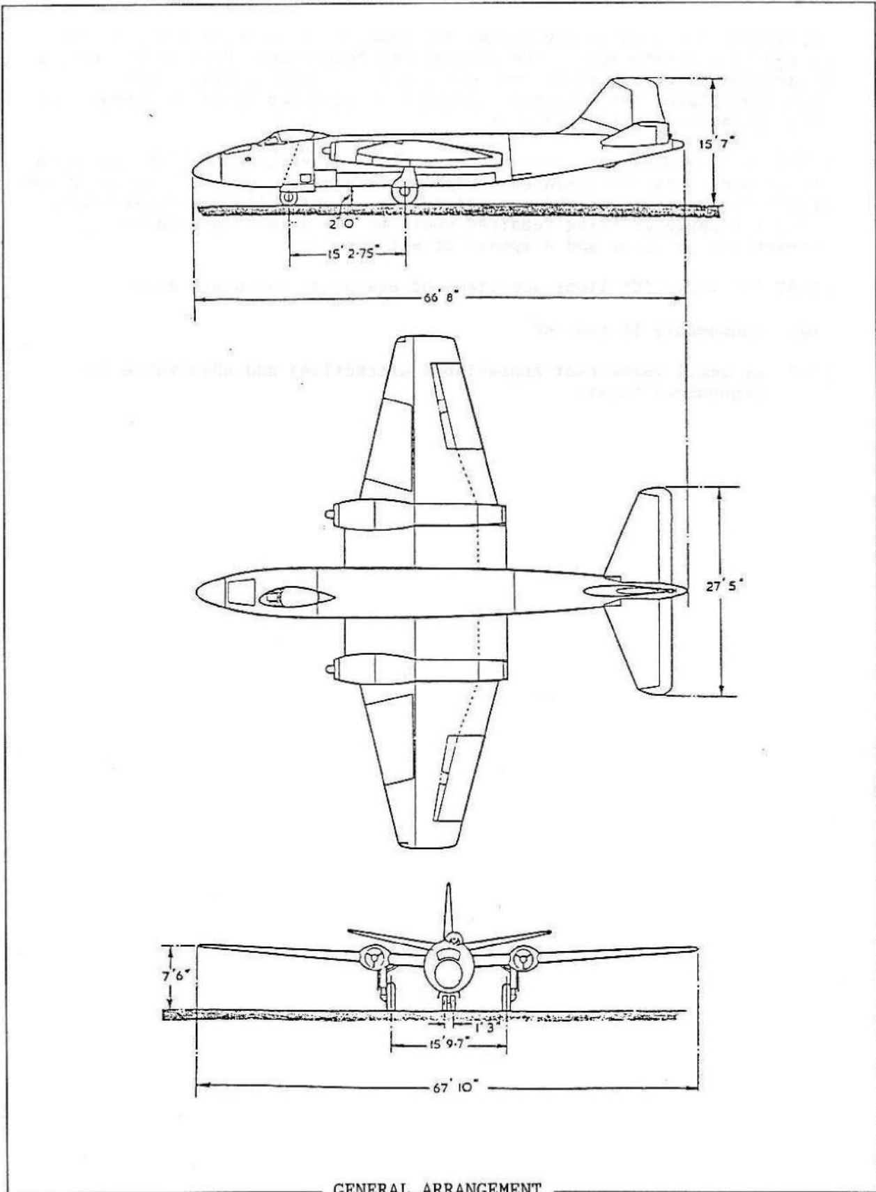
GENERAL ARRANGEMENT
