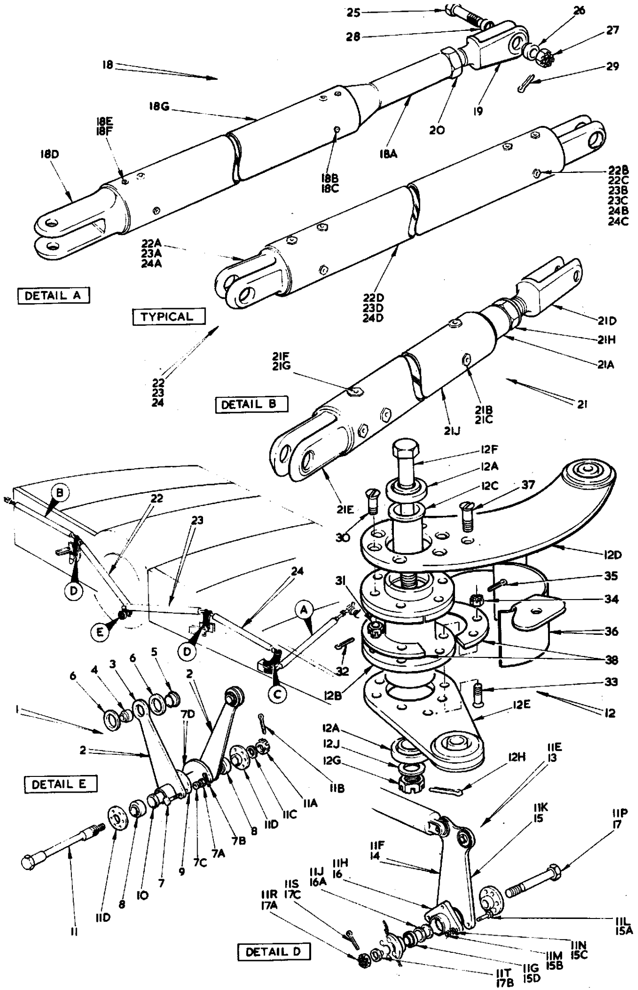
FIG. I AILERON CONTROLS IN WING
