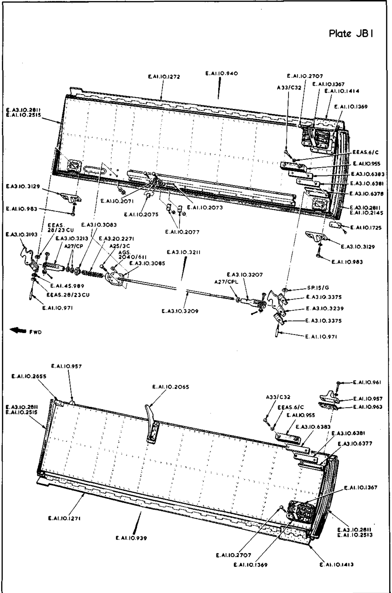
NOSE UNDERCARRIAGE DOORS
