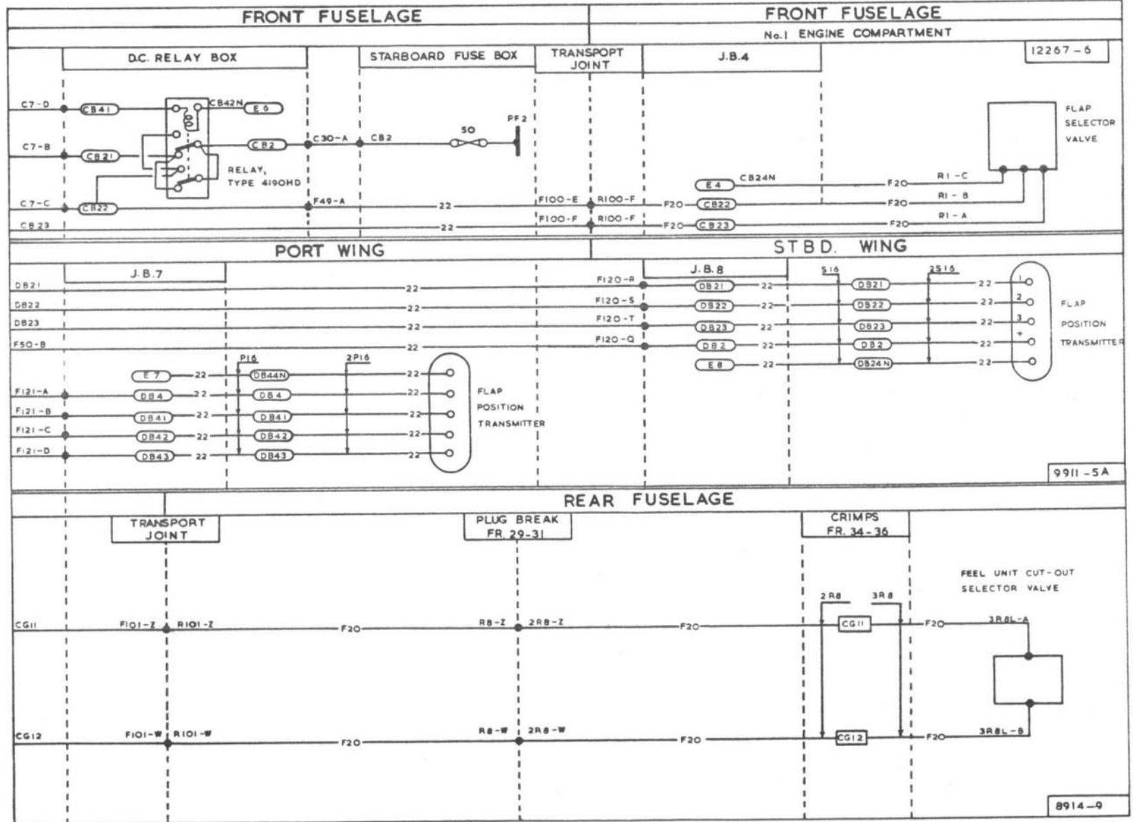
FIG. 6A. FLAPS - FEEL UNIT CUT-OUT
