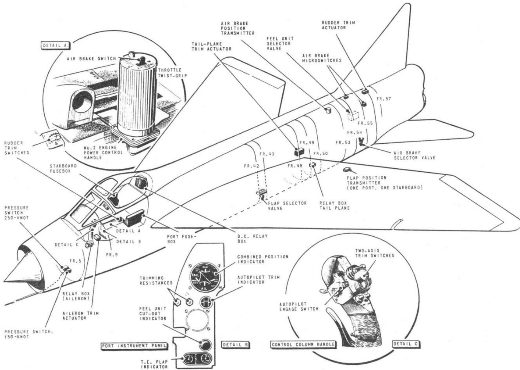
FIG. 1. FLYING CONTROLS EQUIPMENT
