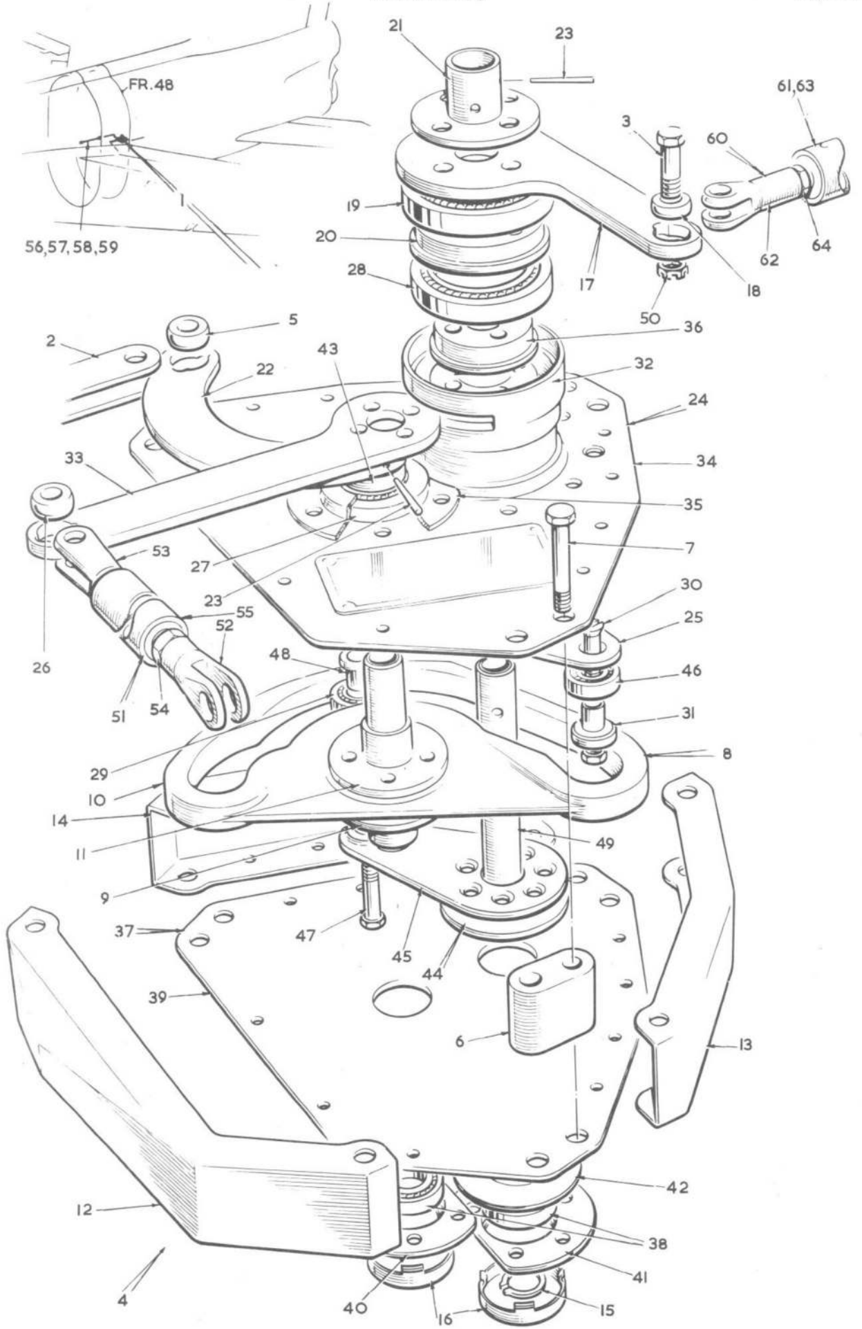
FIG. 14. ENGINE CONTROLS IN REAR FUSELAGE Restricted
