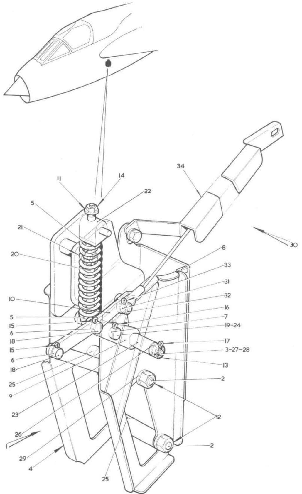
FIG 23A EMERGENCY CONTROLS IN FRONT FUSELAGE.
