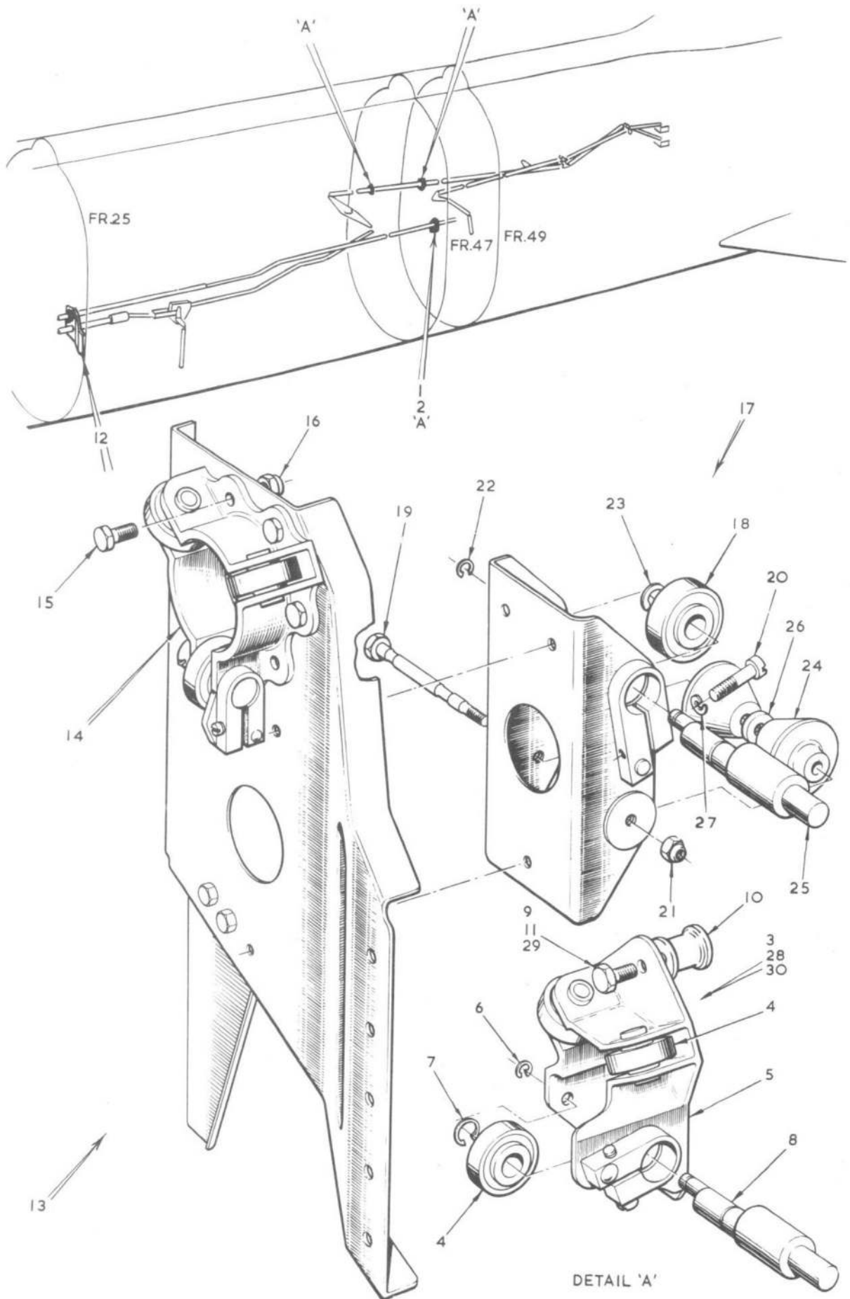
FIG. 15. ENGINE CONTROLS IN REAR FUSELAGE Restricted
