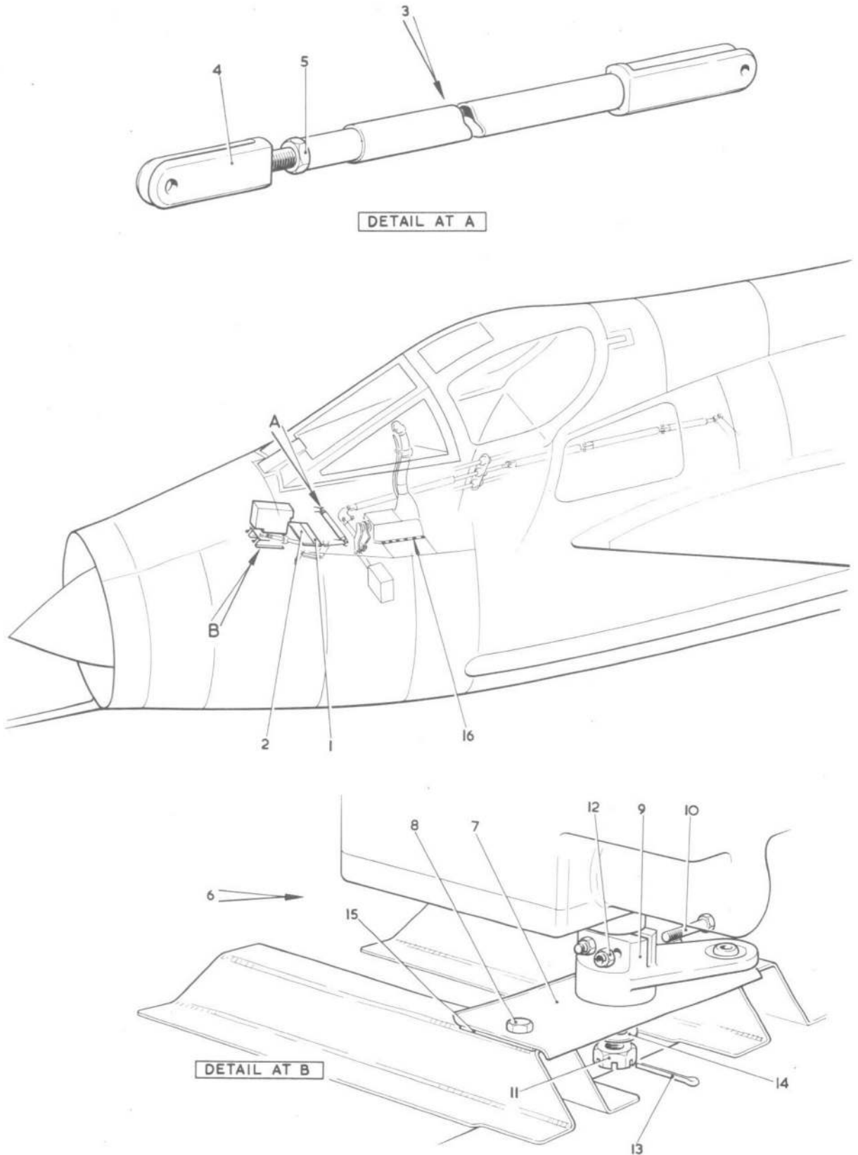
FIG. 30A. CONTROLS - FLYING CONTROLS IN FRONT FUSELAGE
