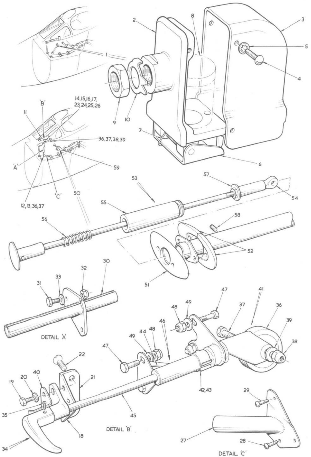
FIG.20 EMERGENCY CONTROLS IN FRONT FUSELAGE, FRAMES 8 TO 15
