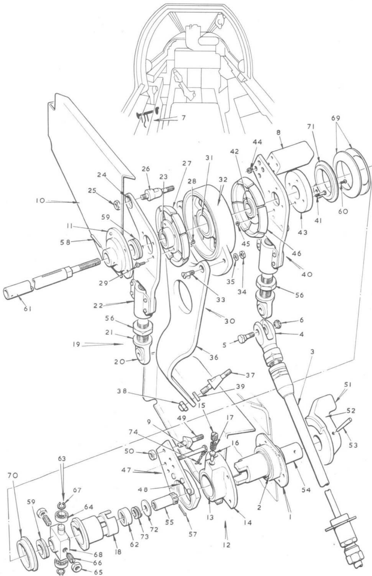
FIG.3. ENGINE CONTROLS IN FRONT FUSELAGE Restricted
