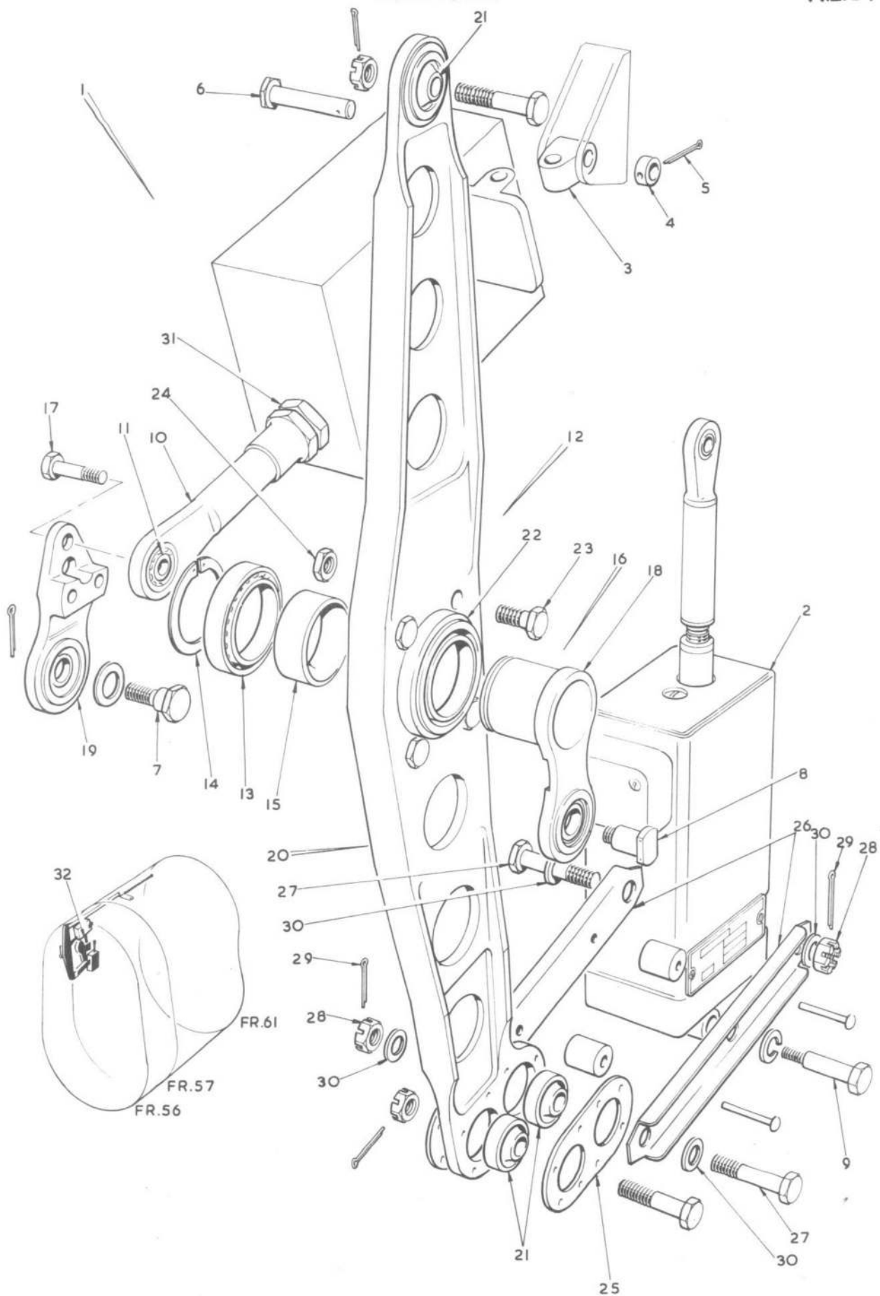
FIG.33. FLYING CONTROLS IN REAR FUSELAGE Restricted
