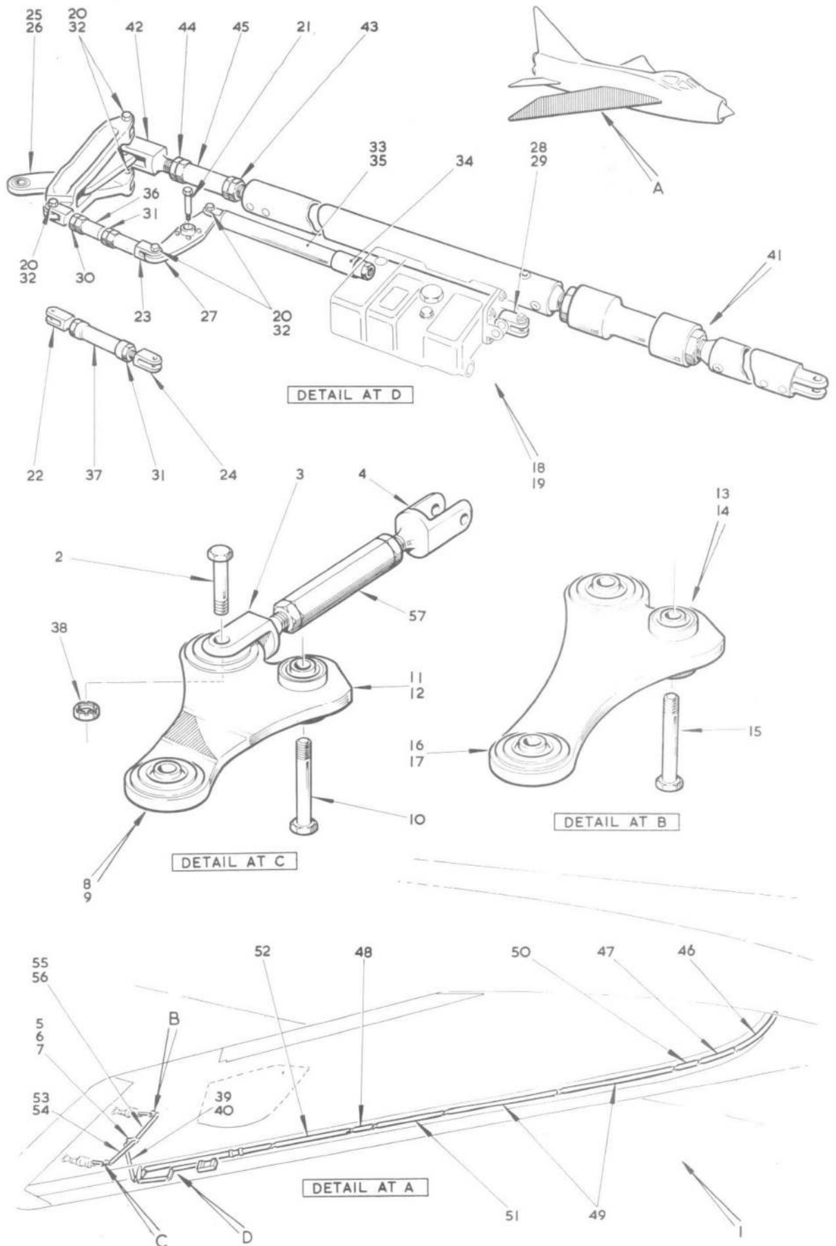
FIG. 38 FLYING CONTROLS IN STARBOARD WING Restricted
