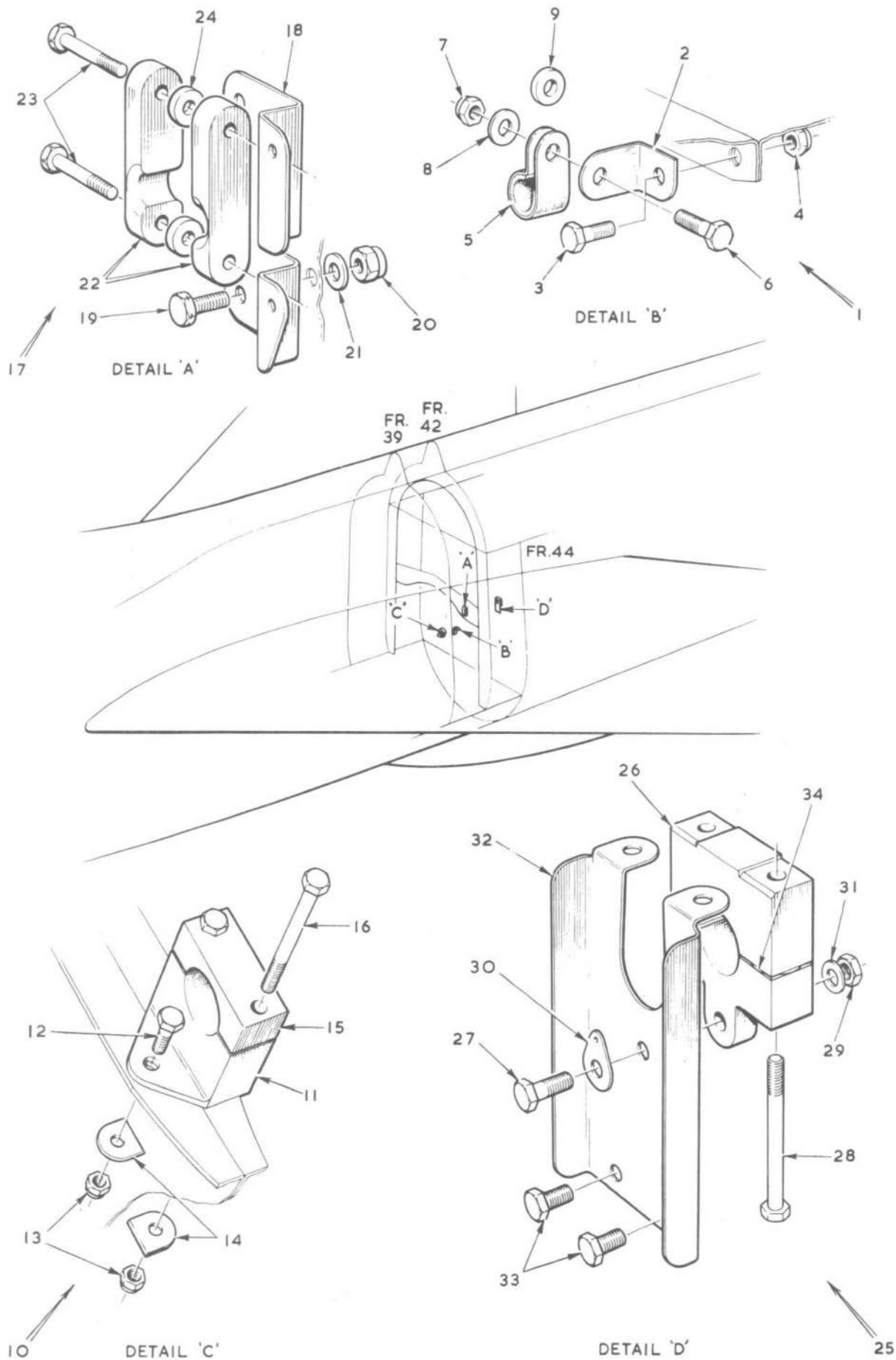
FIG.12. ENGINE CONTROLS IN REAR FUSELAGE Restricted
