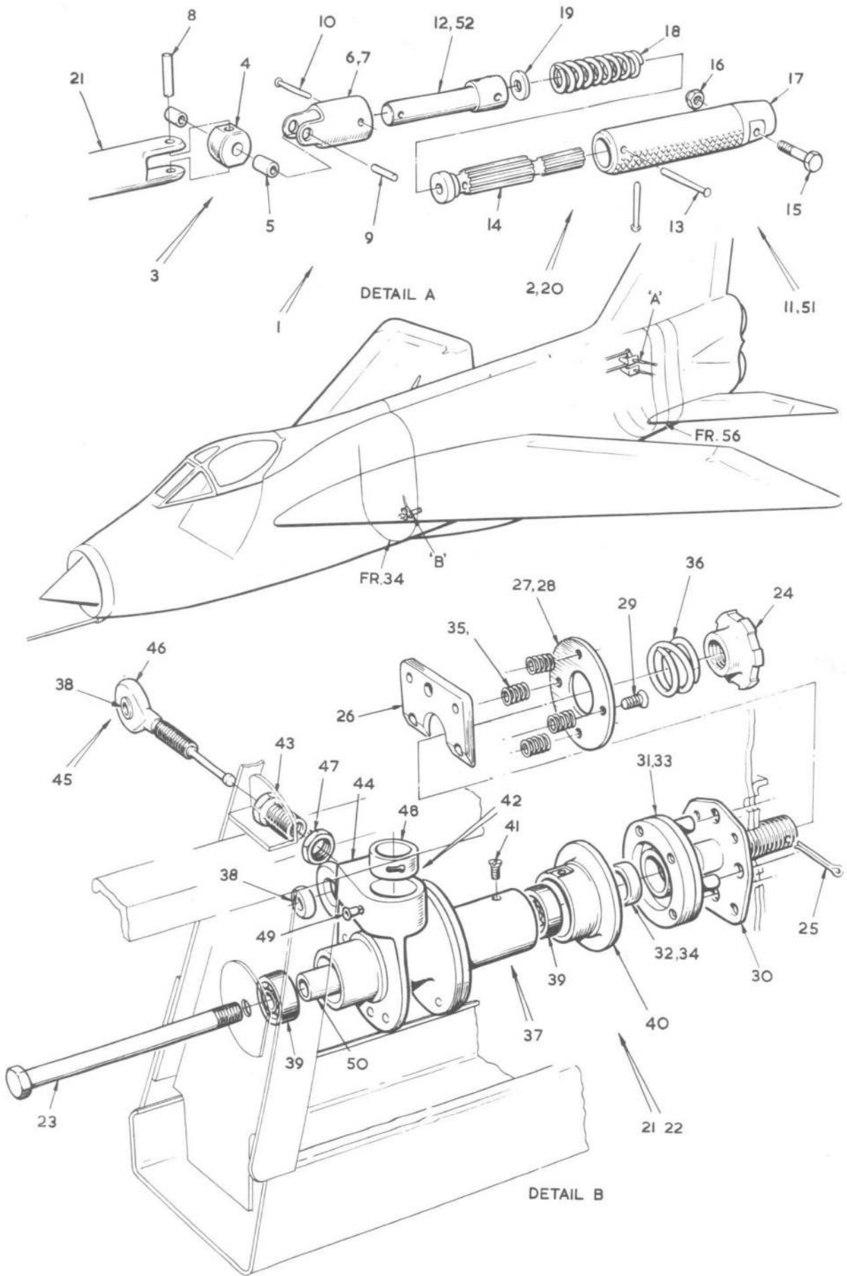
FIG.7. ENGINE CONTROLS IN REAR FUSELAGE Restricted
