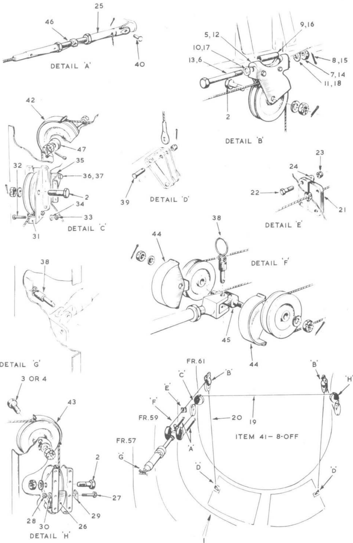
FIG.40. TAIL PARACHUTE STREAM & DROP TANK RELEASE CABLES Restricted
