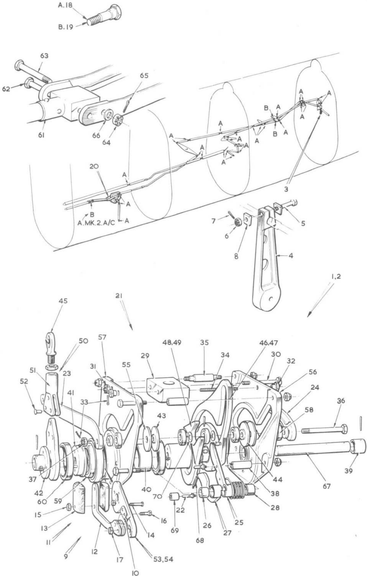
FIG.4. ENGINE CONTROLS IN REAR FUSELAGE Restricted
