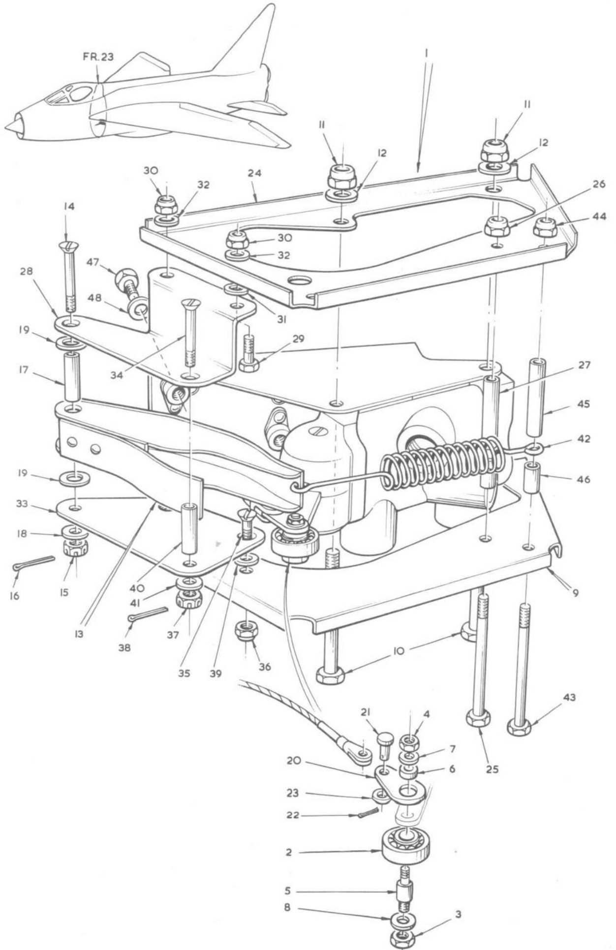
FIG. 23. FLYING CONTROLS Restricted
