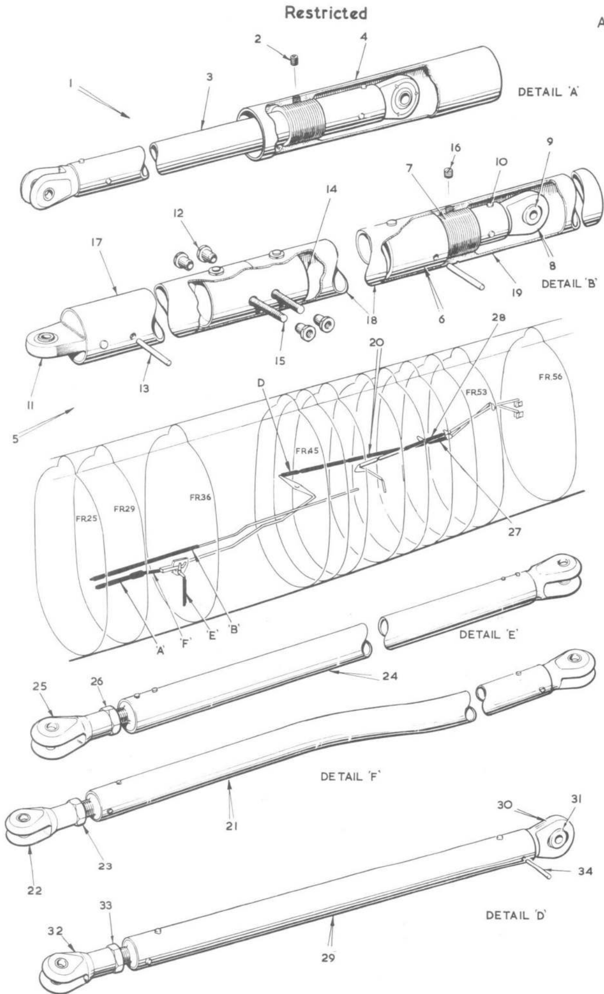
FIG.18. ENGINE CONTROLS IN REAR FUSELAGE Restricted
