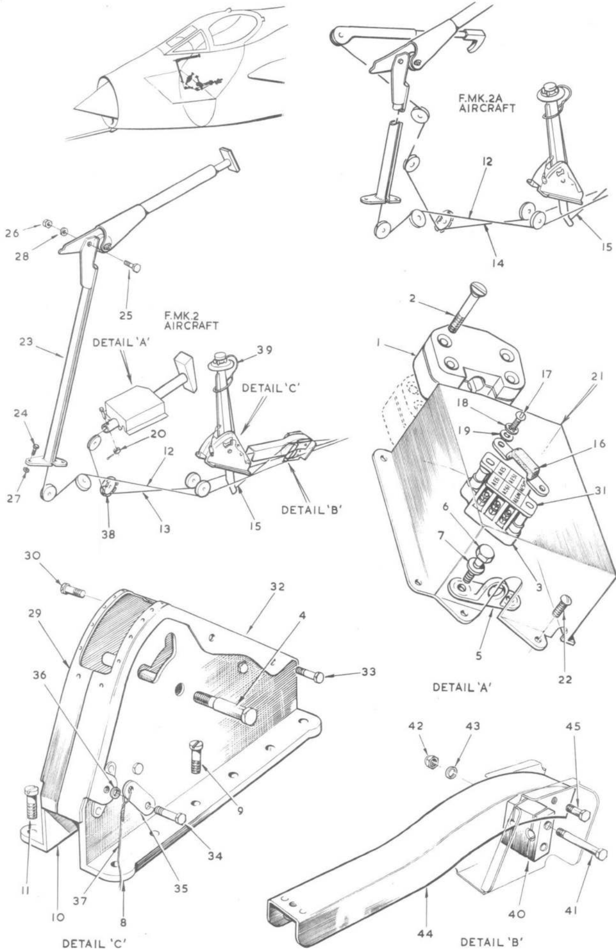
FIG. 19. EMERGENCY CONTROLS IN FRONT FUSELAGE Restricted
