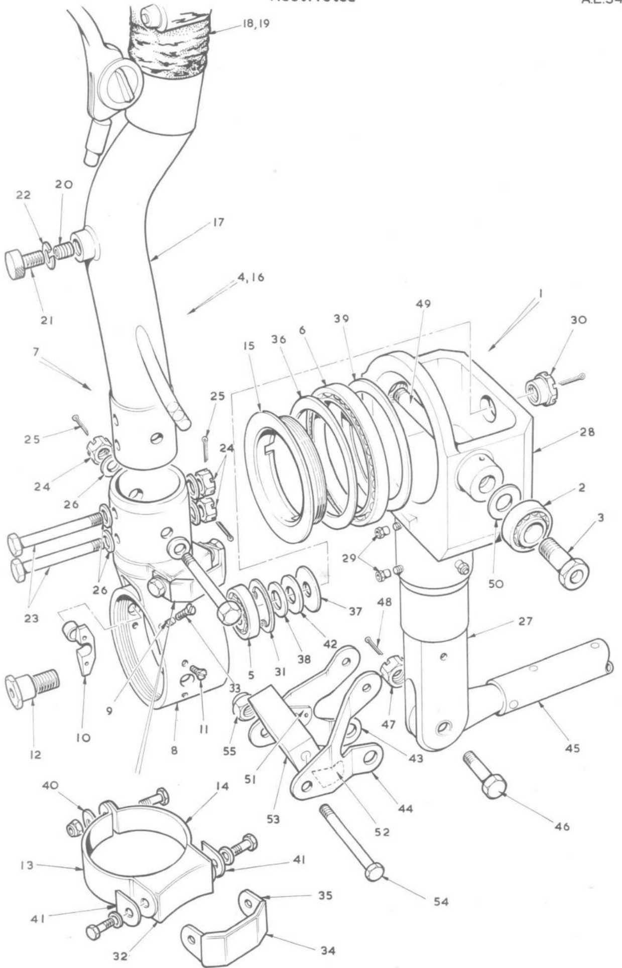
FIG. 29A. FLYING CONTROLS IN FRONT FUSELAGE
