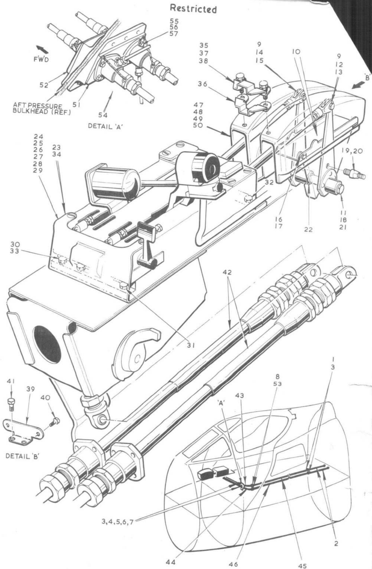
FIG.1. ENGINE CONTROLS IN FRONT FUSELAGE Restricted
