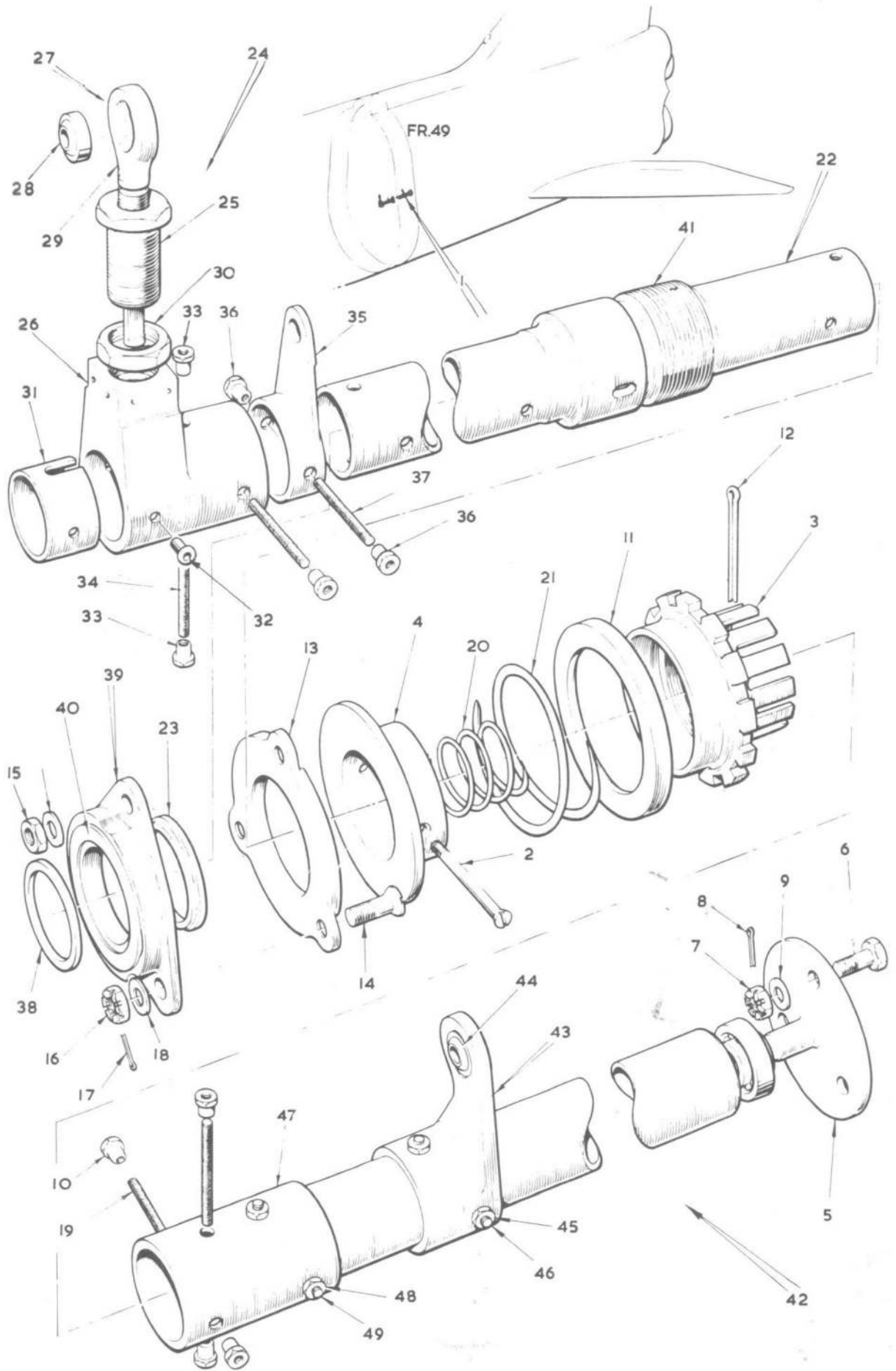
FIG.16. ENGINE CONTROLS IN REAR FUSELAGE
