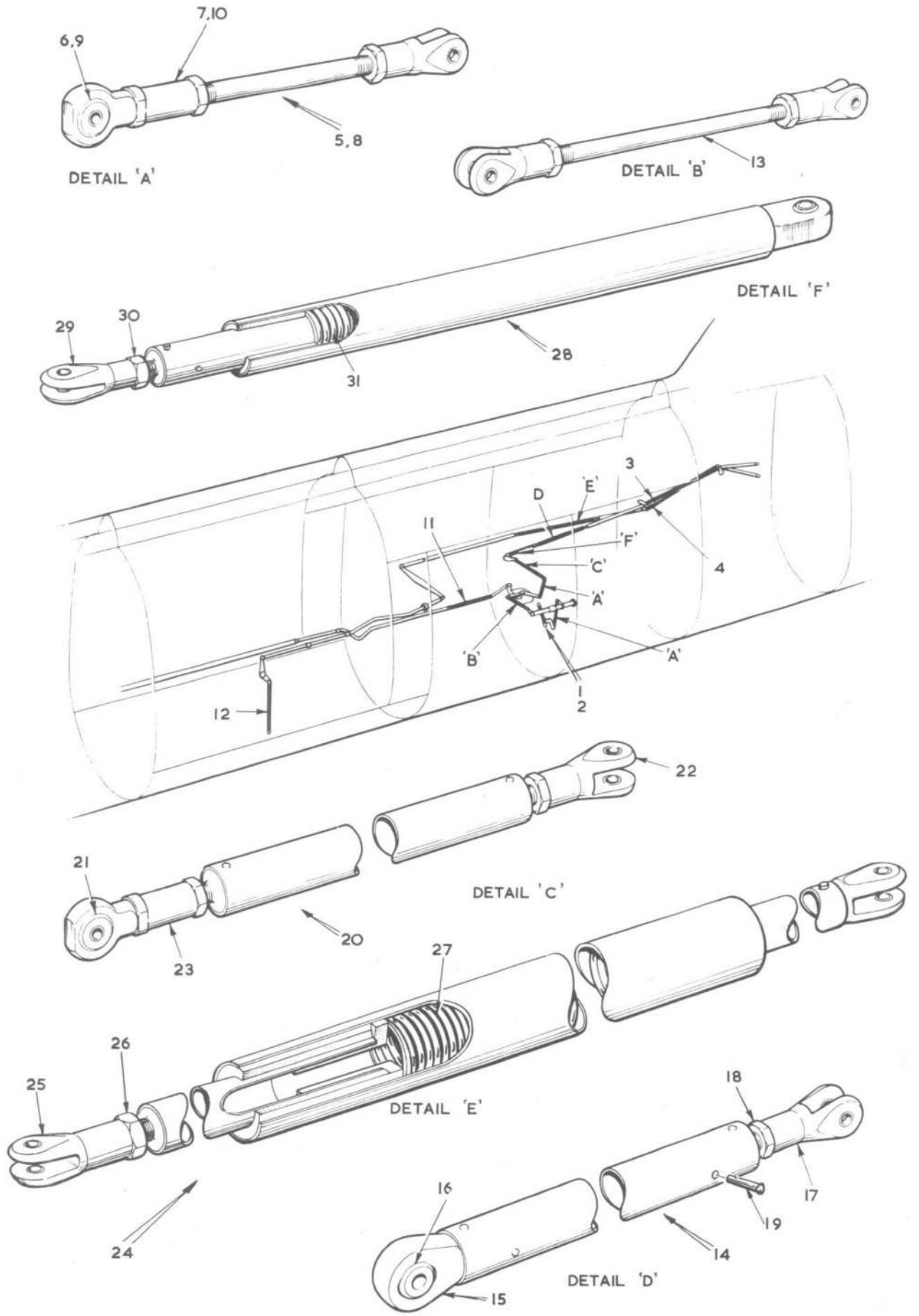
FIG.17. ENGINE CONTROLS IN REAR FUSELAGE Restricted
