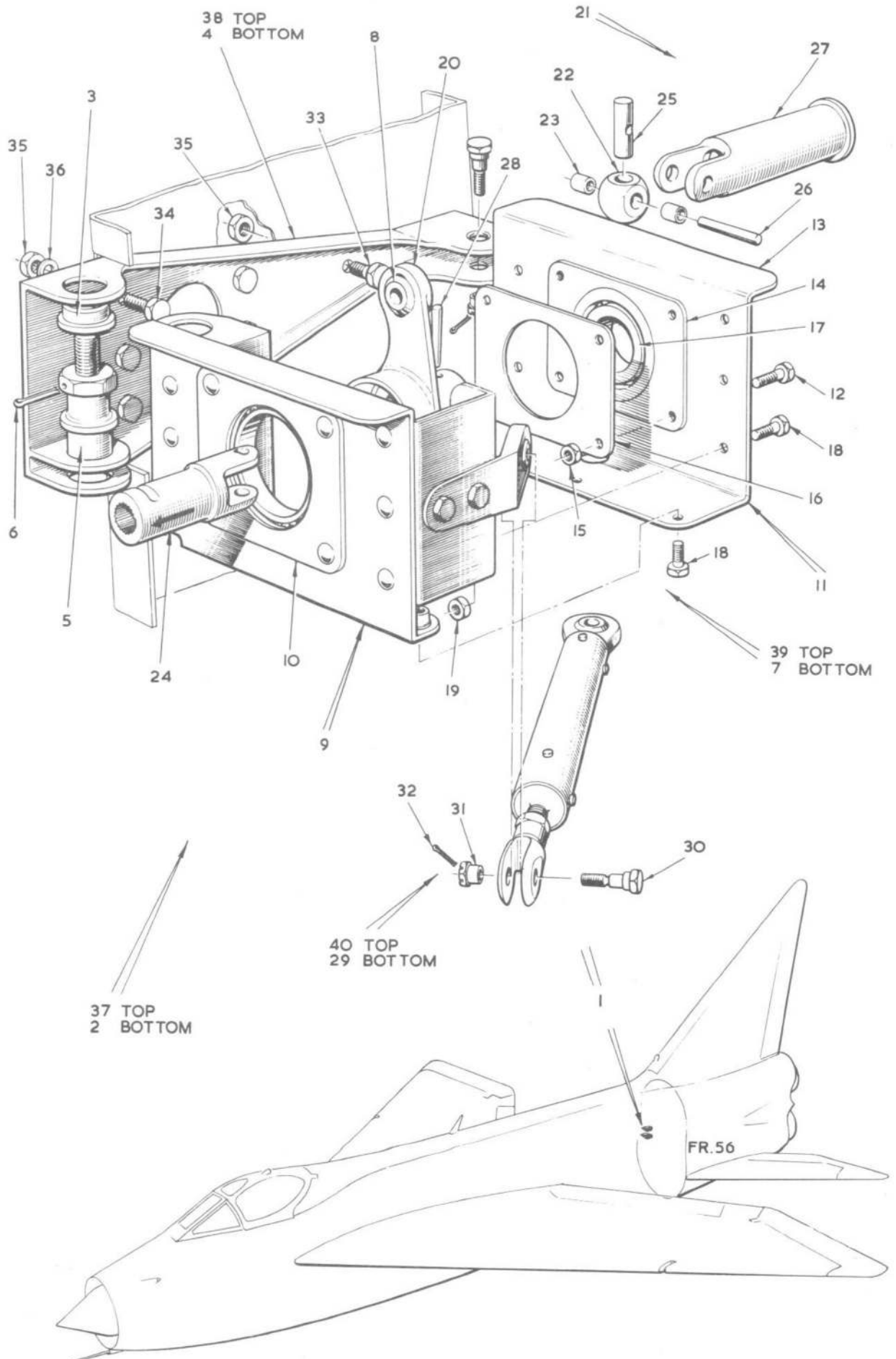
FIG.10. ENGINE CONTROLS IN REAR FUSELAGE Restricted
