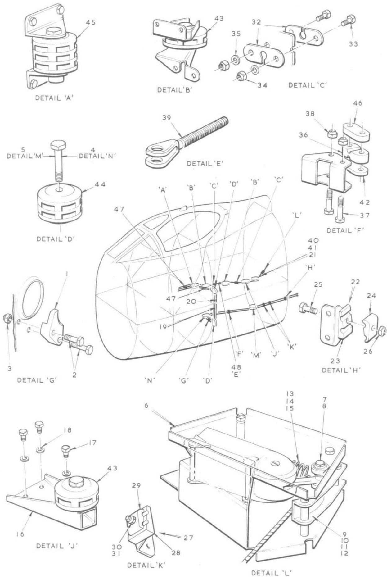
FIG.22. EMERGENCY CONTROLS IN FRONT FUSELAGE Restricted
