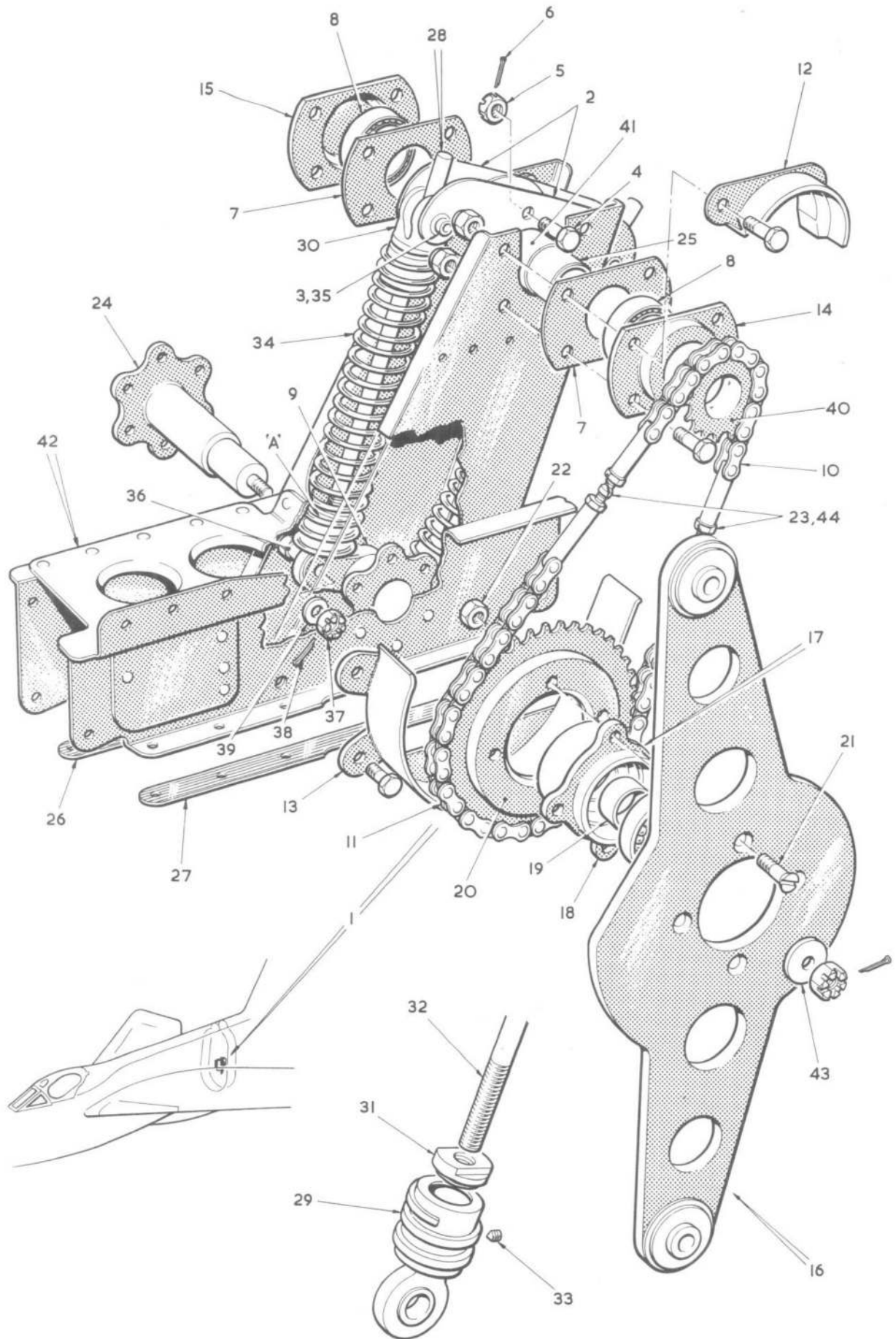
FIG.35. FLYING CONTROLS IN REAR FUSELAGE Restricted
