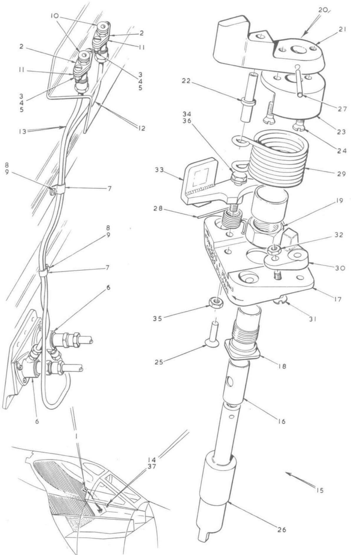
FIG.3A. ENGINE CONTROLS IN FRONT FUSELAGE
