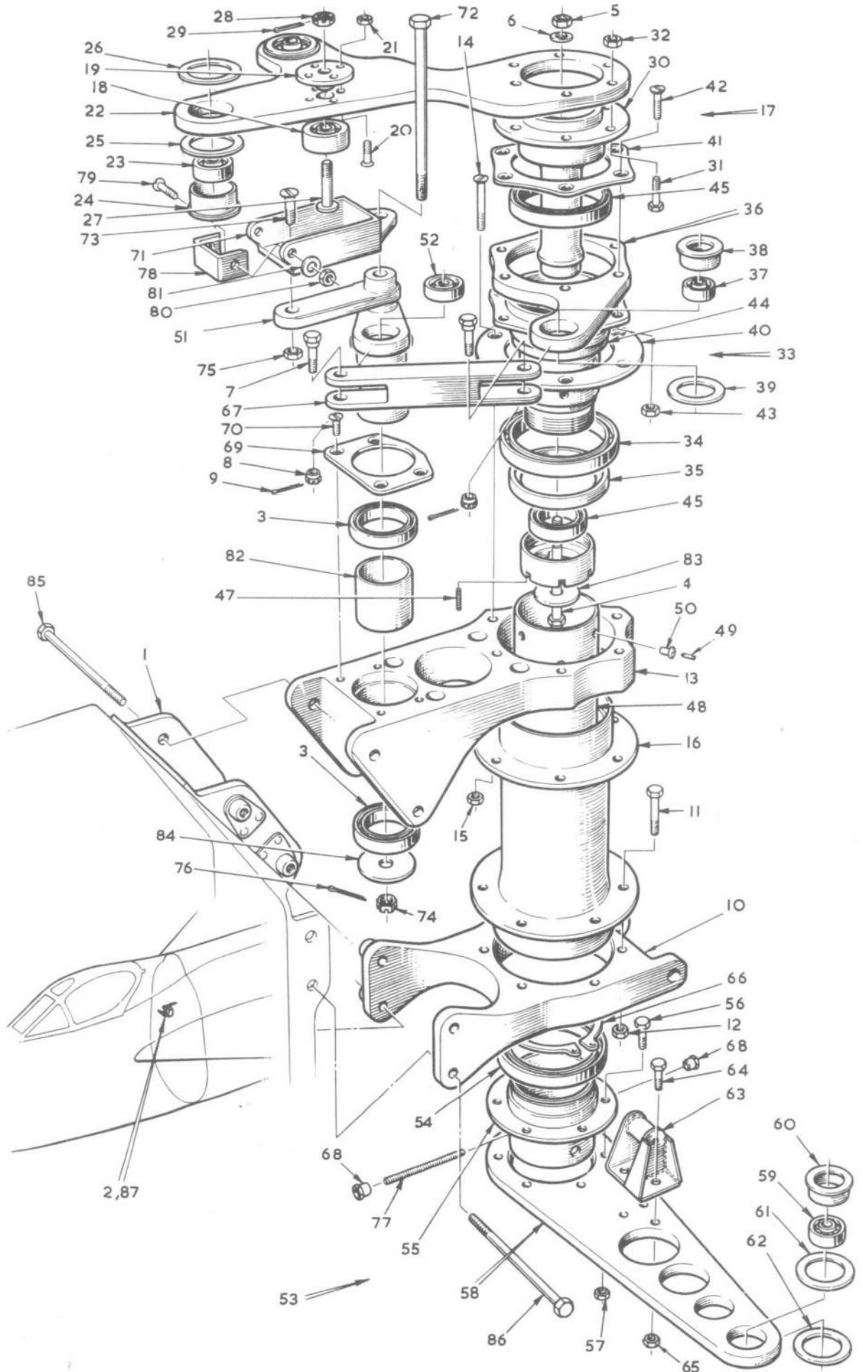
FIG. 26. FLYING CONTROLS Restricted
