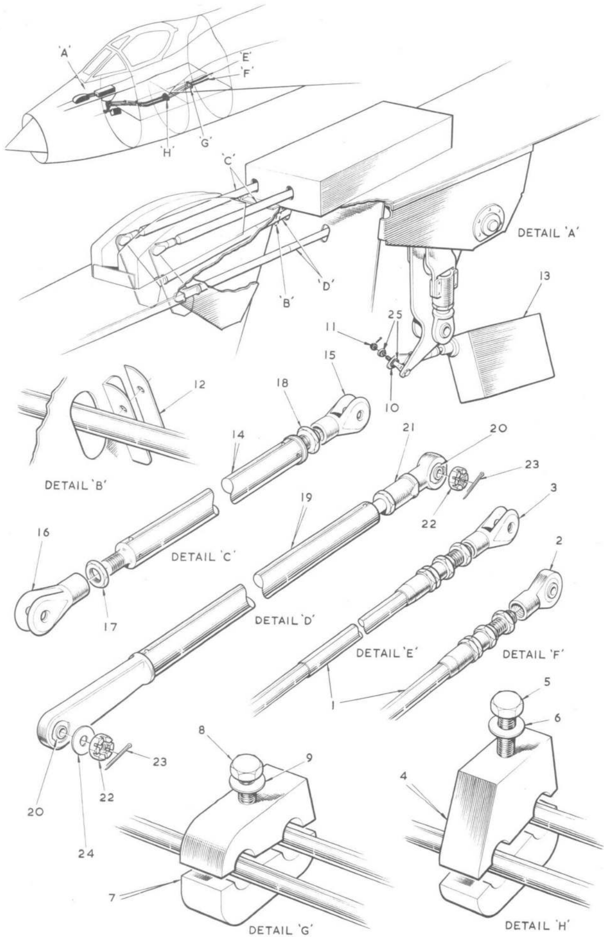
FIG. 2. ENGINE CONTROLS IN FRONT FUSELAGE
