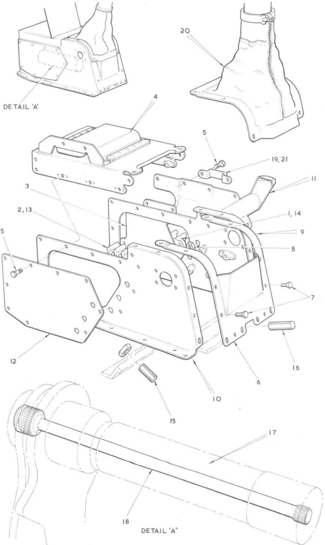
FIG.29. FLYING CONTROLS IN FRONT FUSELAGE Restricted
