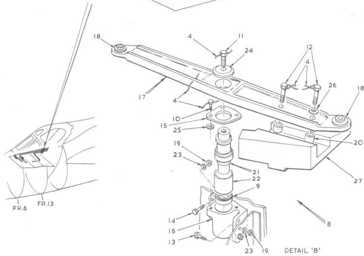
FIG.31. FLYING CONTROLS IN FRONT FUSELAGE Restricted
