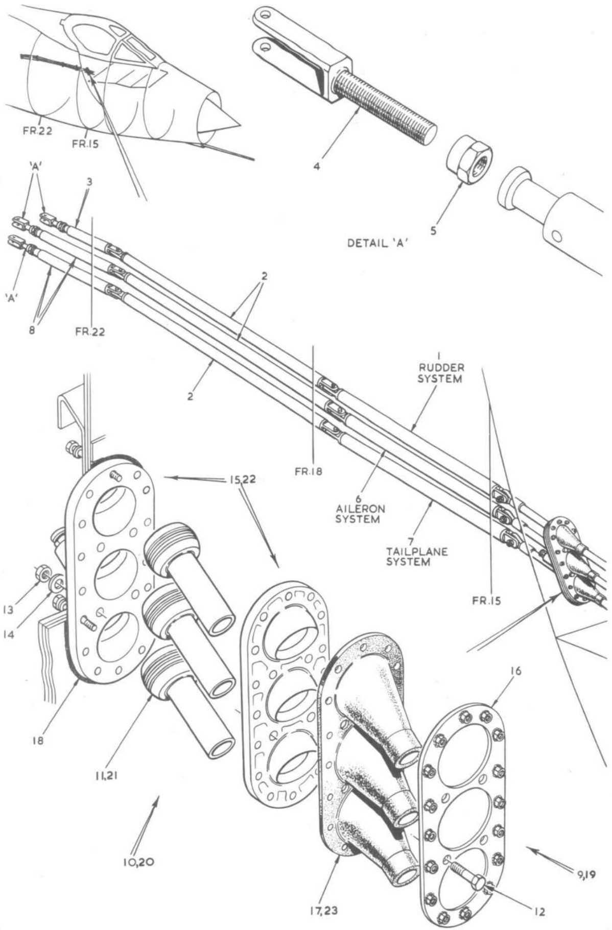
FIG.31A. FLYING CONTROLS IN FRONT FUSELAGE Restricted
