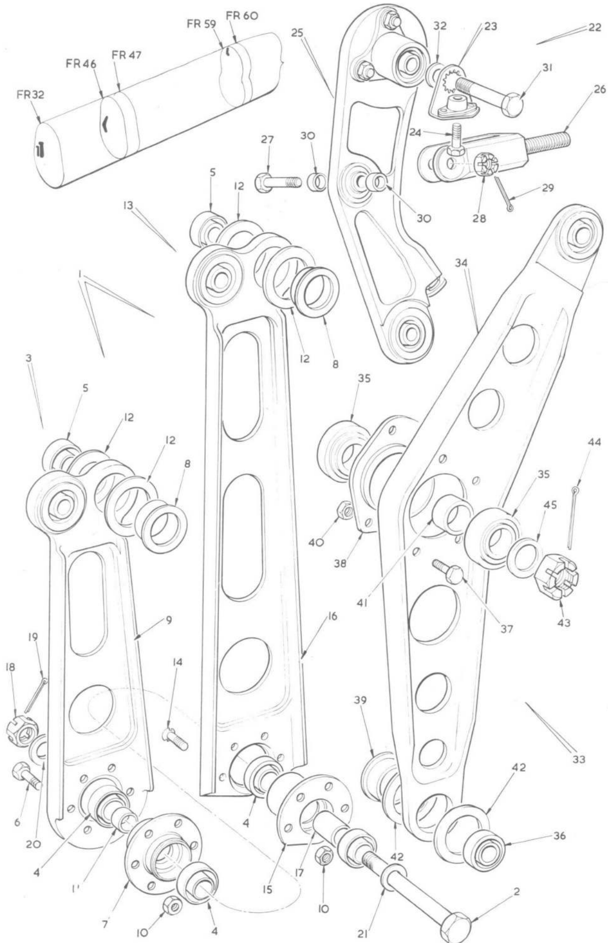
FIG.34. FLYING CONTROLS IN REAR FUSELAGE
