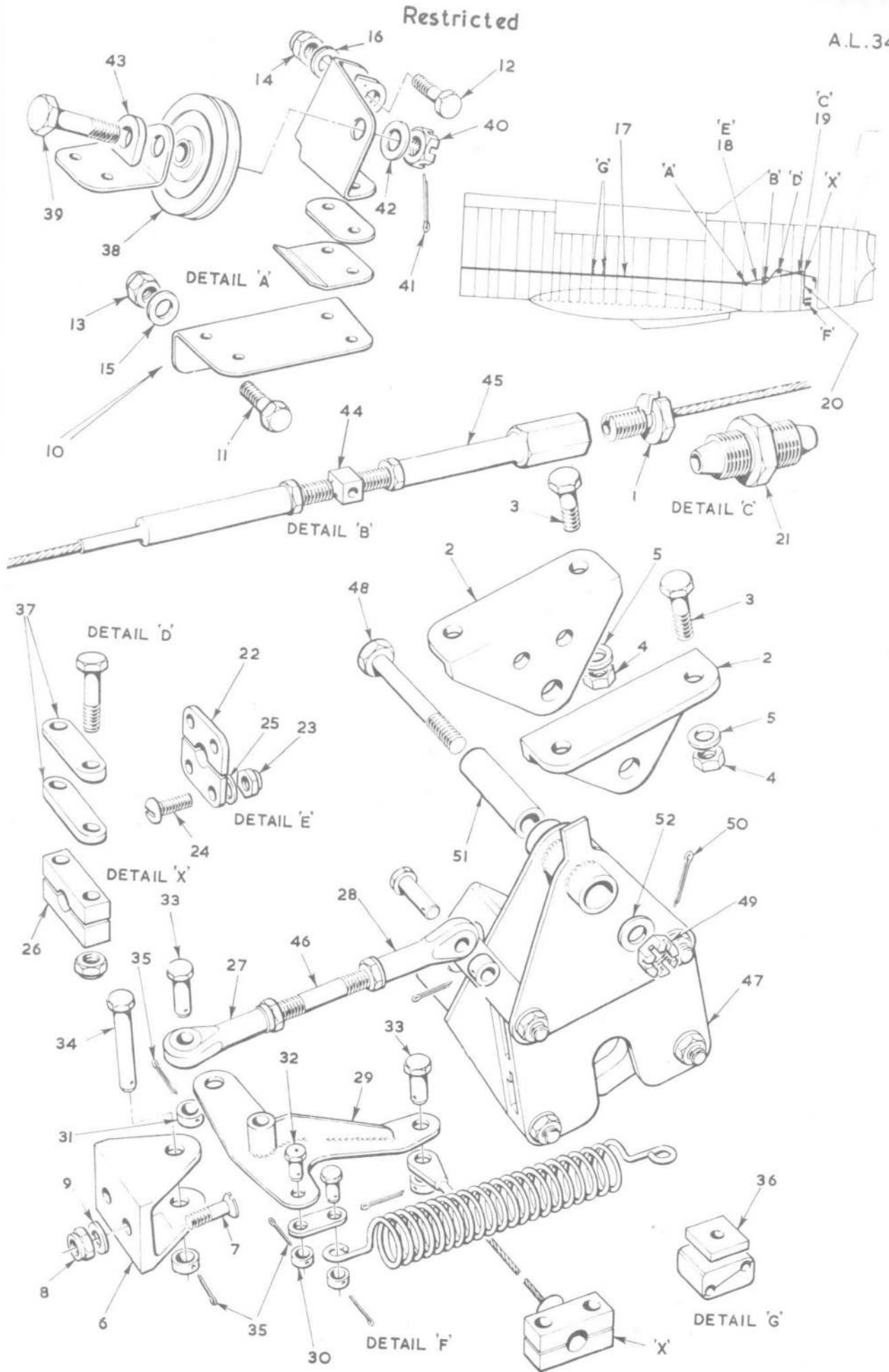
FIG.41. TAIL PARACHUTE, AND ARRESTER HOOK CABLES
