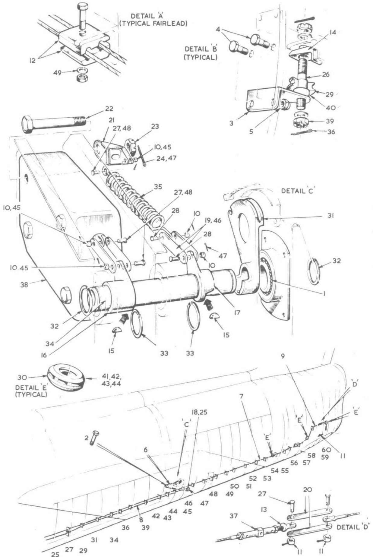
FIG. 39. TAIL PARACHUTE AND ARRESTER HOOK CABLES TAIL PARACHUTE STREAM AND DROP TANK RELEASE CABLES
