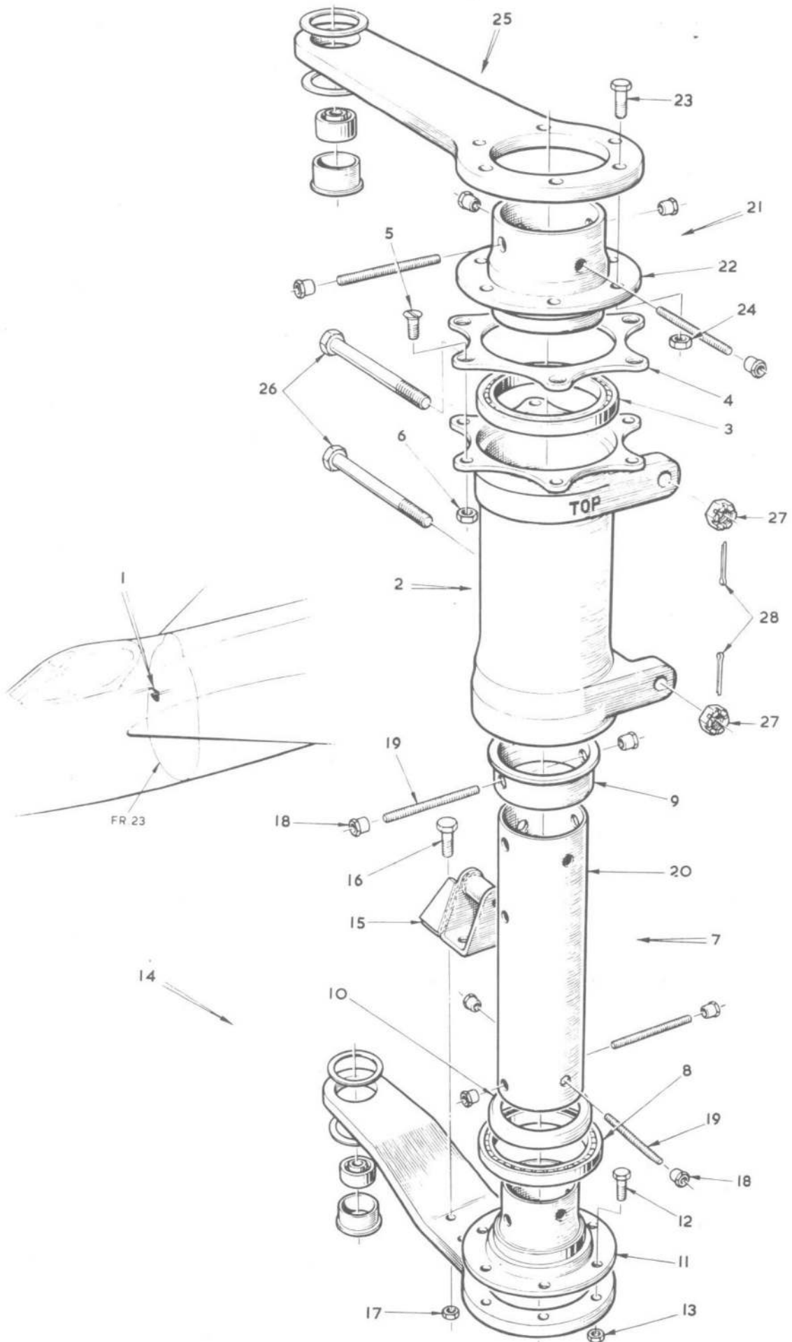
FIG. 27. FLYING CONTROLS Restricted
