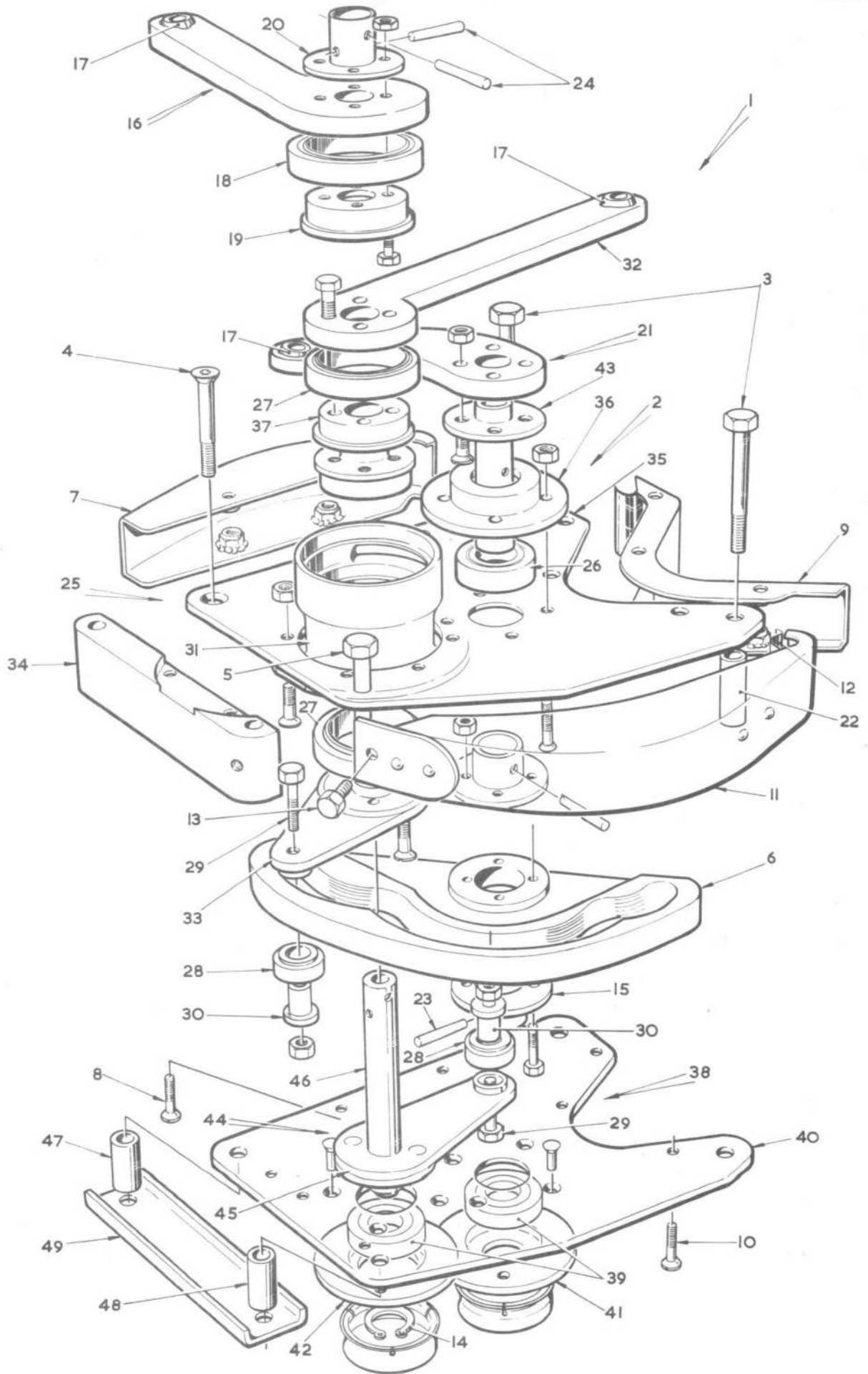
FIG.5. ENGINE CONTROLS IN REAR FUSELAGE Restricted
