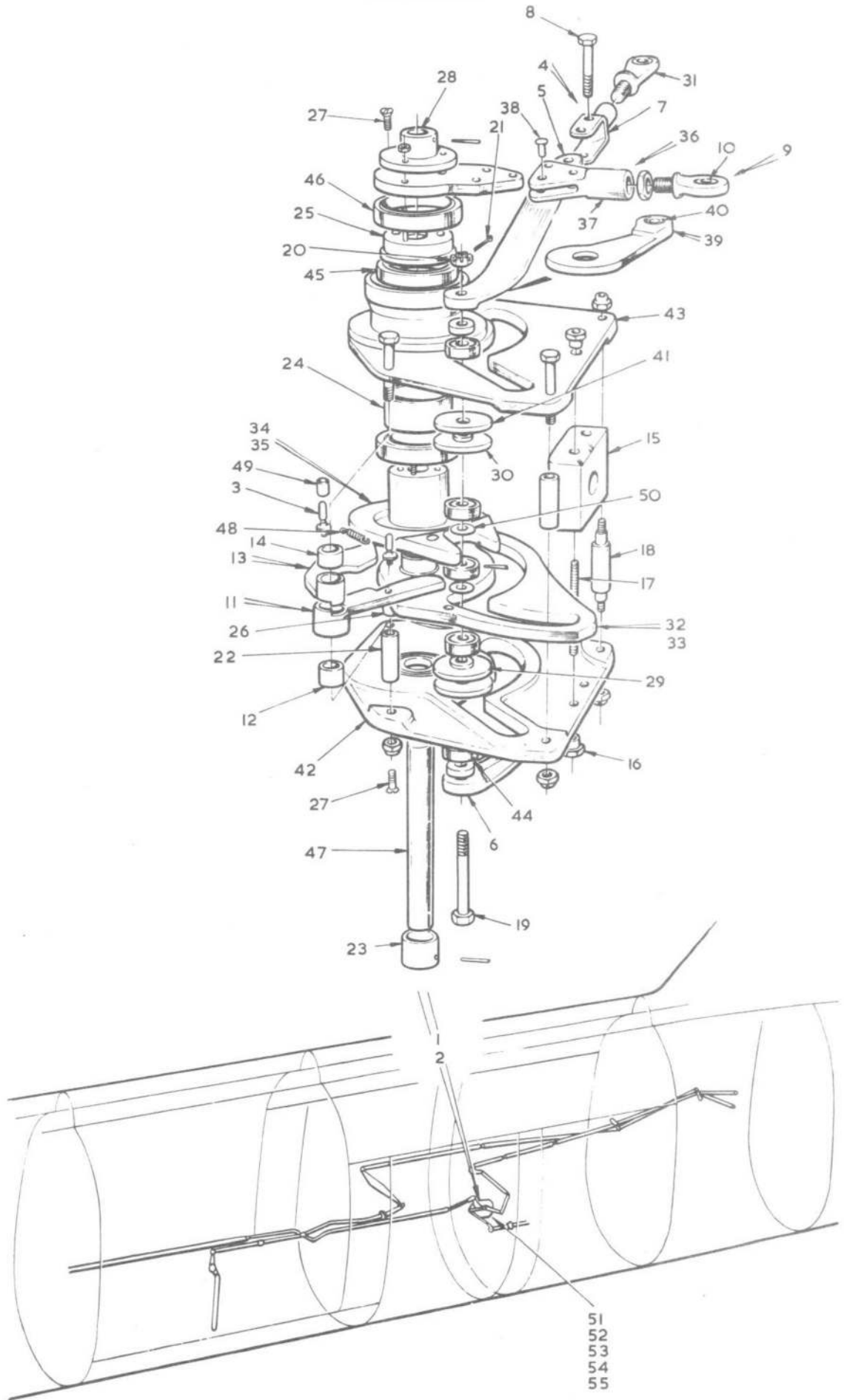
FIG.13. ENGINE CONTROLS IN REAR FUSELAGE Restricted
