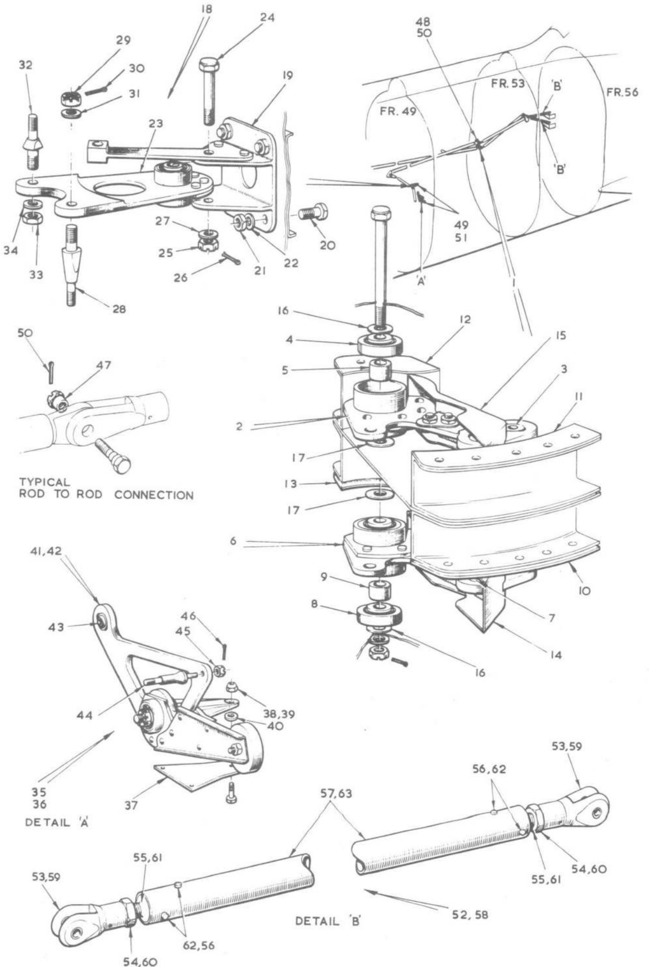
FIG.9. ENGINE CONTROLS IN REAR FUSELAGE
