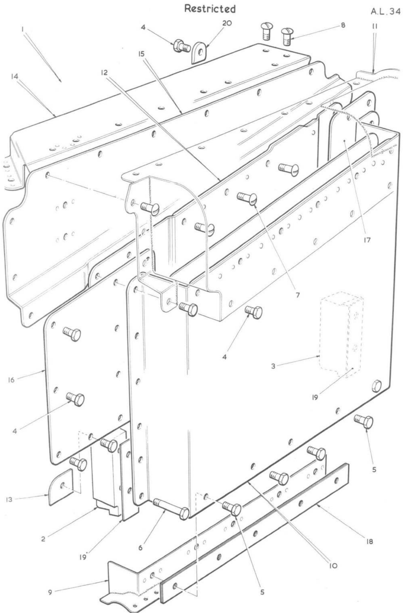
FIG. 35A. FLYING CONTROLS IN REAR FUSELAGE Restricted
