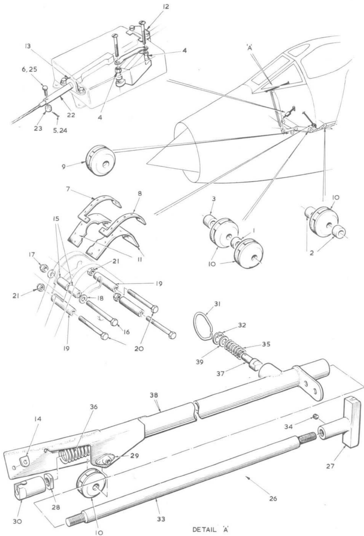
FIG.21. EMERGENCY CONTROLS IN FRONT FUSELAGE FRAMES 8 TO 15
