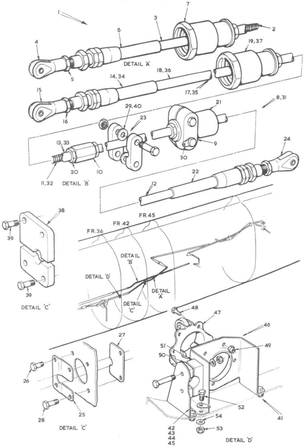
FIG.6. ENGINE CONTROLS IN REAR FUSELAGE
