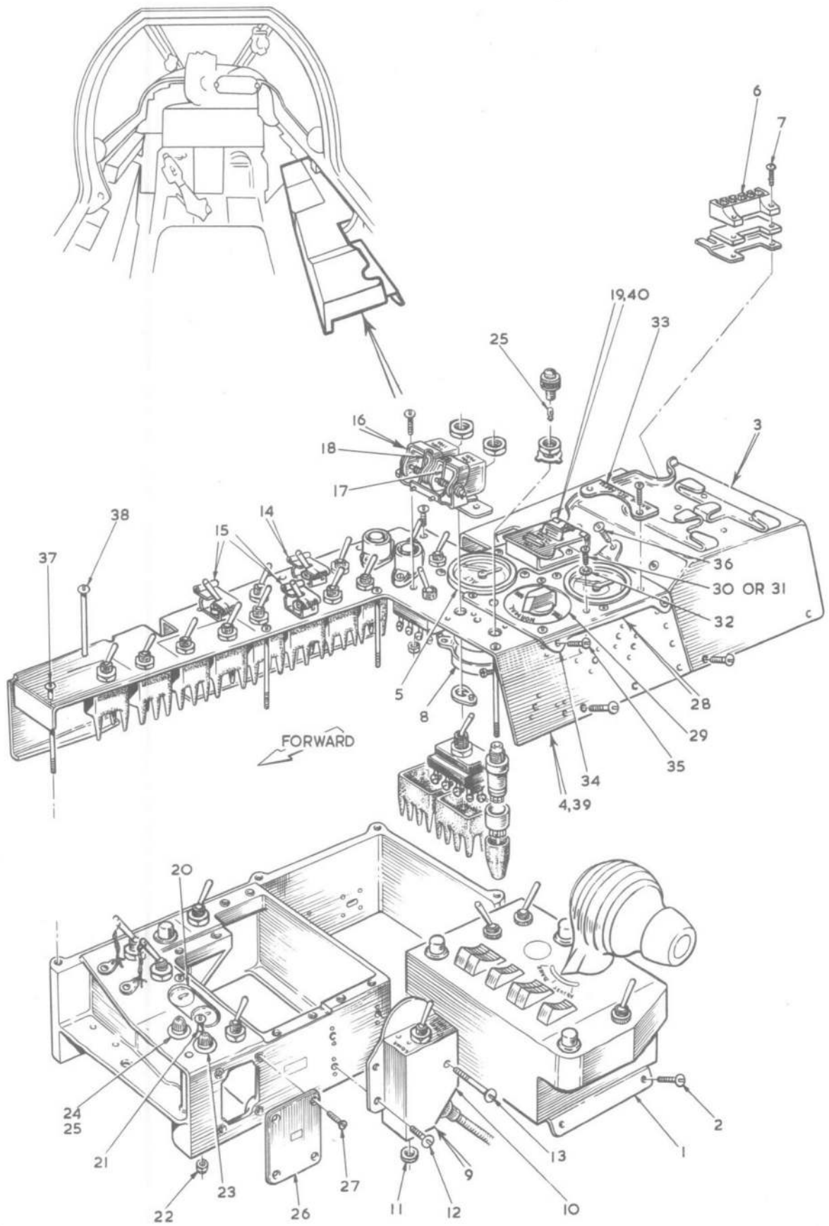
FIG.4. PILOT'S INSTRUMENTS AND CONTROLS
