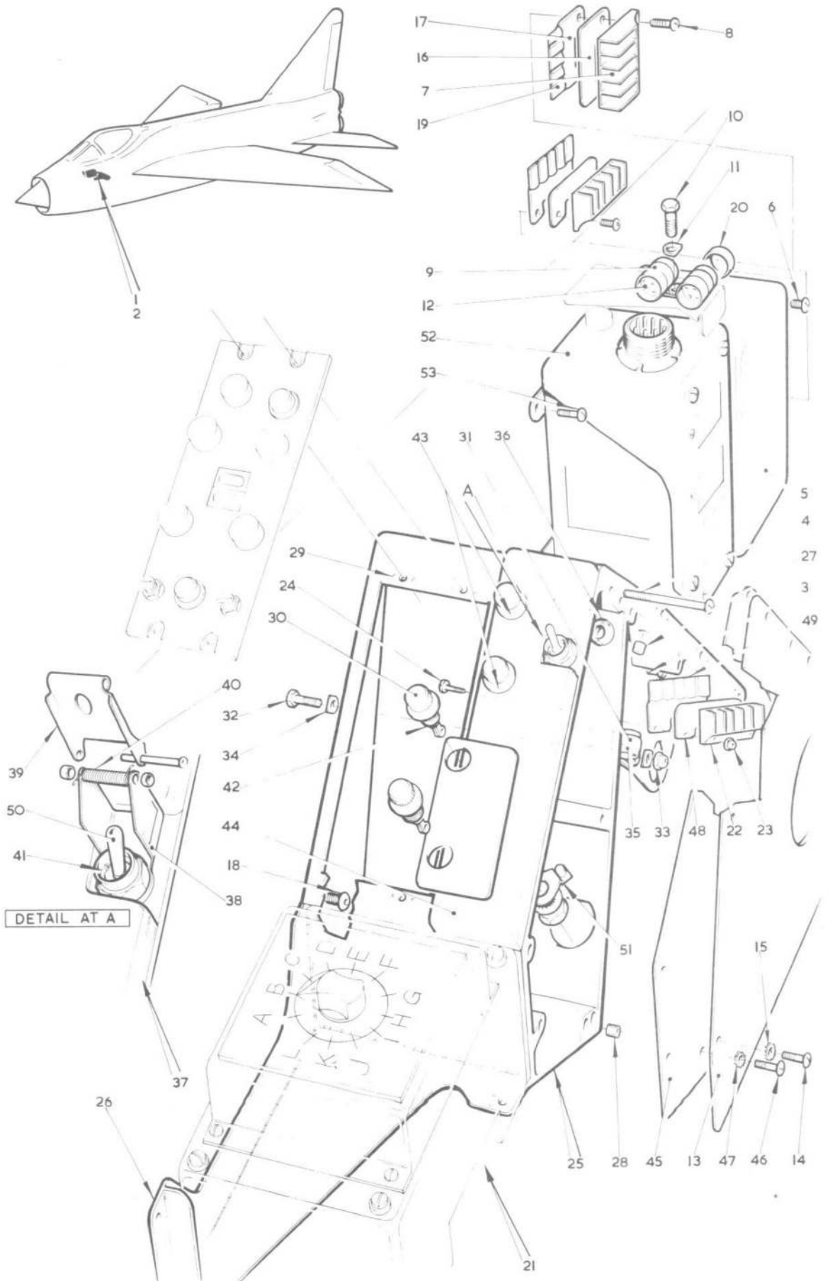
FIG.2 INSTRUMENTS PILOTS INSTRUMENTS AND CONTROLS
