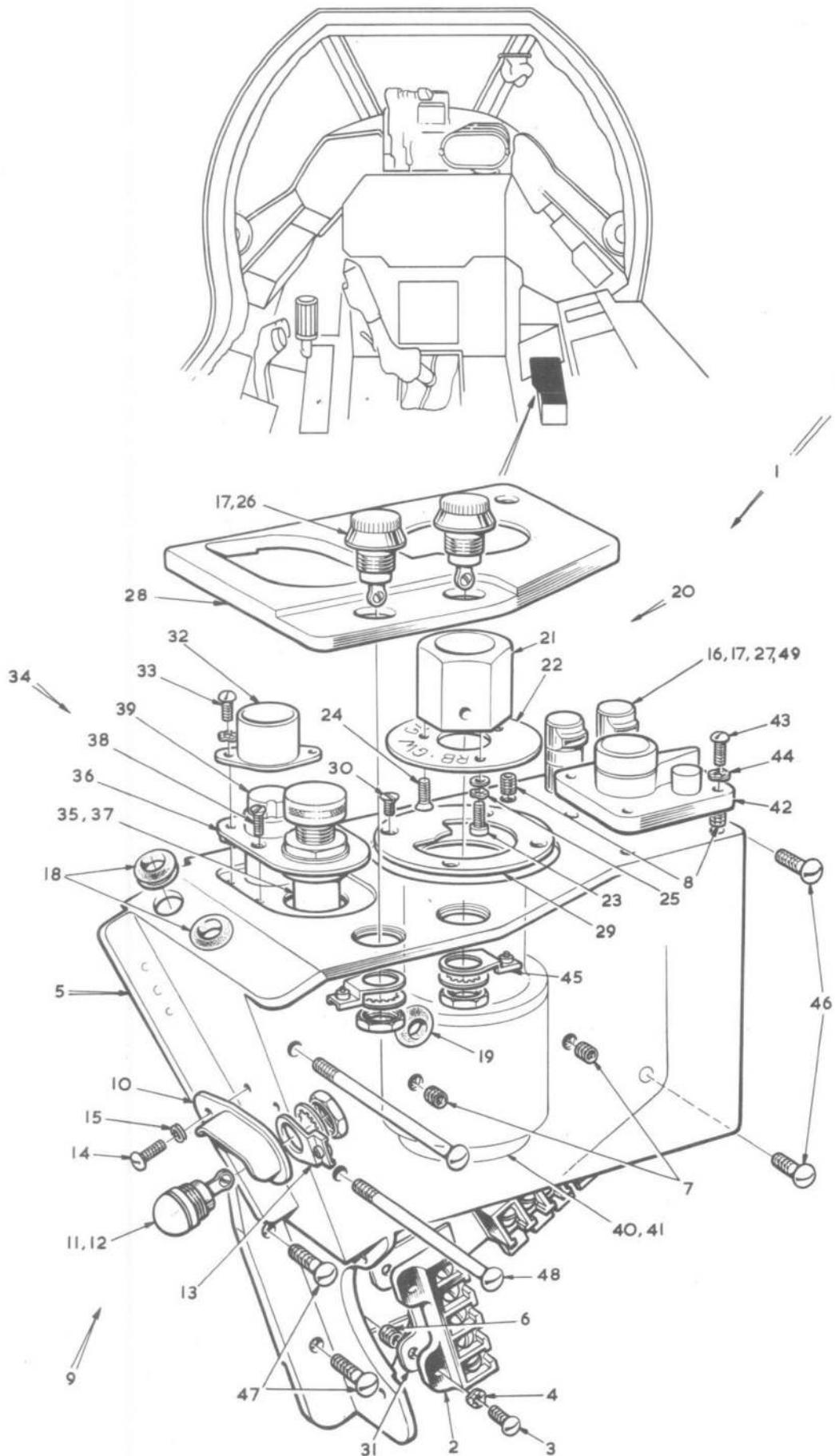
FIG.7. PILOT'S INSTRUMENTS AND CONTROLS Restricted
