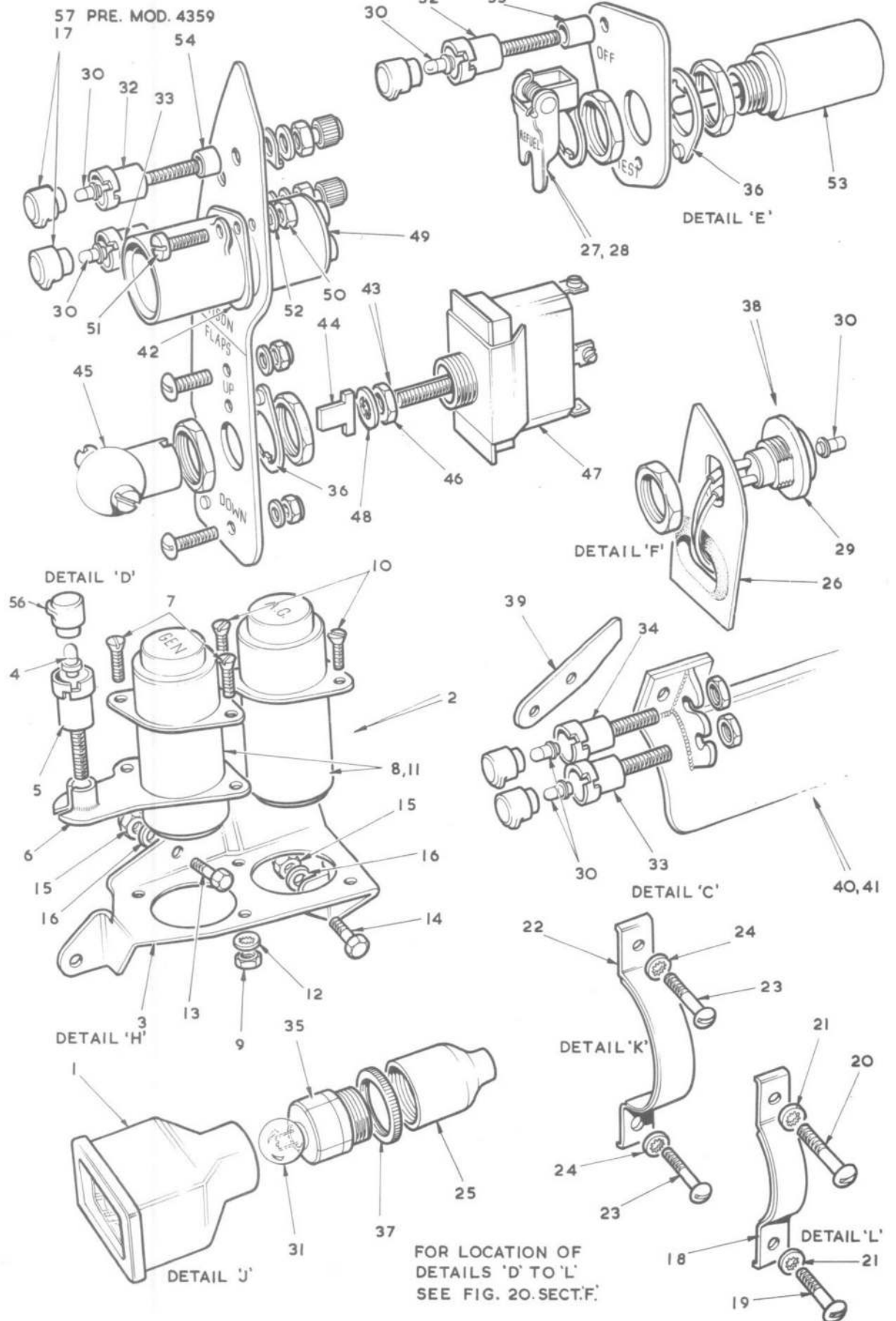
FIG. 21. PILOT'S INSTRUMENTS AND CONTROLS
