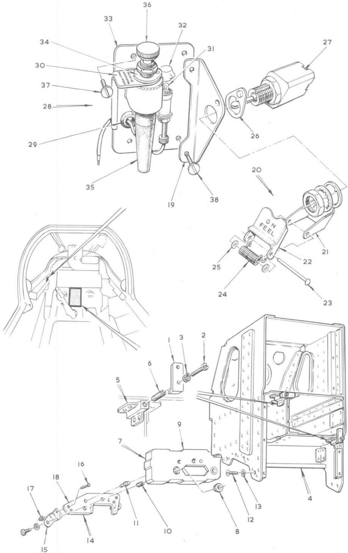
FIG. 22. PILOT'S INSTRUMENTS AND CONTROLS
