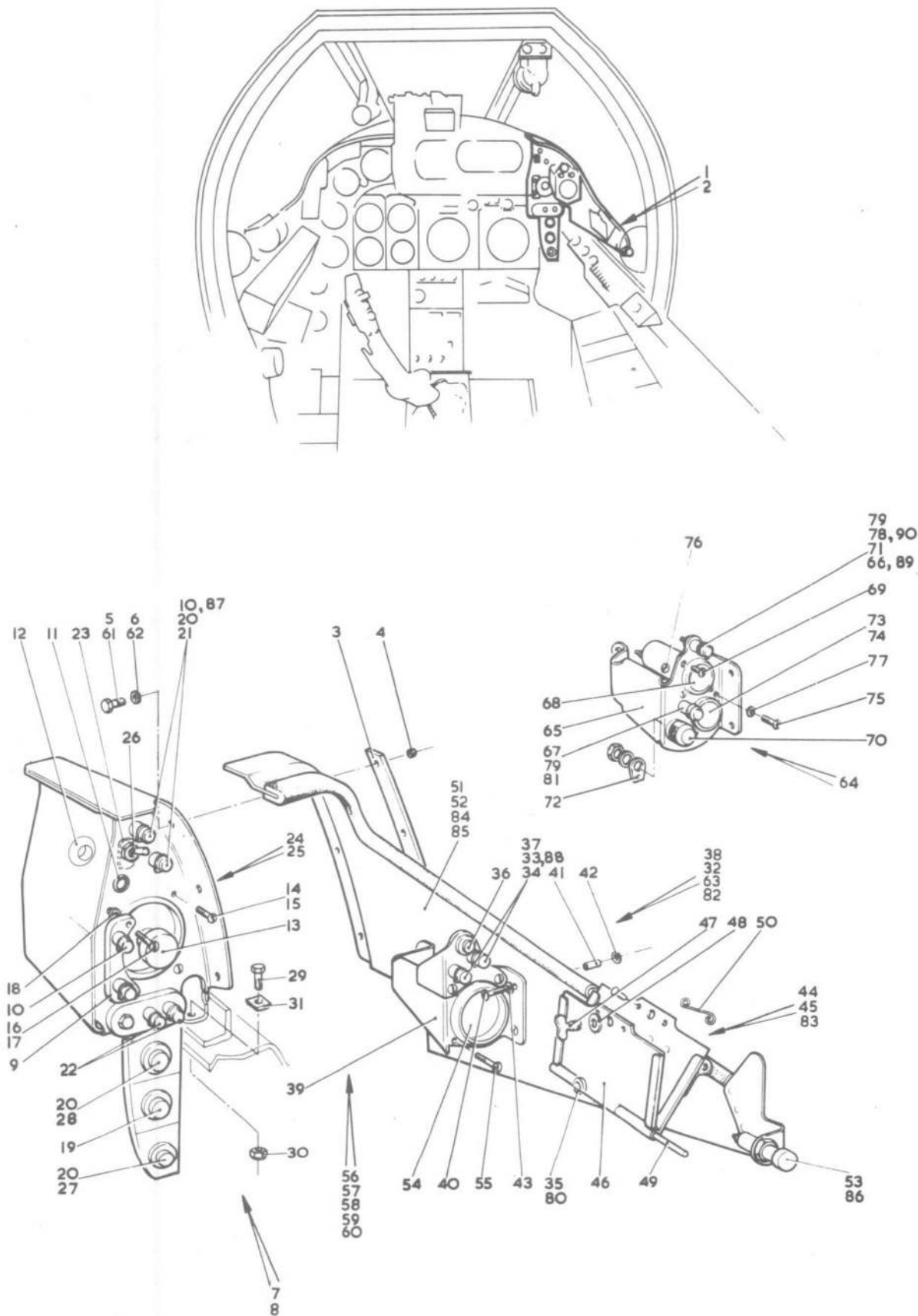
FIG. 15. INSTRUMENTS-PILOTS INSTRUMENTS AND CONTROLS
