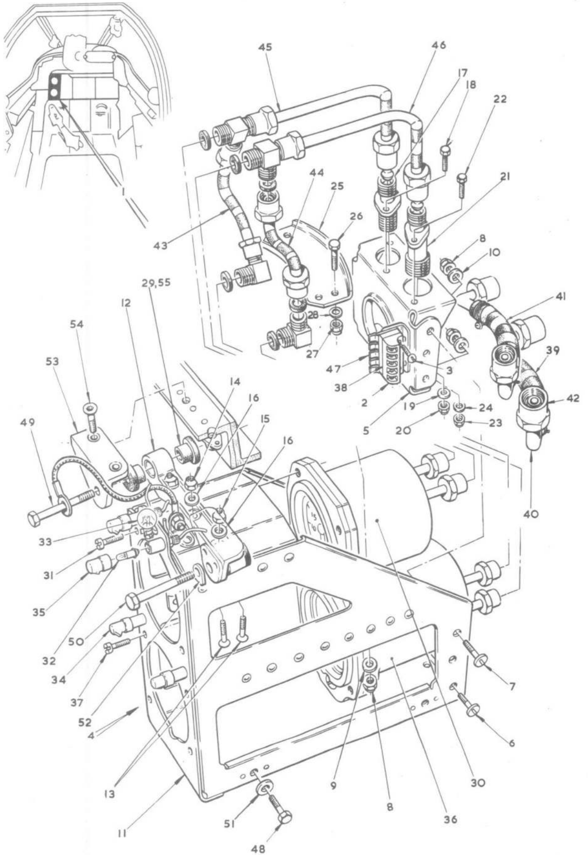
FIG.24. PILOT'S INSTRUMENTS AND CONTROLS
