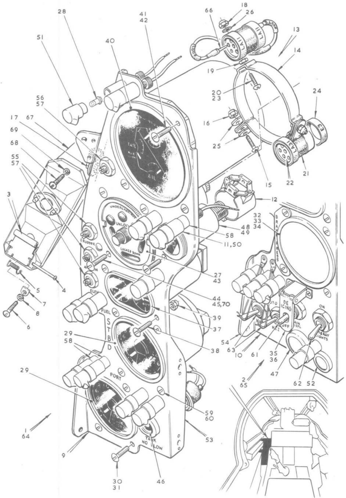
FIG.13. PILOT'S INSTRUMENTS AND CONTROLS
