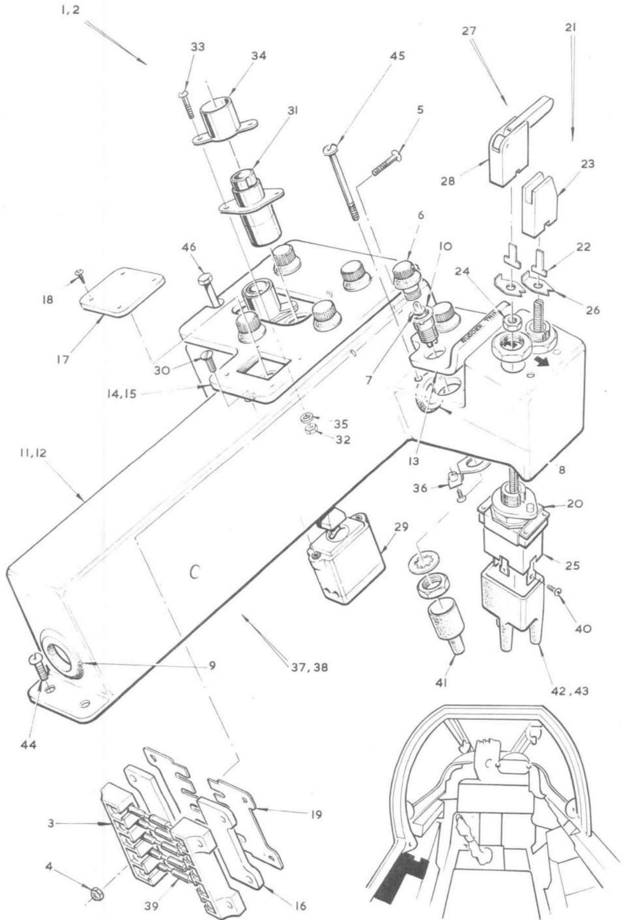
FIG.17. PILOT'S INSTRUMENTS AND CONTROLS
