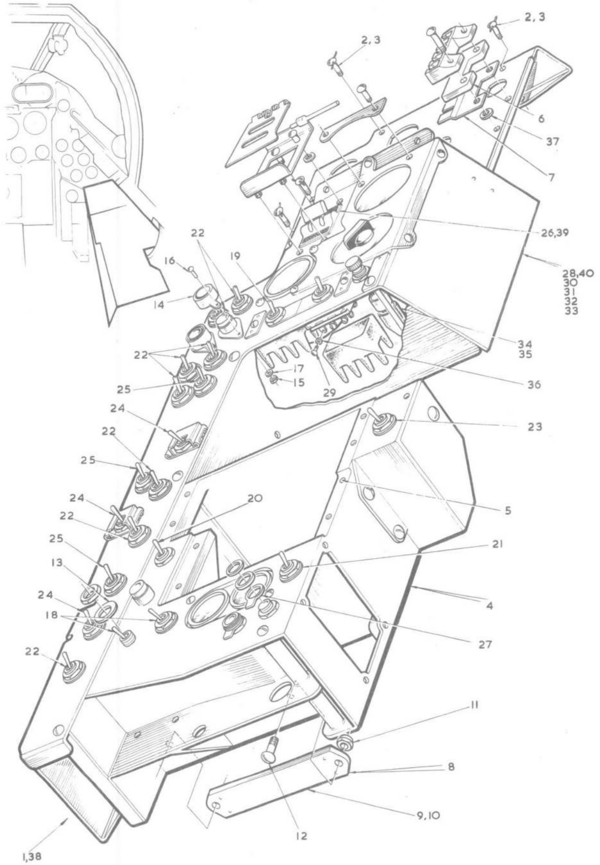
FIG. 5. PILOT'S INSTRUMENTS AND CONTROLS
