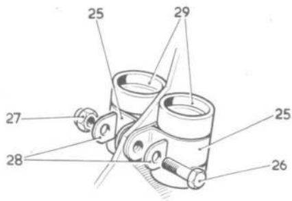
DETAIL AT A
