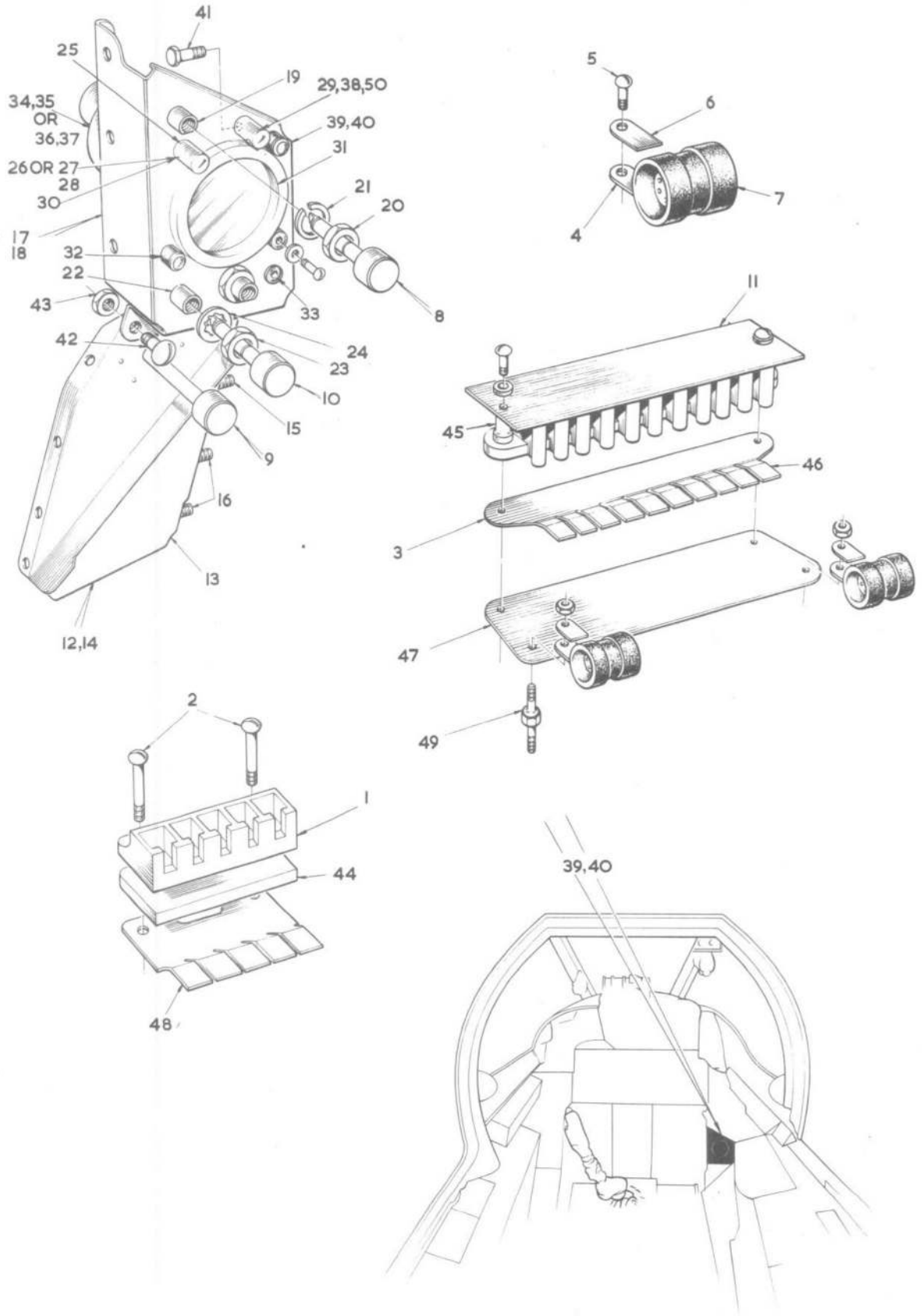
FIG. 8. PILOT'S INSTRUMENTS AND CONTROLS Restricted
