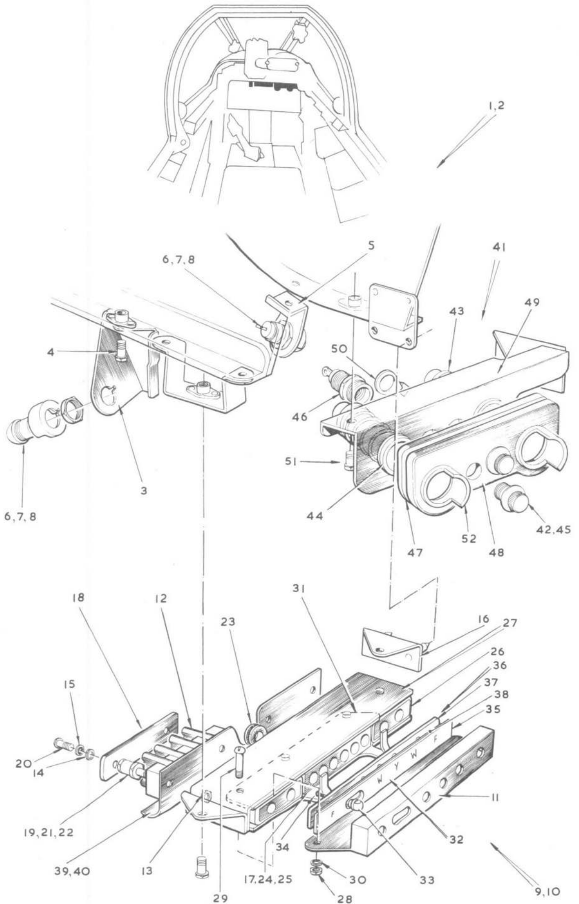
FIG.18. PILOT'S INSTRUMENTS AND CONTROLS Restricted
