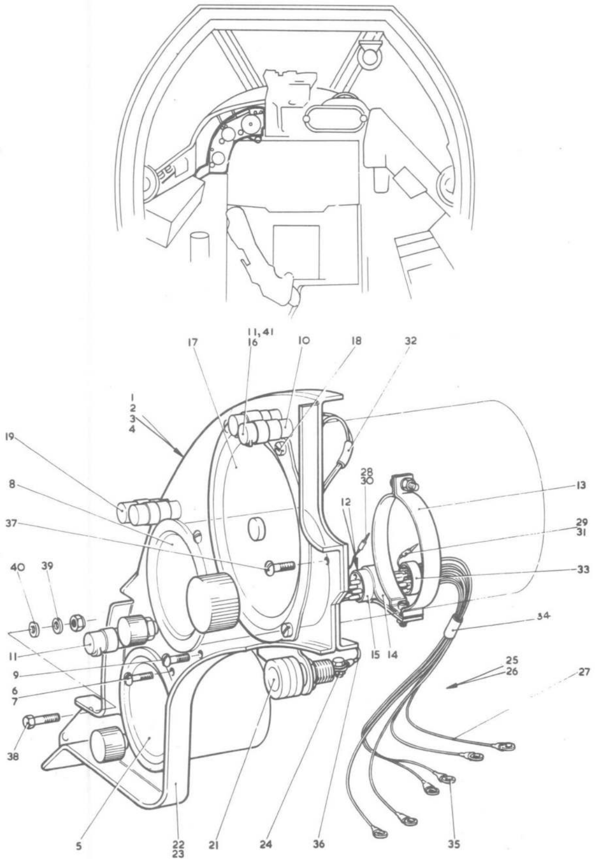
FIG.19 INSTRUMENTS-PILOTS INSTRUMENTS AND CONTROLS
