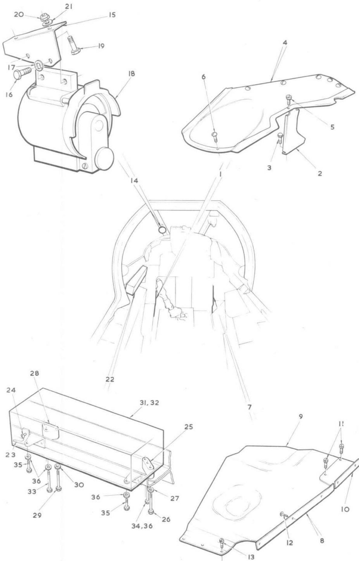
FIG.12. PILOT'S INSTRUMENTS AND CONTROLS Restricted
