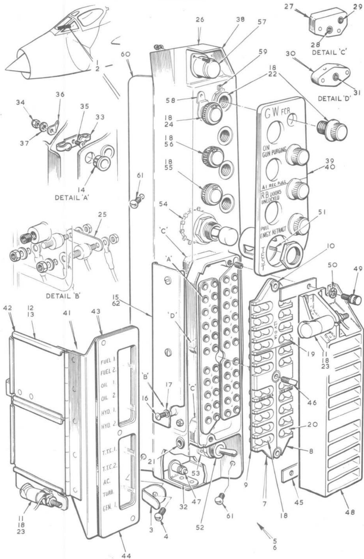
FIG.14. PILOT'S INSTRUMENTS AND CONTROLS
