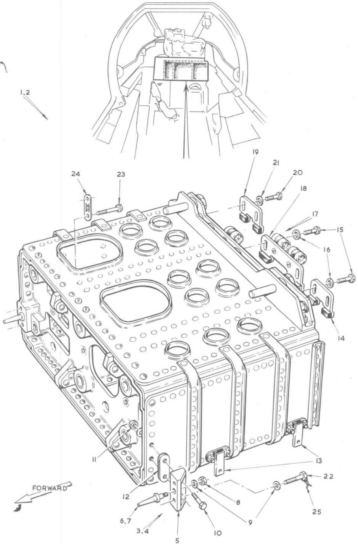
FIG. 25. PILOT'S INSTRUMENTS AND CONTROLS Restricted
