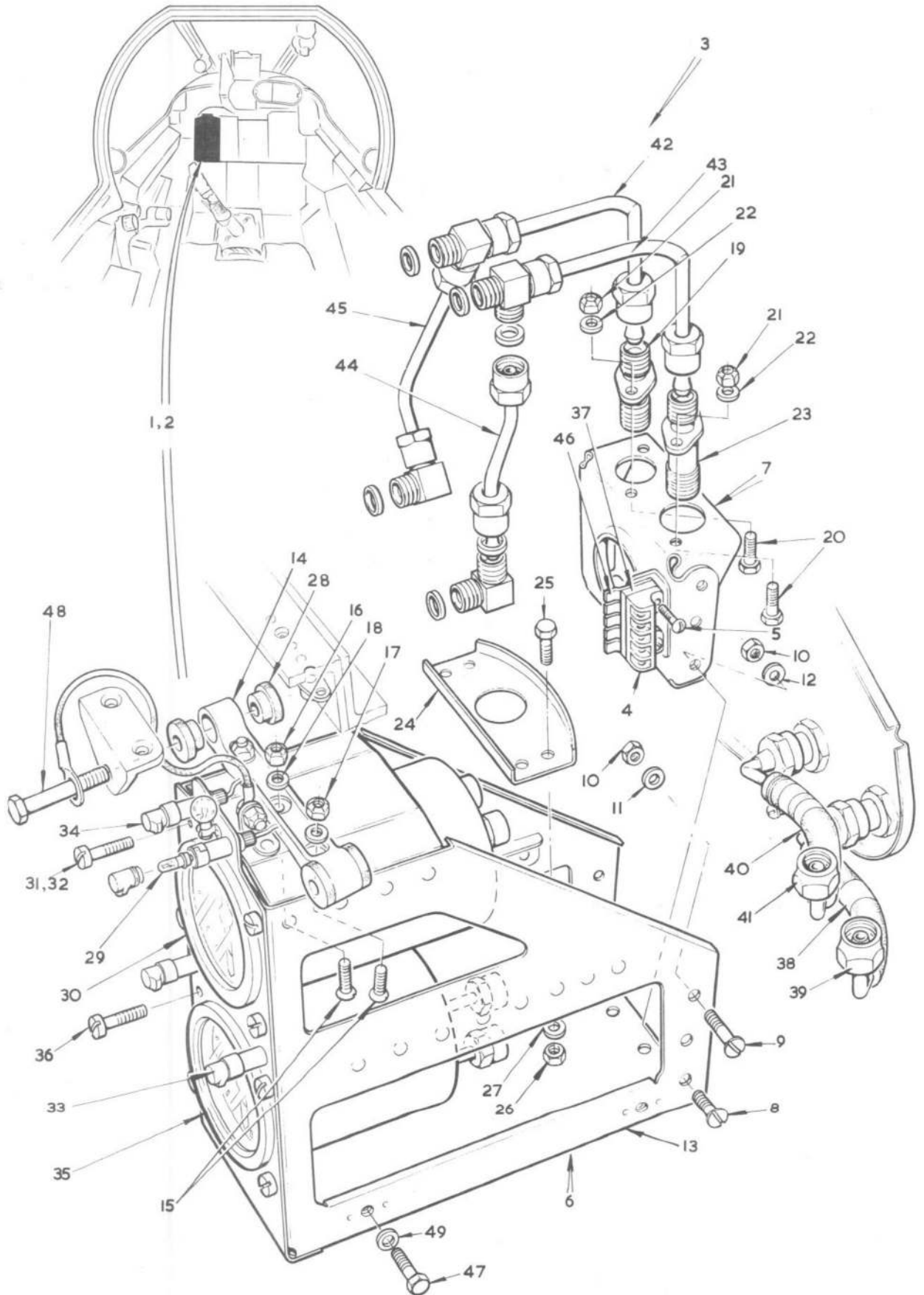
FIG. 23. PILOT'S INSTRUMENTS AND CONTROLS
