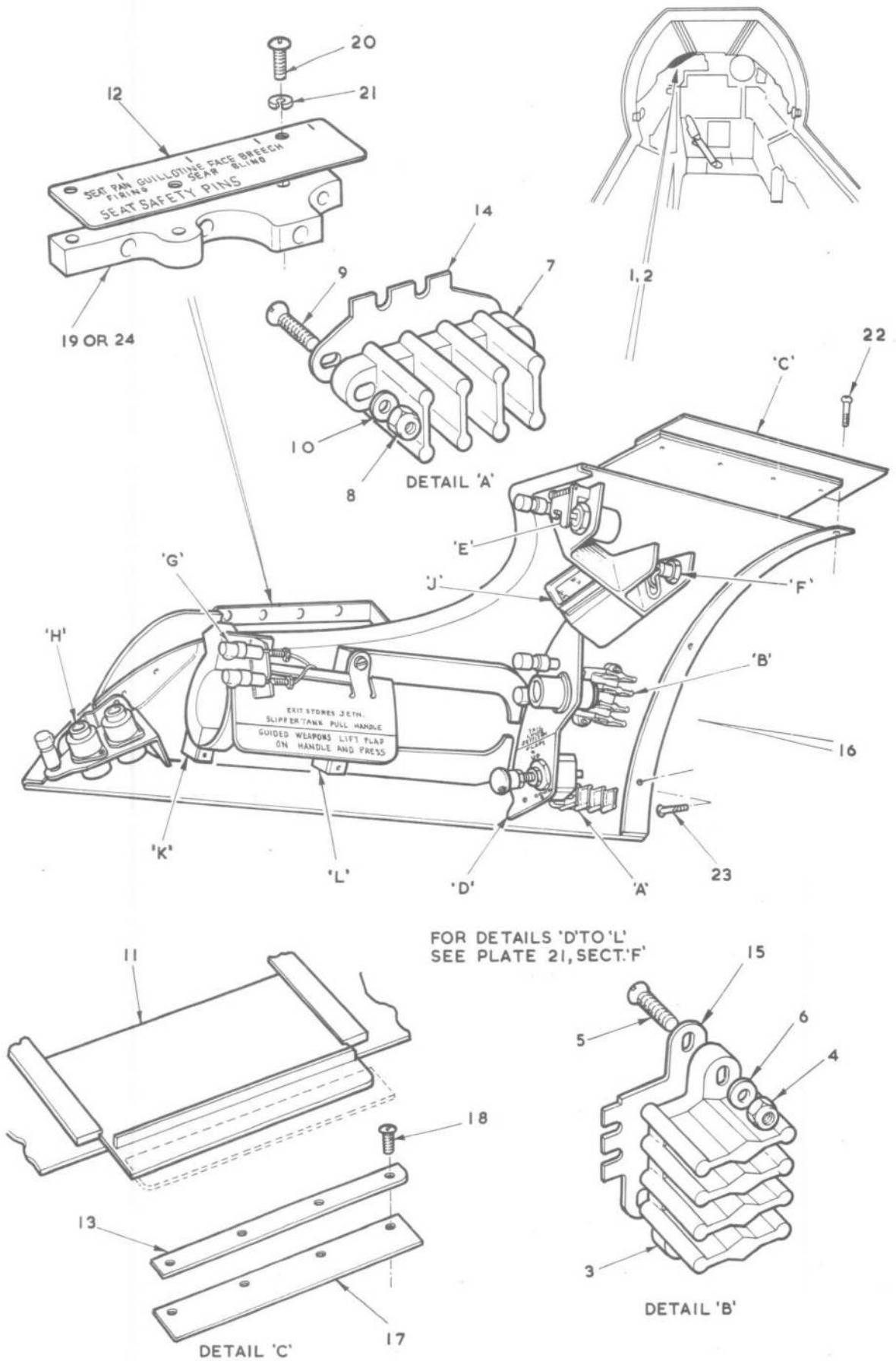
FIG.20. PILOT'S INSTRUMENTS AND CONTROLS
