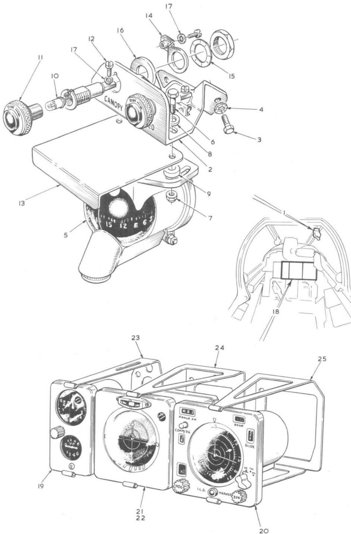
FIG. I. PILOT'S INSTRUMENTS AND CONTROLS Restricted
