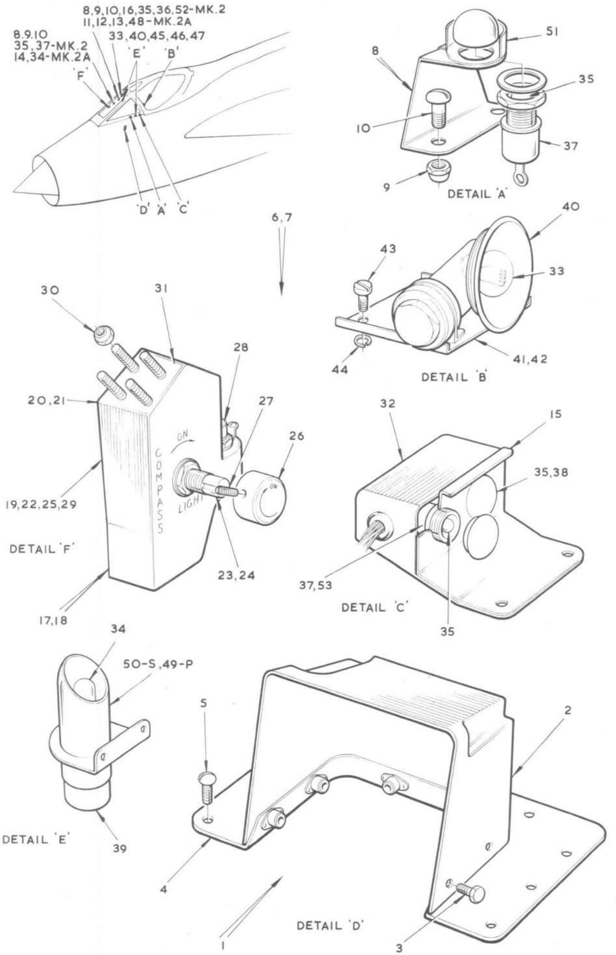
FIG.10. PILOT'S INSTRUMENTS AND CONTROLS Restricted
