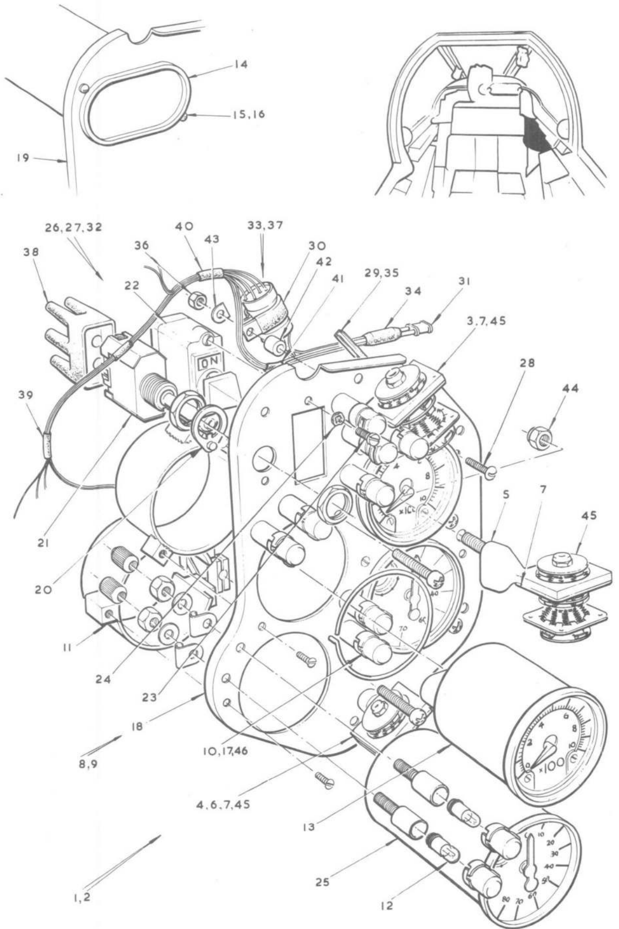
FIG.16. PILOT'S INSTRUMENTS AND CONTROLS Restricted
