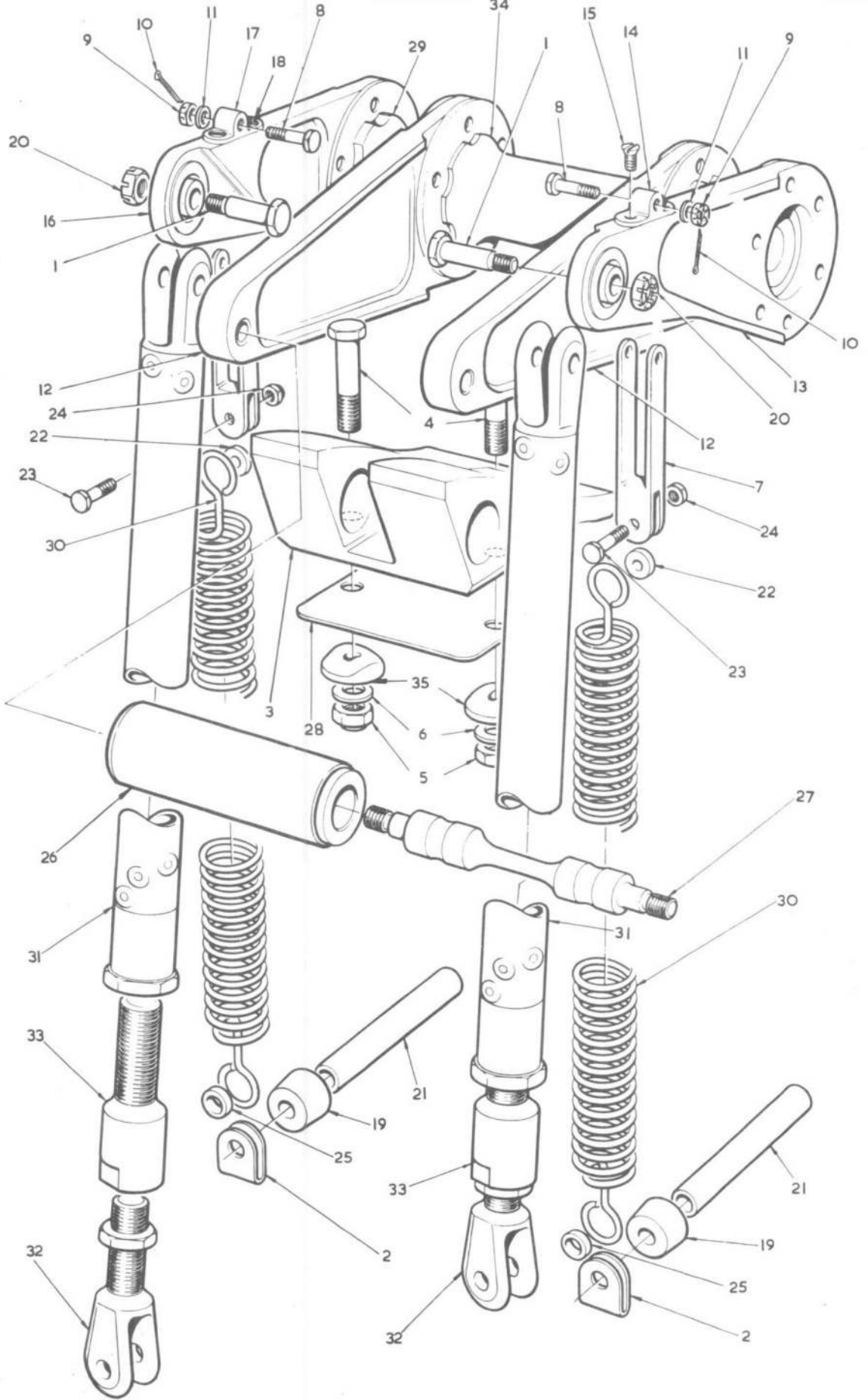
FIG.3 UNDERCARRIAGE, NOSE UNDERCARRIAGE Restricted
