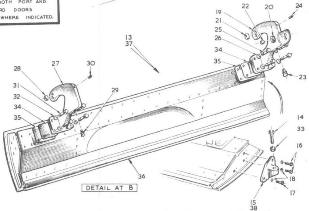
FIG. 4 UNDERCARRIAGE, NOSE UNDERCARRIAGE DOORS Restricted
