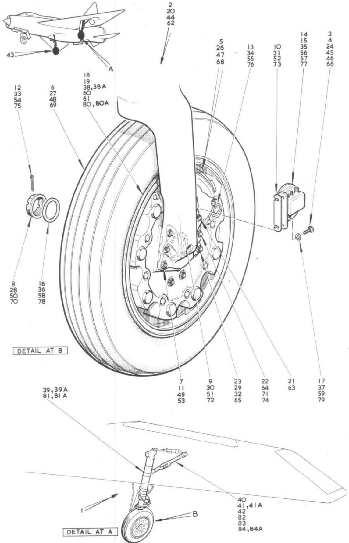
FIG. I MAIN UNDERCARRIAGE, PORT AND STARBOARD Restricted
