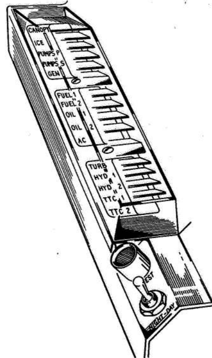
1—9 Fig 4 — Auxiliary Warning Panel — F Mk 3 and F Mk 6
