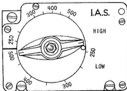
AIRSPEED SETTING CONTROL AND SCALES
