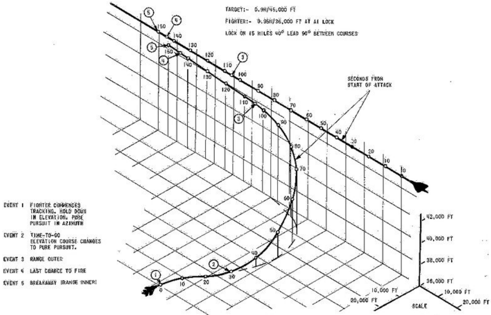
1-8-1 Fig 1 Firestreak Attack — Subsonic Target
