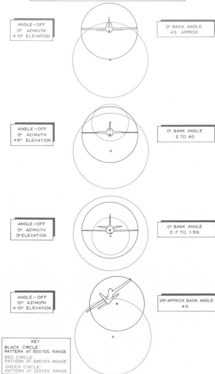
1-8-3 Fig. 3 Typical Bullet Patterns (1)
