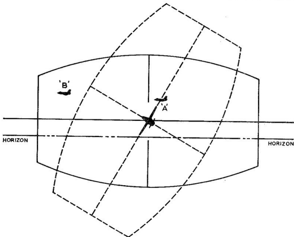
2-1-1 Fig 3 Look Angle Boundaries in Track Phase
