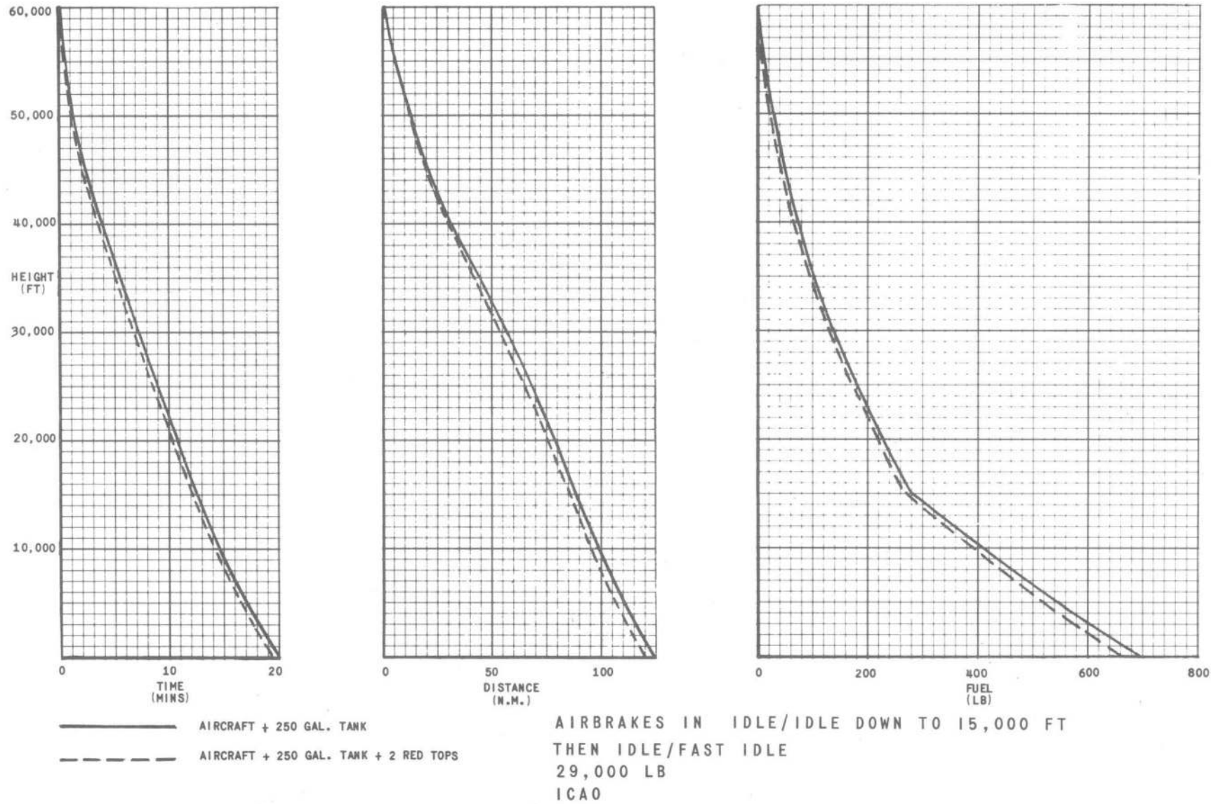
FIG. 6-2. RANGE DESCENT AT 0.9M/250KT.
