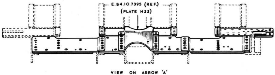
VIEW ON ARROW 'A'
