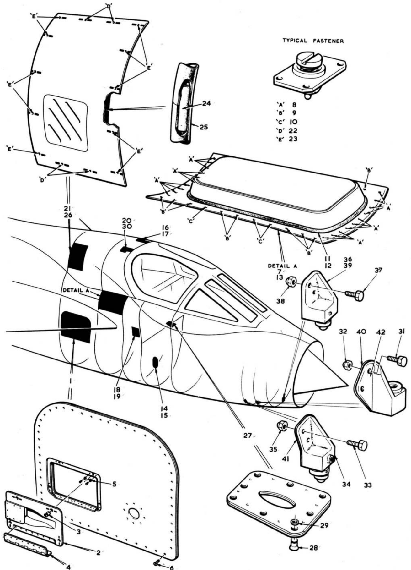
FIG.17 FUSELAGE - FRONT FUSELAGE STRUCTURE
