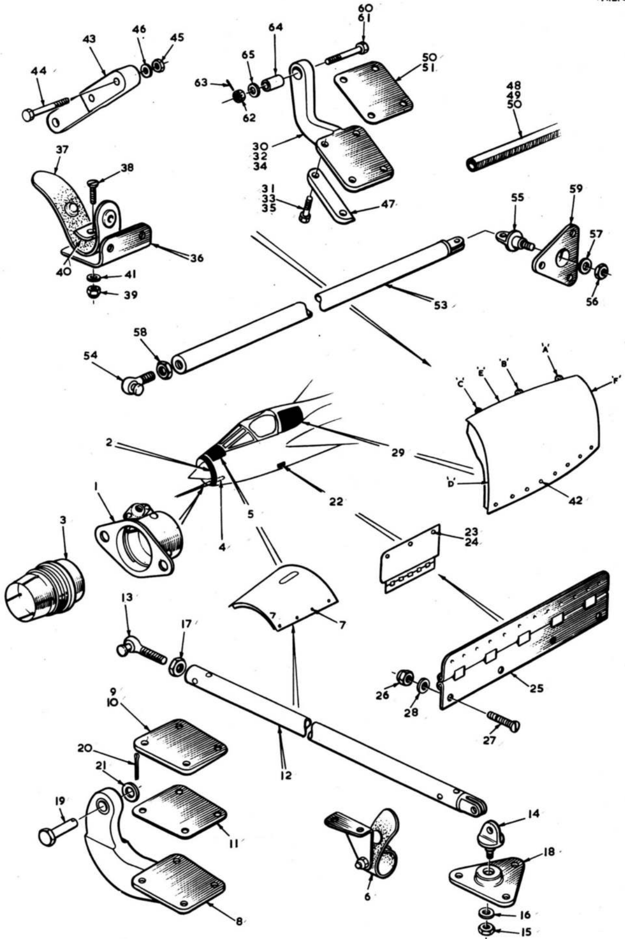
FIG.14 FUSELAGE - FRONT FUSELAGE STRUCTURE
