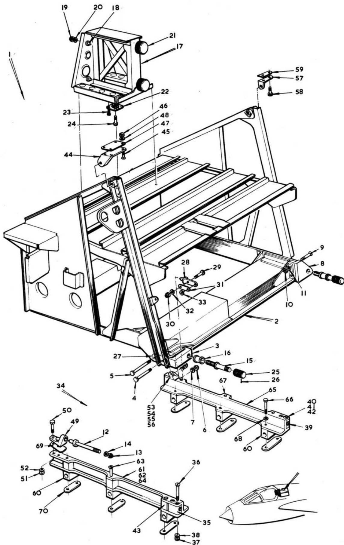
FIG.12 FUSELAGE - FRONT FUSELAGE
