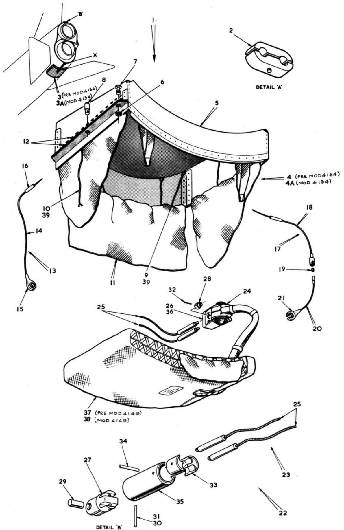
FIG.9 FUSELAGE-BRAKING PARACHUTE INSTALLATION
