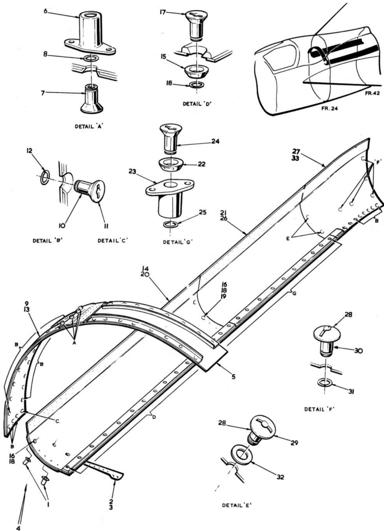
FIG.10 FUSELAGE - DUCT PANELS, ASSEMBLY TO AIRCRAFT
