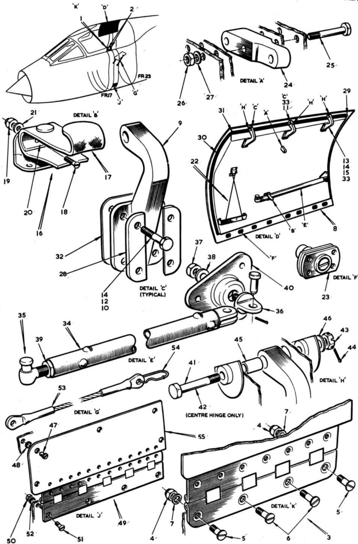
FIG.15 FUSELAGE-FRONT FUSELAGE STRUCTURE
