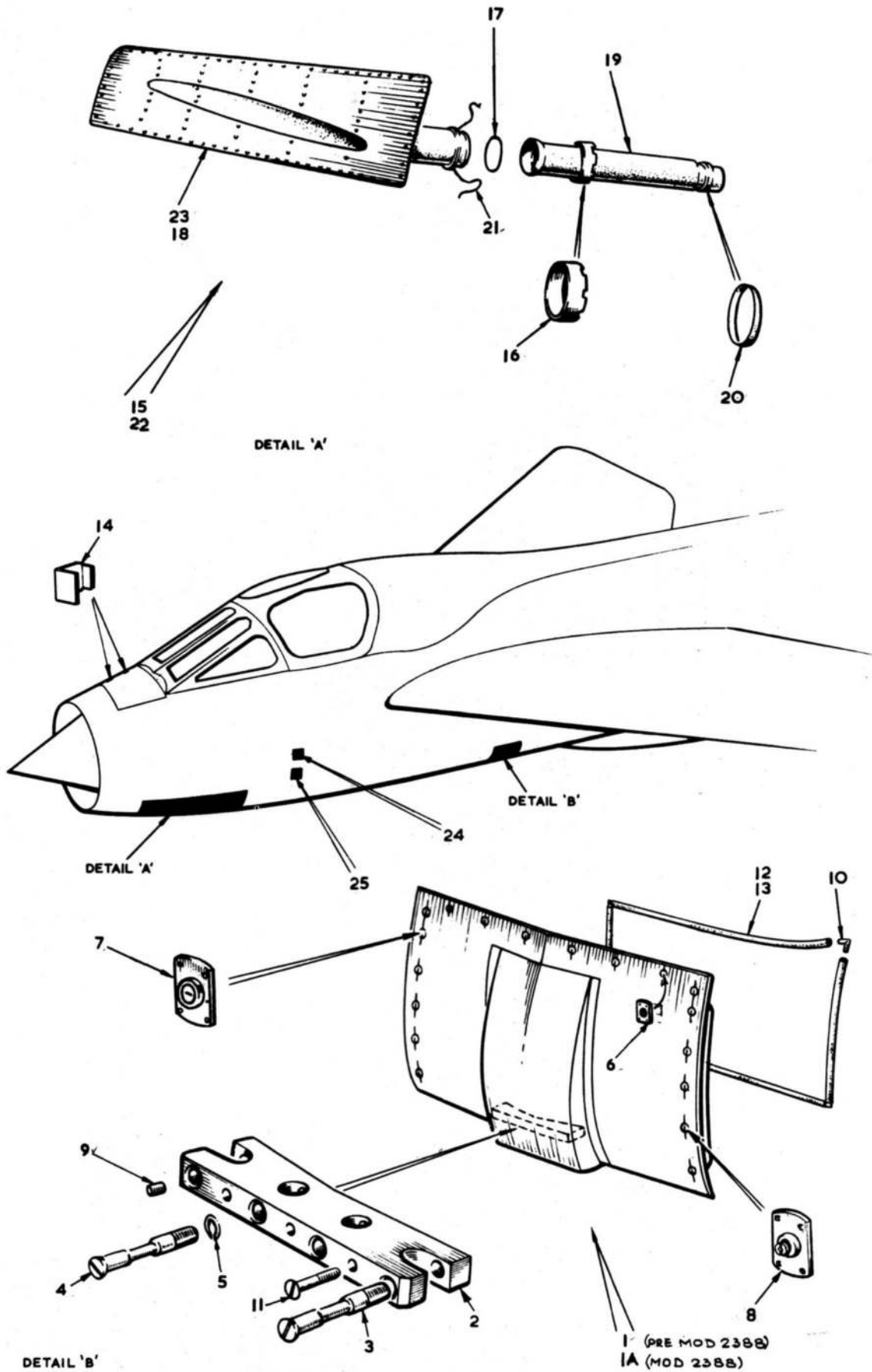
FIG.18A FUSELAGE - FRONT FUSELAGE STRUCTURE
