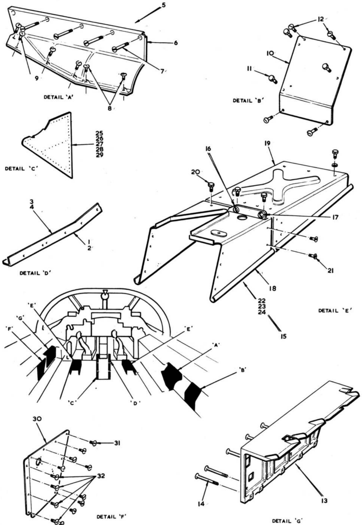
FIG.19 FUSELAGE - FRONT FUSELAGE STRUCTURE
