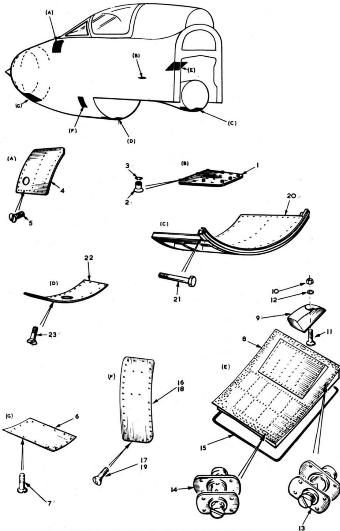
FIG. 8 FUSELAGE-FRONT FUSELAGE STRUCTURE
