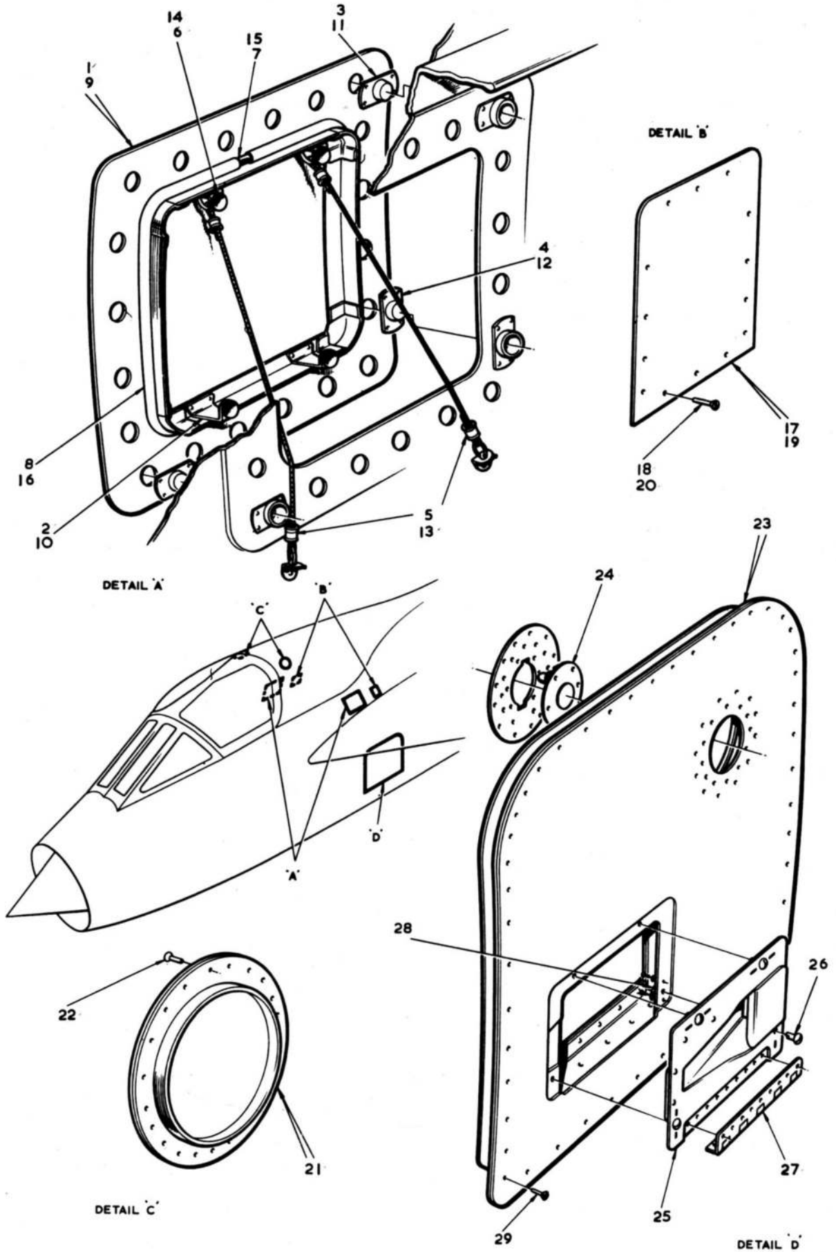
FIG.16 FUSELAGE - FRONT FUSELAGE STRUCTURE
