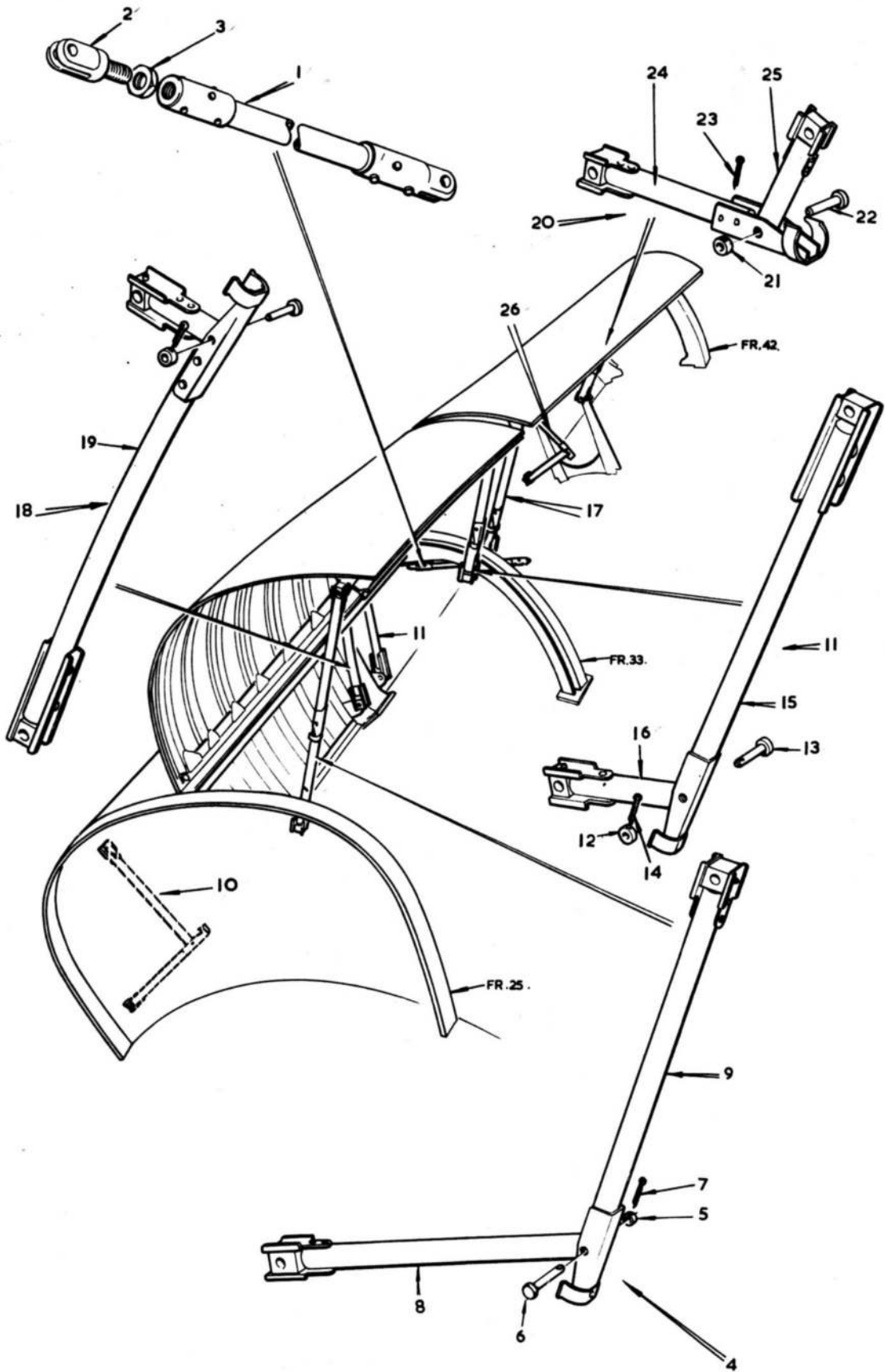
FIG.5 FUSELAGE - ASSEMBLY OF SPINE TO FUSELAGE
