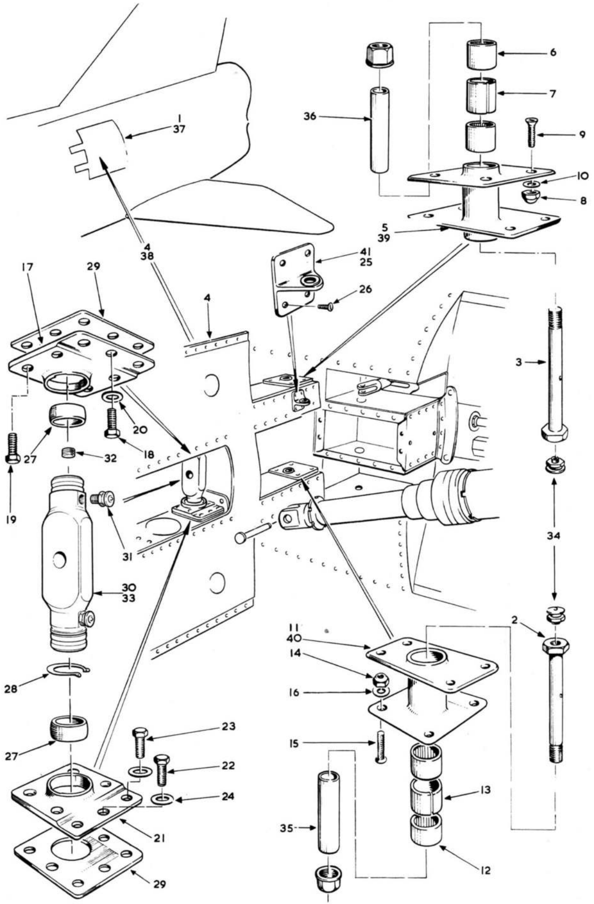
FIG.2 FUSELAGE-ASSEMBLY OF AIR BRAKE TO FUSELAGE,P&S
