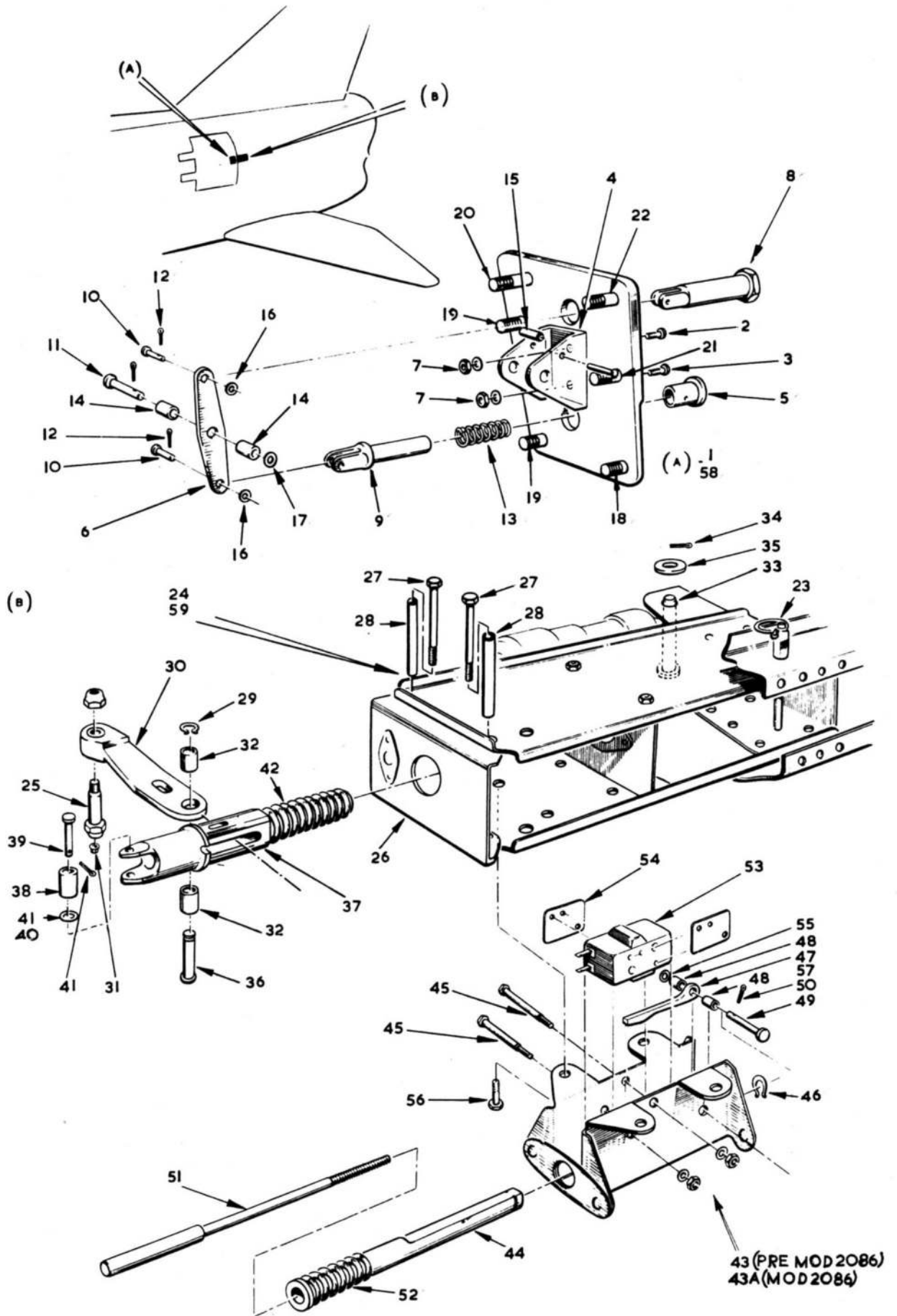
FIG.3 FUSELAGE-ASSEMBLY OF AIR BRAKE TO FUSELAGE, P & S
