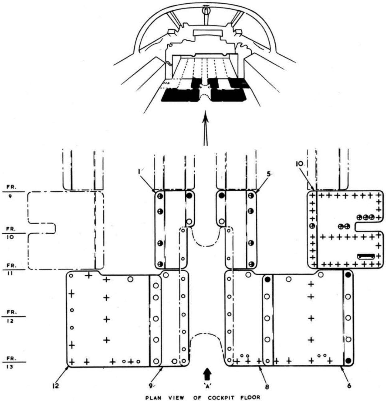
PLAN VIEW OF COCKPIT FLOOR
