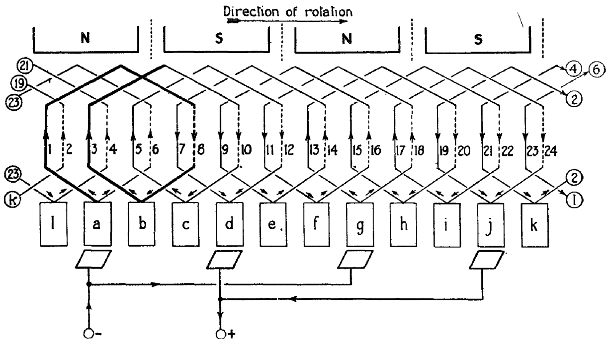
FIG. 16, CHAP. IV.—Principle of lap winding.
