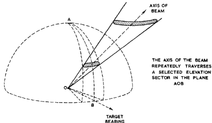
Fig.L: Fan beam system for elevation sector scanning.
