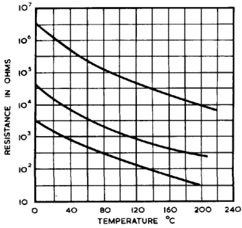
(a) Resistance/Temperature characteristic of three thermistors.
