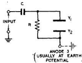
Fig. 294 - Input circuit to deflector plates.
