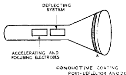
Fig. 287 - Extra electrode assembly for post-deflector acceleration.
