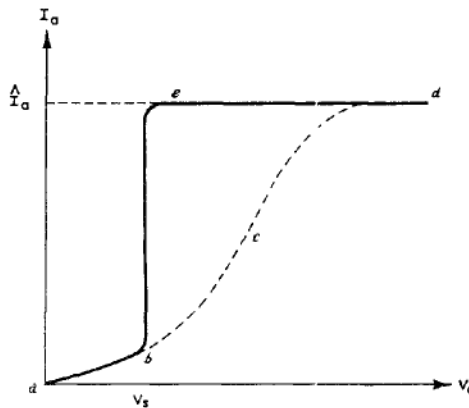
Fig. 302 - Effect of gas on diode characteristic.
