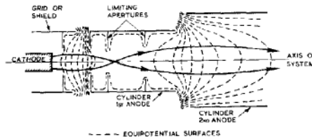
Fig. 269 - Two-anode focusing system of CRT.
