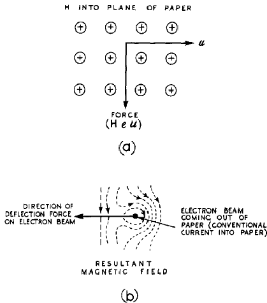
Fig. 272 - Force acting on an electron moving in a magnetic field.
