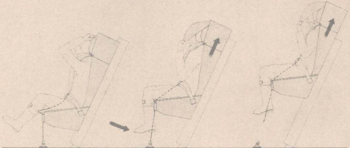
FIG.1. LEG RESTRAINT CORDS (MK.2 AND 3 SERIES SEATS) - FUNCTIONING
