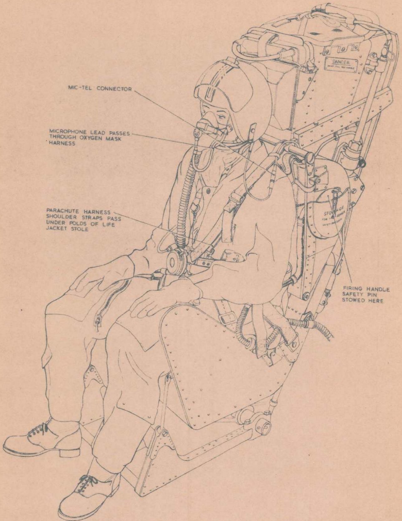
Fig. 5. The seat occupied (2)
