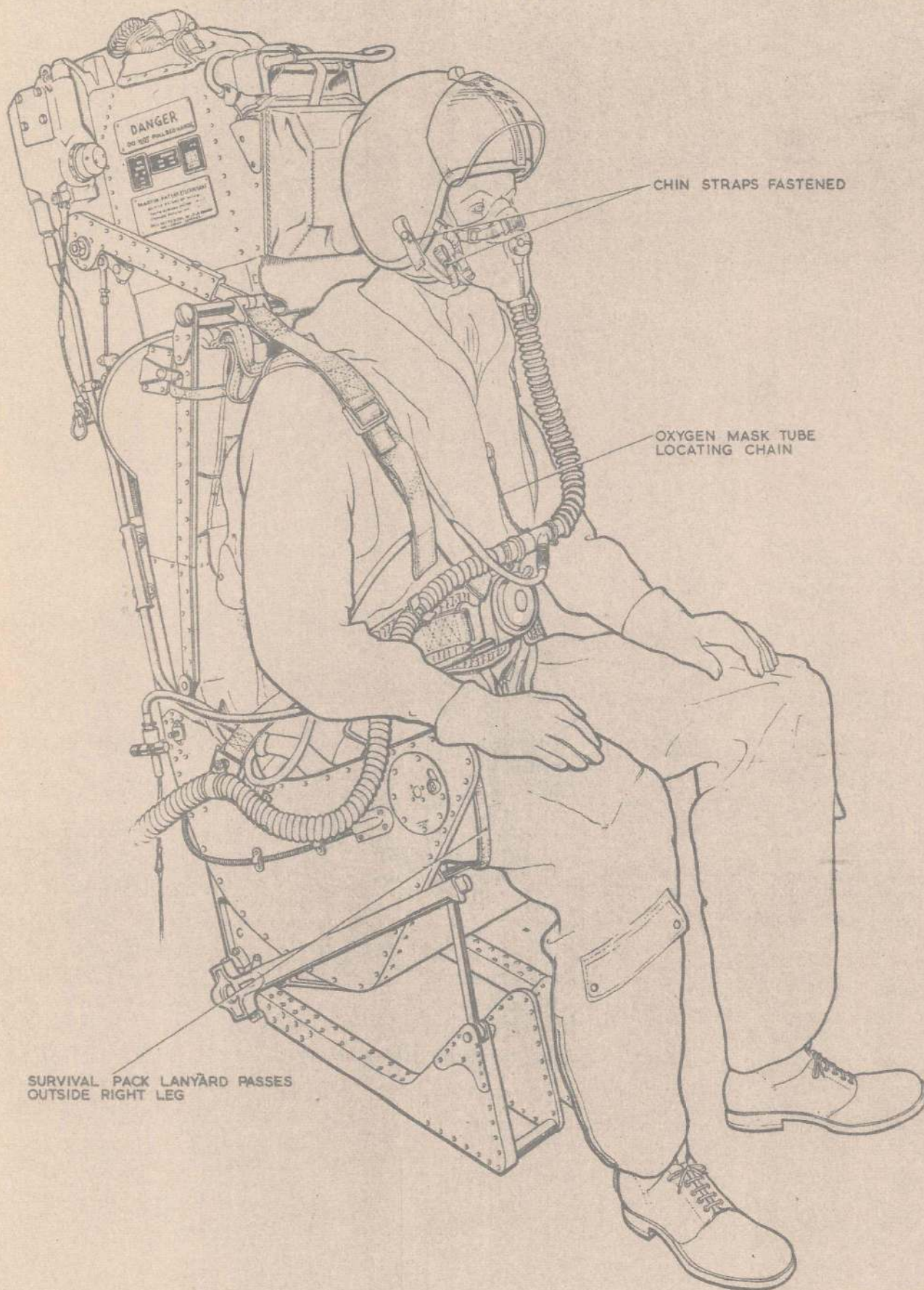
Fig. 4. The seat occupied (I)
