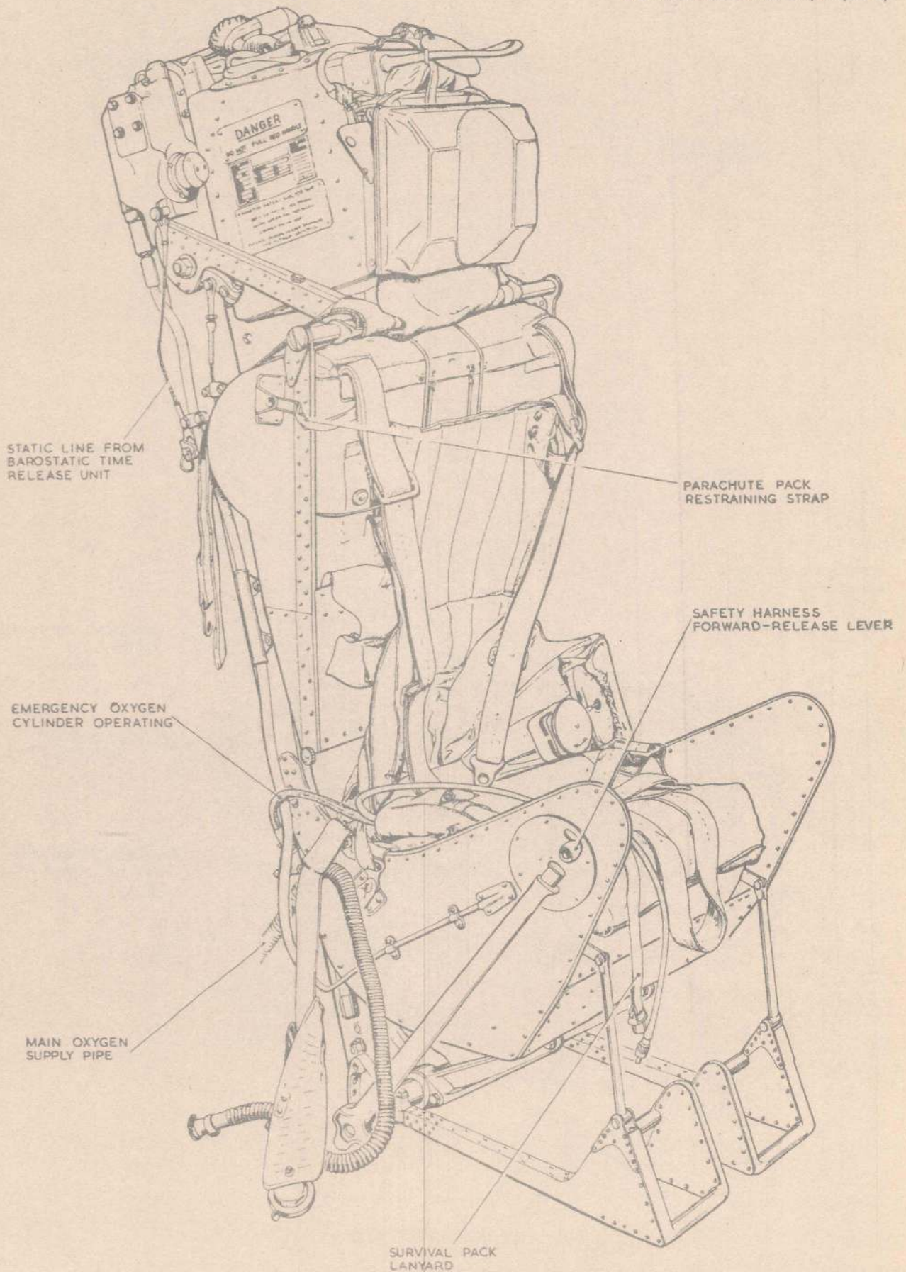
Fig. 1. The seat equipped (1) RESTRICTED
