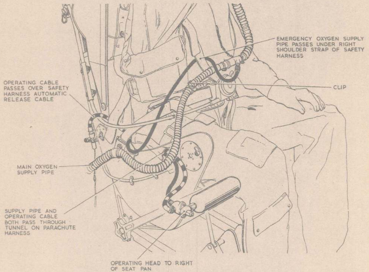
Fig. 3. Arrangement of oxygen pipes on the seat
