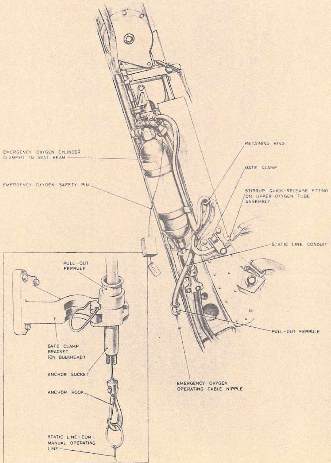
Fig. 1. Arrangement of emergency oxygen supply (inset: Anchor socket on bulkhead)
