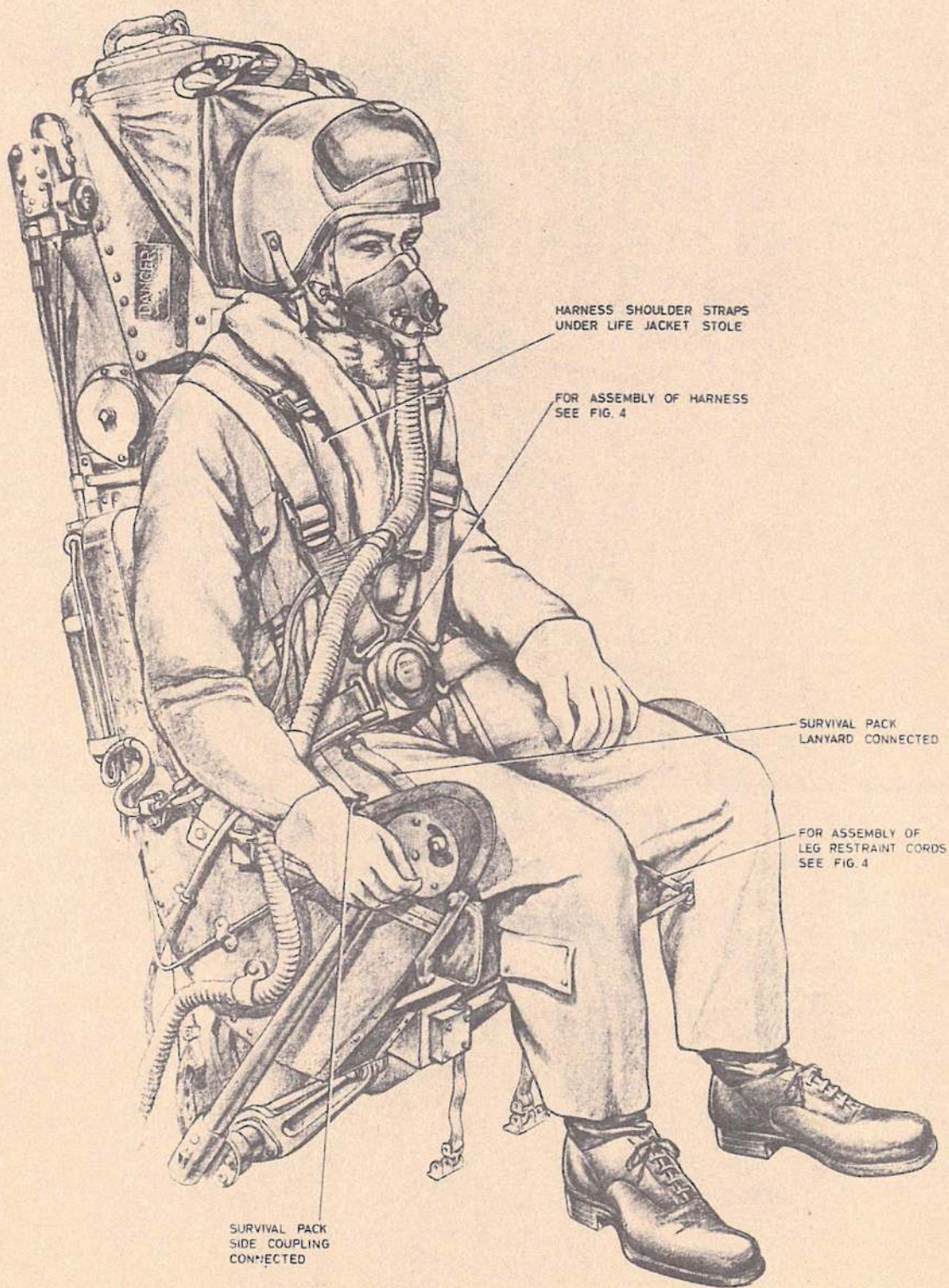
Fig. 5. The ejection seat Type 2CB occupied (1)
