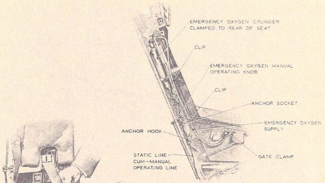
Fig. 3. Arrangement of emergency oxygen supply
