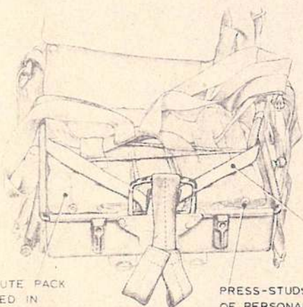
Fig. 7. Installing parachute assembly (Stage 4)
