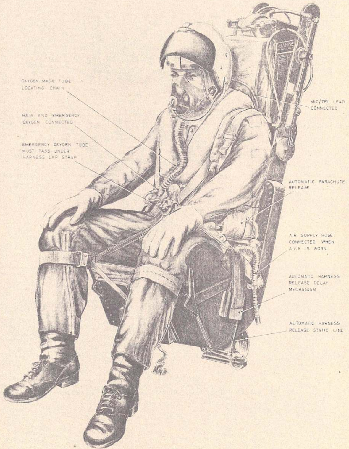
Fig. 13. The Mk. 1CN seat occupied (2)
