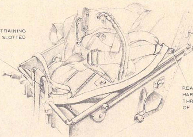
Fig. 6. Installing parachute assembly (Stage 3)
