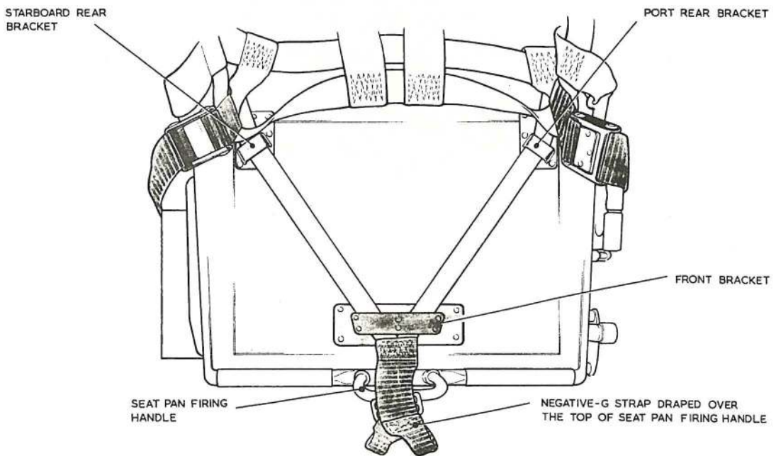
Fig. 5. Fitting negative-G strap
