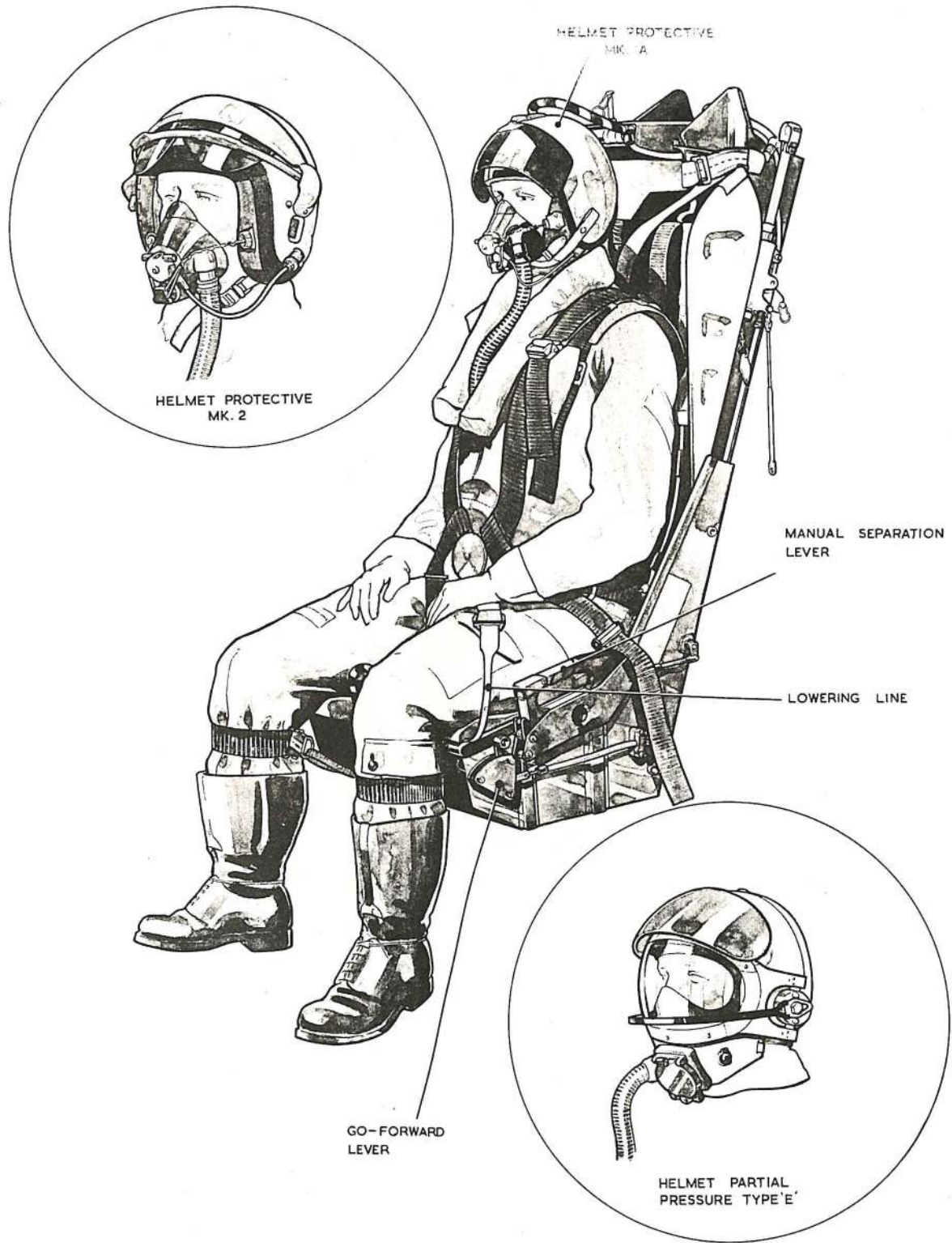
Fig. 10. The seat occupied (port)
