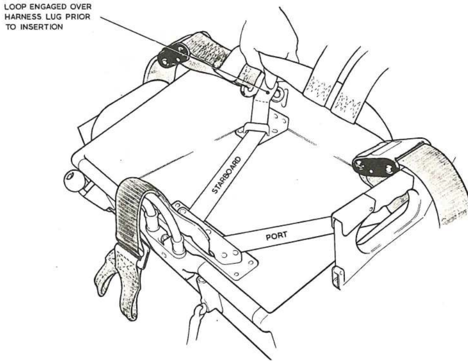
Fig. 5. Fitting negative-G strap
