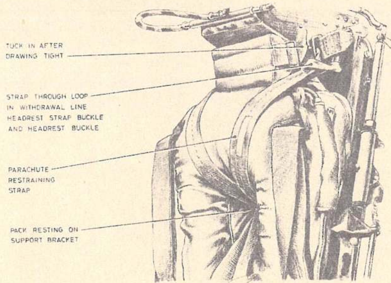
Fig. 3. Ejection seat: Installing the parachute assembly: Stage 2
