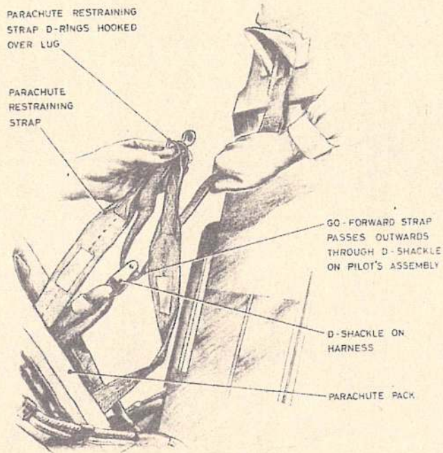
Fig. 2. Ejection seat: Installing the parachute assembly: Stage 1
