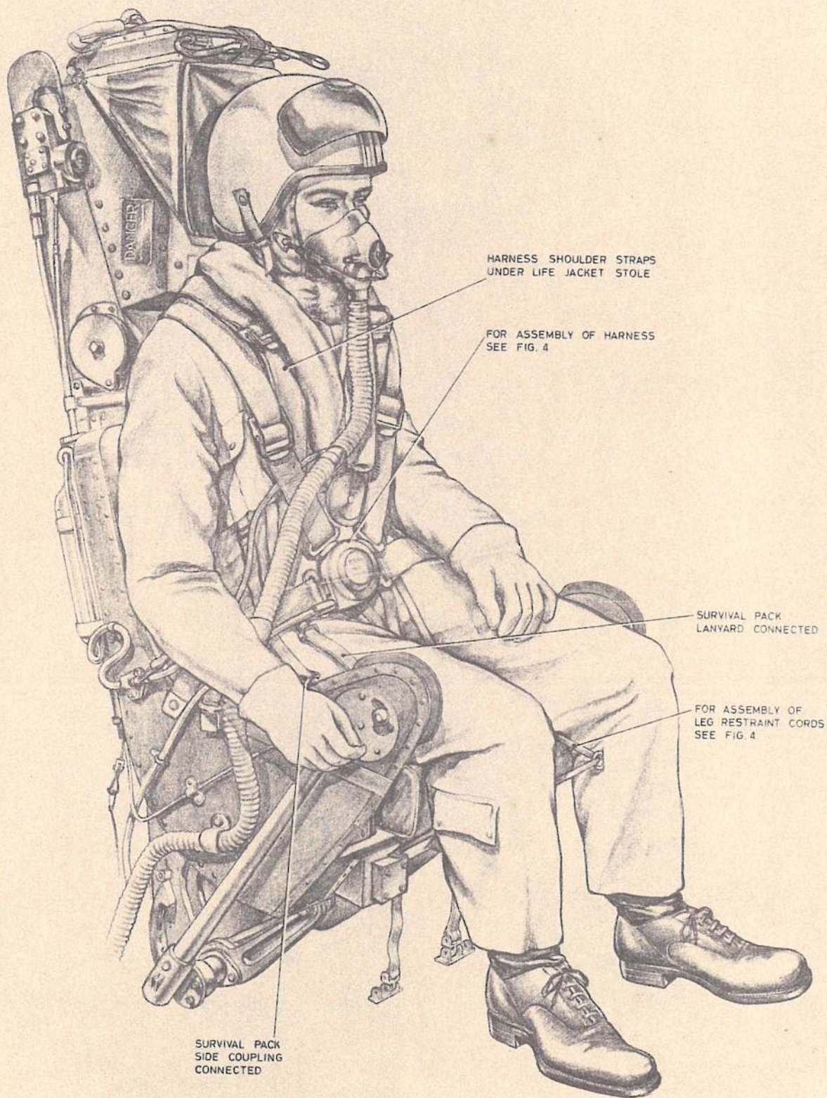
Fig. 5. The ejection seat Type 2CA occupied (1)
