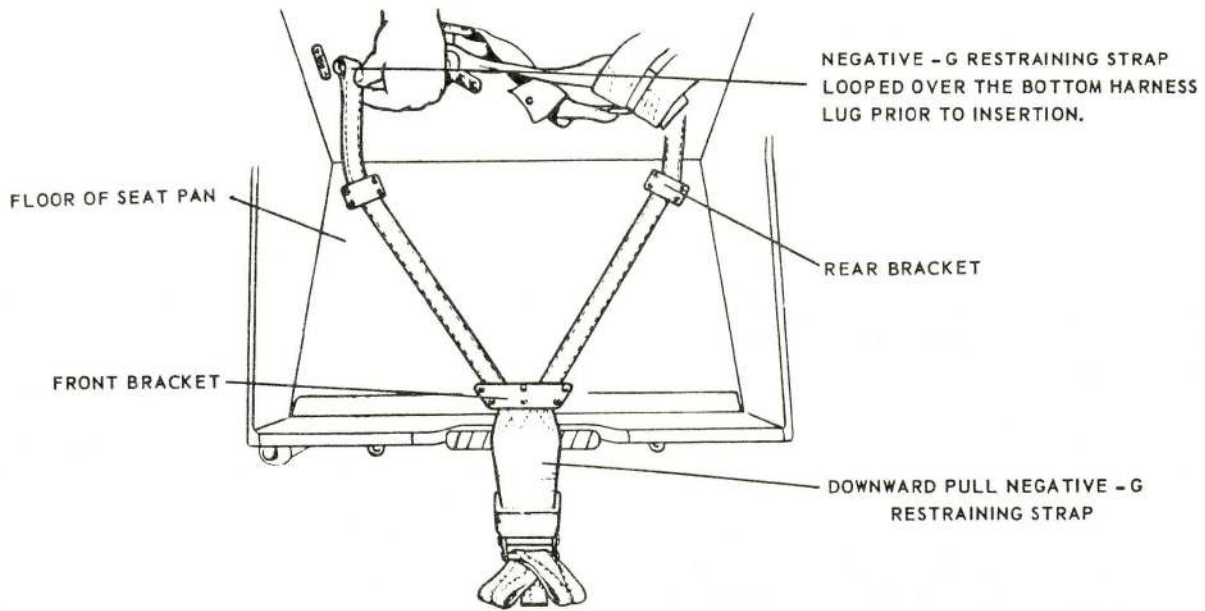
Fig. 1 Arrangement of downward pull negative-G restraining strap in seat pan
