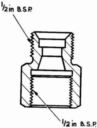
Fig. 1. Adapter, \frac{1}{2} in. B.S.P. (803088), Ref. No. 6C/2582
