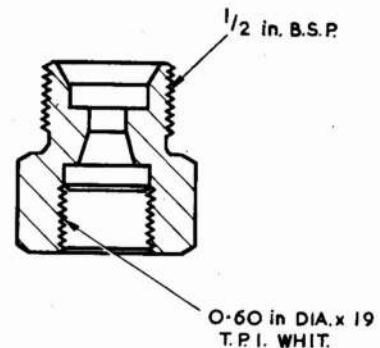
Fig. 1. Adapter, 0.60 in. \times 19 T.P.I., (803087) Ref. No.6C/2581
