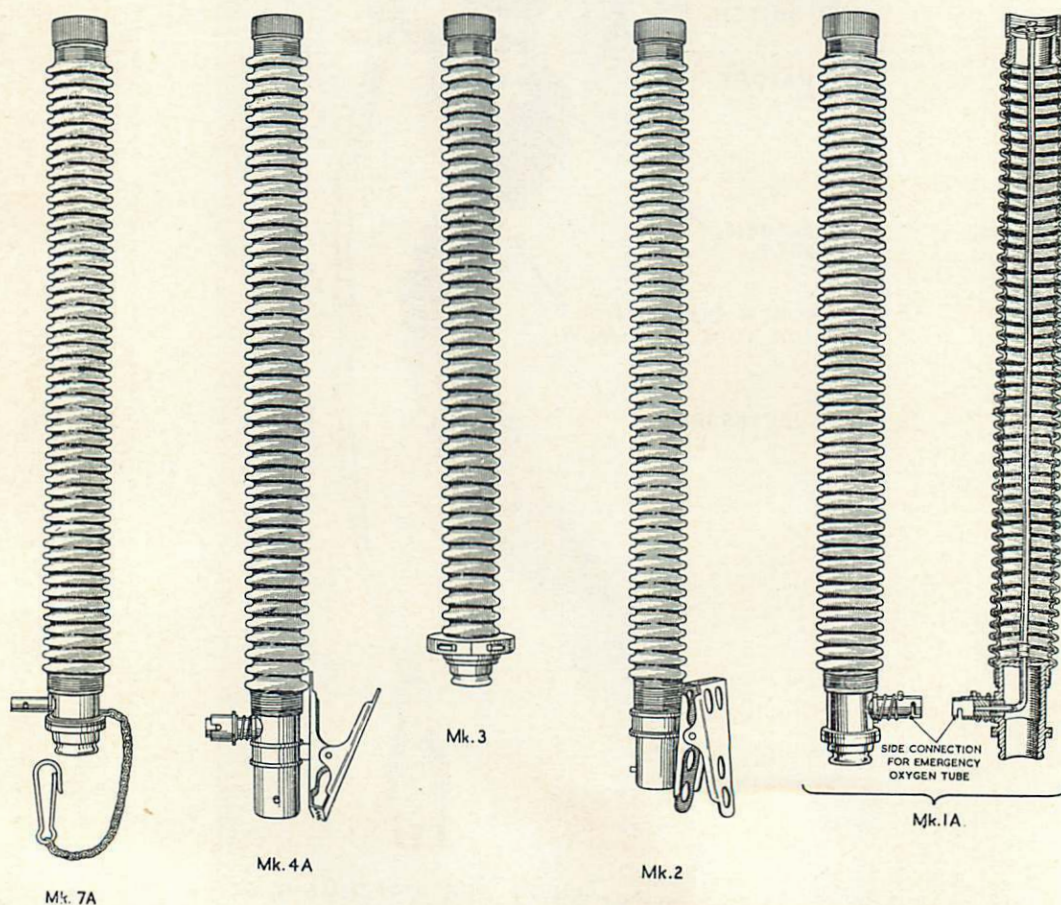
Fig. 2. Mask Tube Assemblies.
