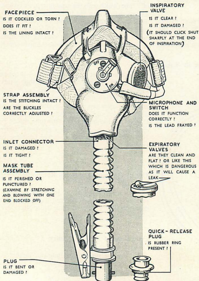
Fig. 7. Points to be Observed when Servicing the Mask.
