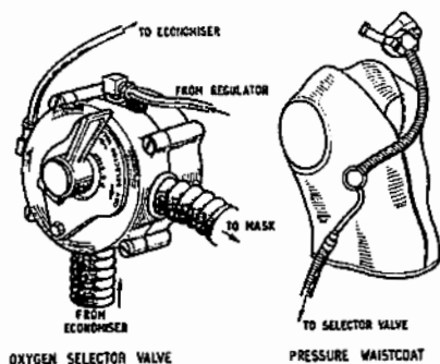
Fig. 5. Typical Pressure-Breathing System.
