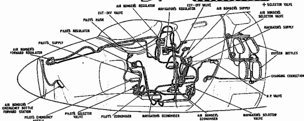
Fig. 5. Typical Pressure-Breathing System.
