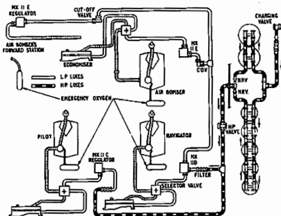
Fig. 5. Typical Pressure-Breathing System.
