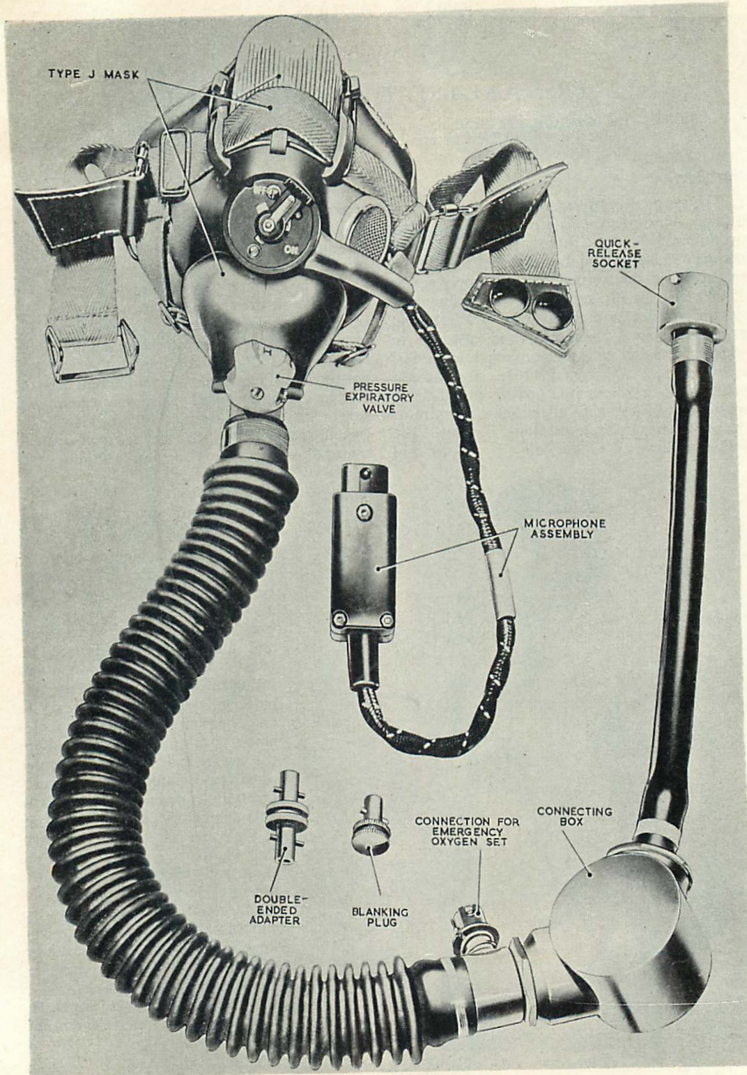
Fig. 2. Oxygen Mask, Type J.
