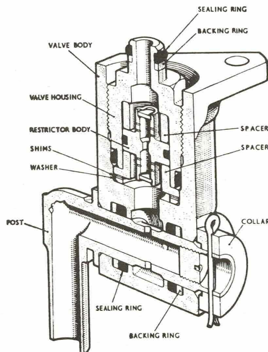
Fig. 2 Detail showing restrictor valve
