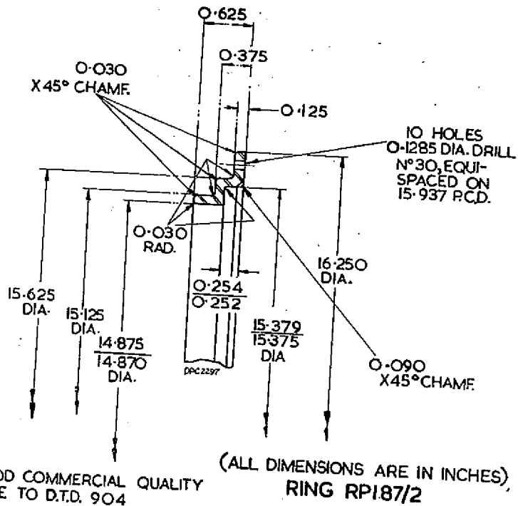
Fig. 2. Dimensions of ring
