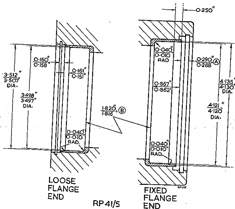
Fig. 2. Dimension for machining fitted liners
