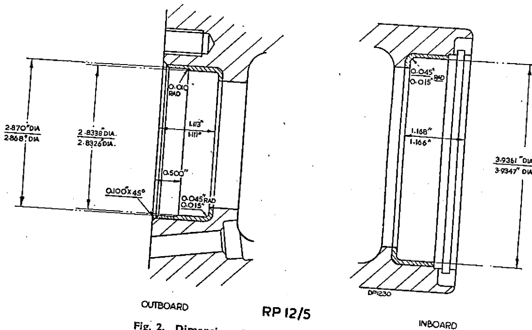
Fig. 2. Dimensions for machining fitted liners
