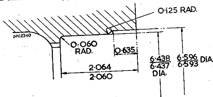
Fig. 1. Machining of bearing housing
