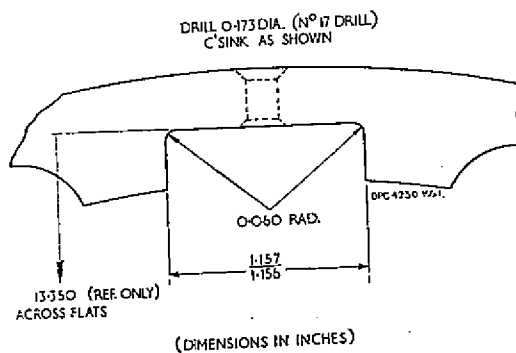
Fig. 1. Drilling and machining the tenons
