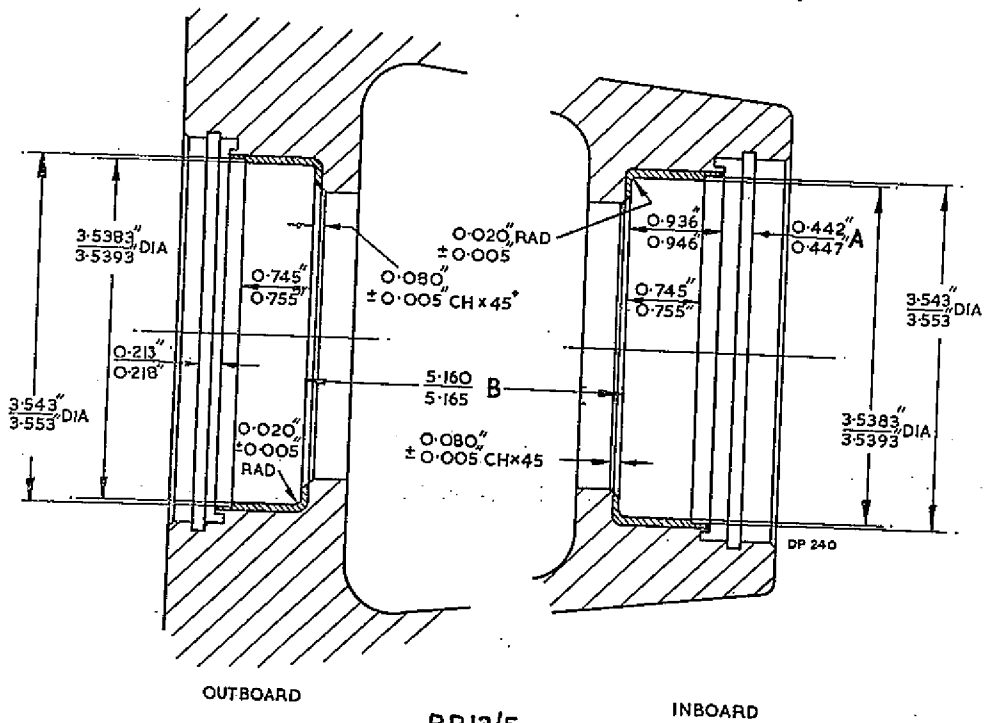
Fig. 2. Dimensions for machining fitted liners
