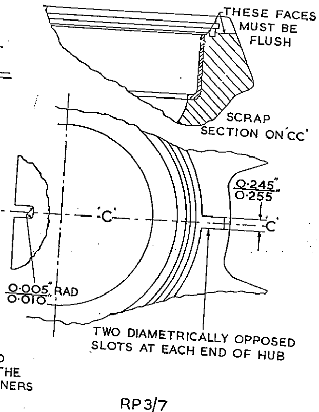
Fig. 4. Dimensions for milling slots in hub
