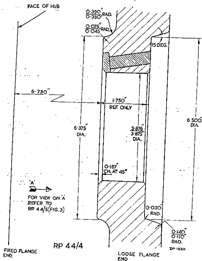
Fig. 2. Machining of bearing housings
