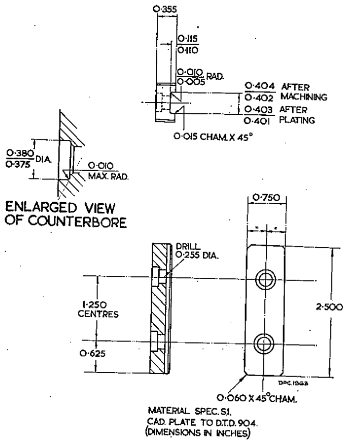
INNER DRIVE BLOCK RP.134/1 Fig. 1. Details of inner drive block
