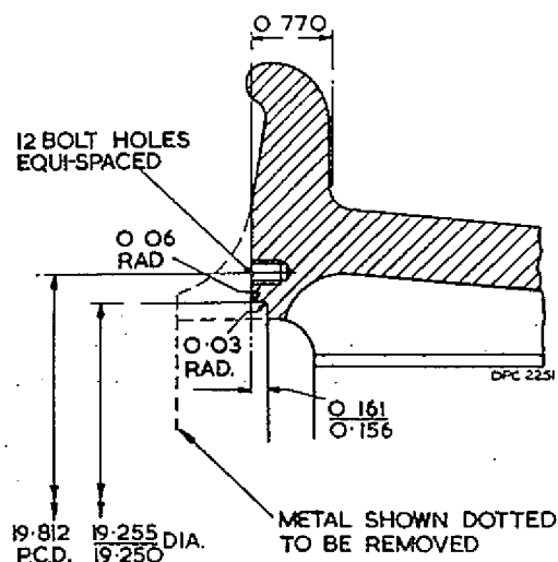
RP. 182/1 (DIMENSIONS IN INCHES)
