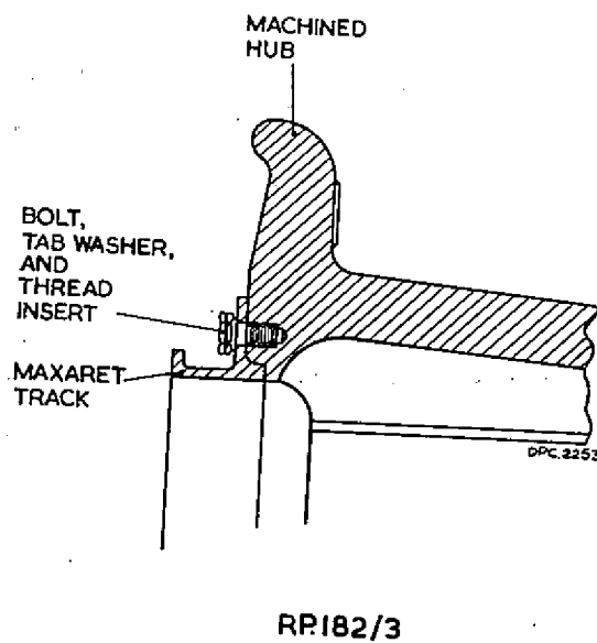
Fig. 3. Maxaret track assembled to wheel
