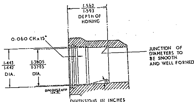
Fig. 1. Machining dimensions of cylinder bores
