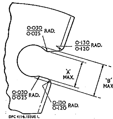
Fig. 2. Segment slots
