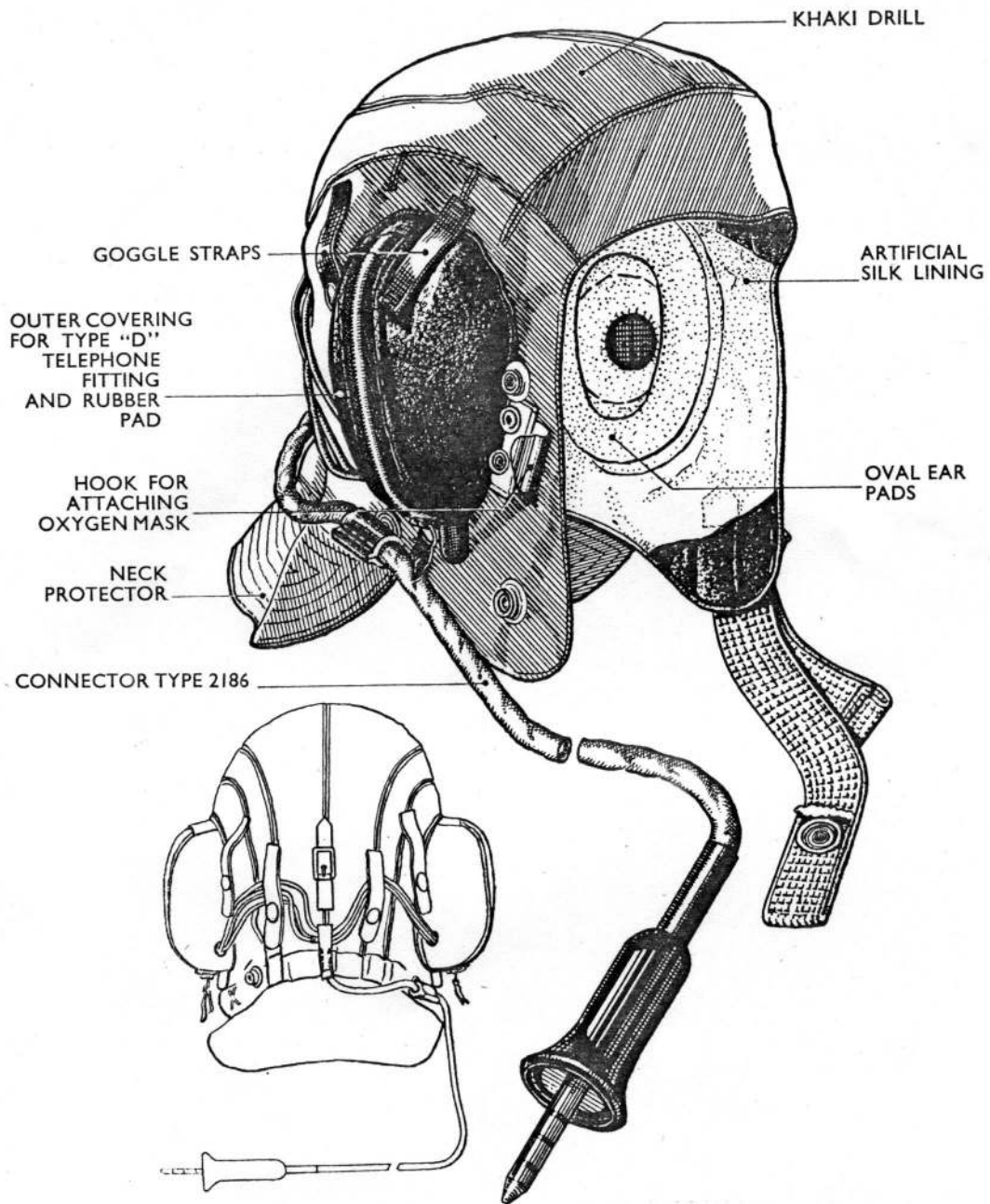
Fig. 9.—Type D wired naval helmet
