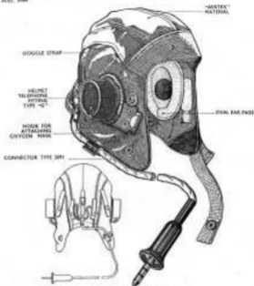
Fig. 4.—Type E wired helmet
