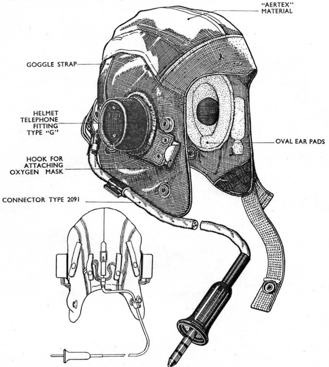
Fig. 6.—Type E wired helmet
