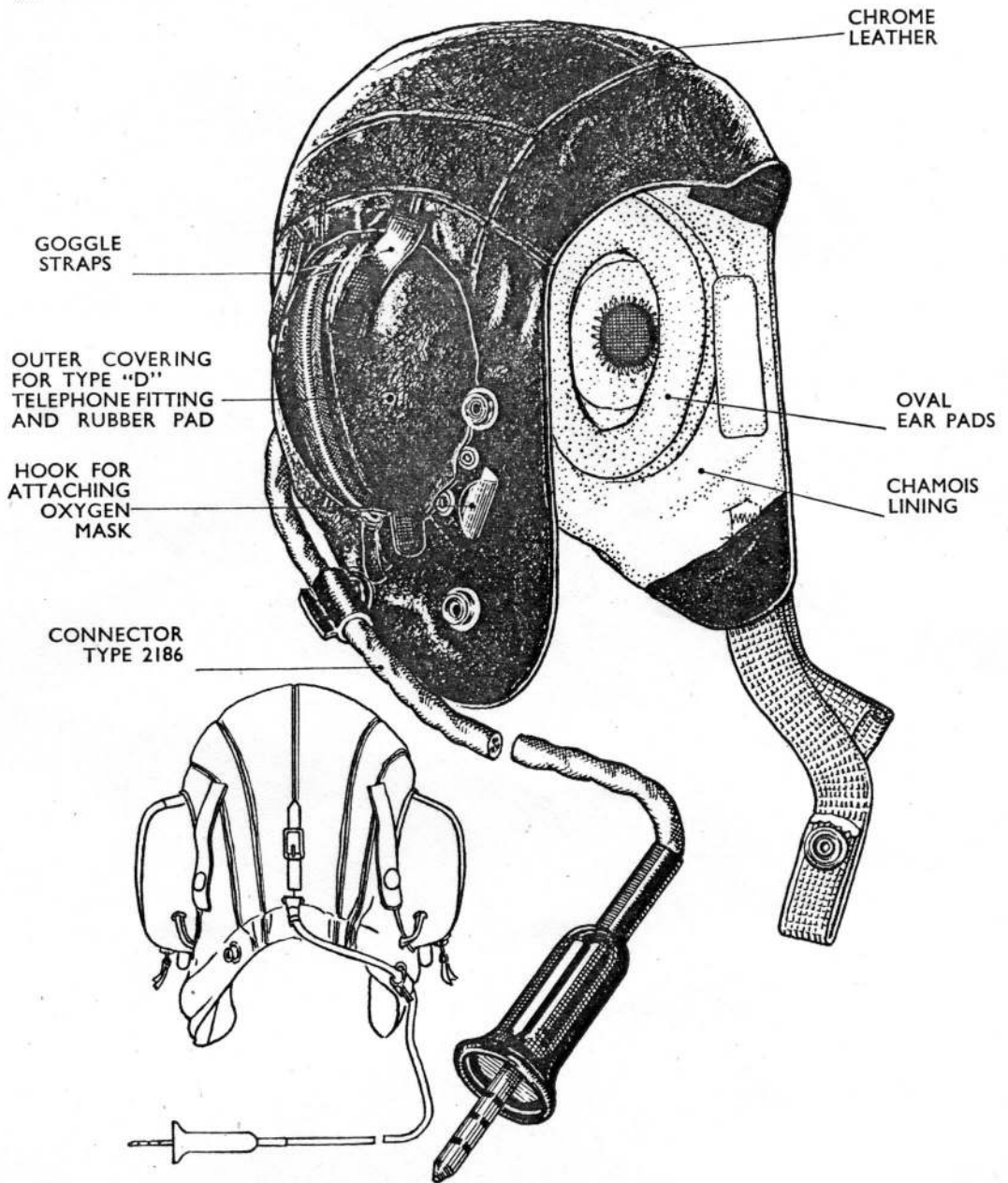
Fig. 8.—Type C wired naval helmet
