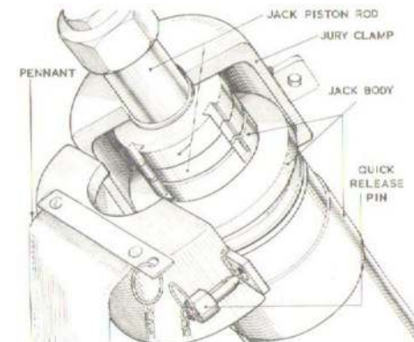
TAIL-WHEEL JURY CLAMP
