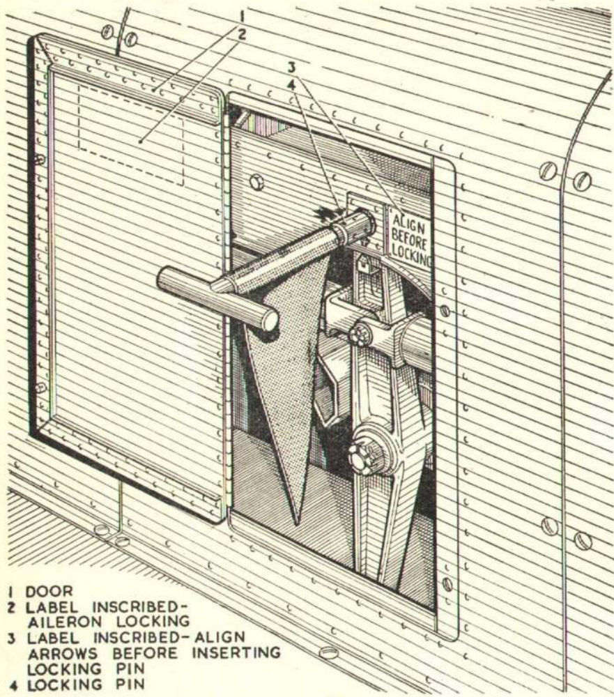
Fig. 8. Aileron locking
