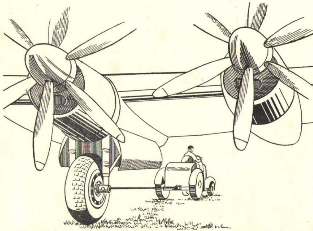
Fig. 6. Backward towing using bridle
