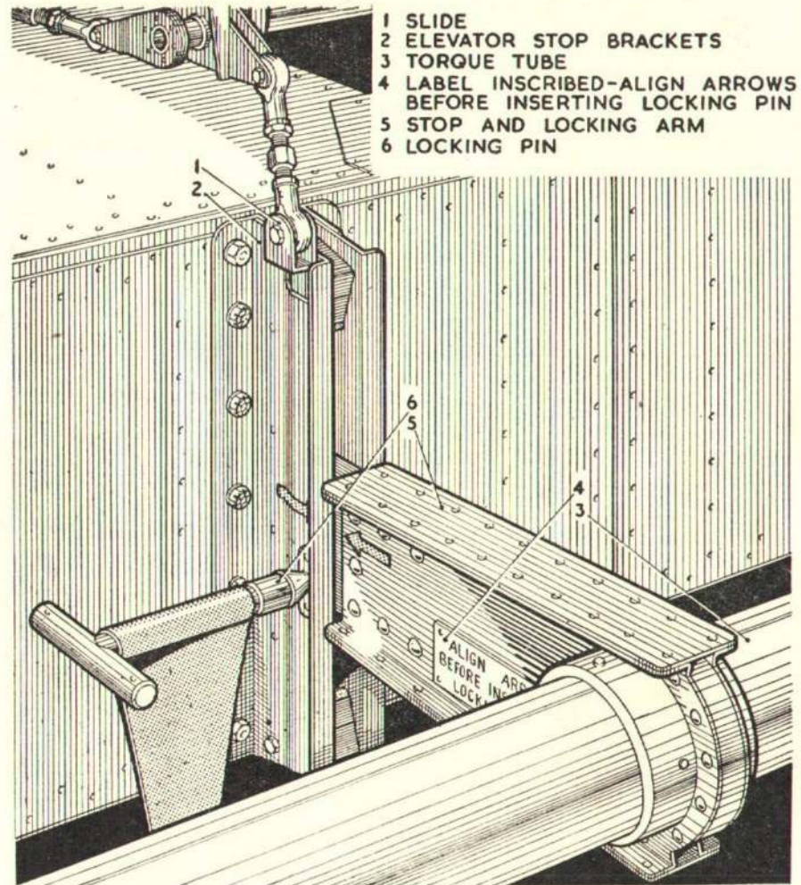
Fig. 9. Elevator locking
