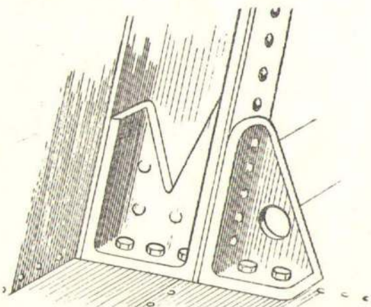
Fig. 7. Former—bomb floor joint
