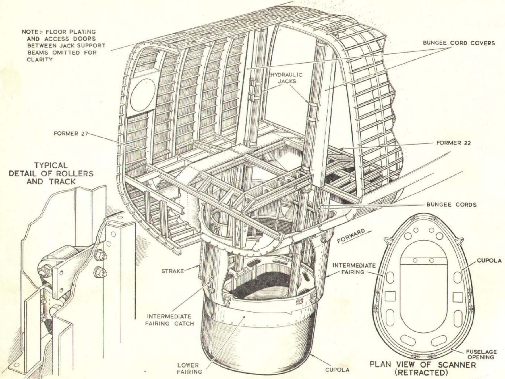
Fig. 19. Retractable scanner
