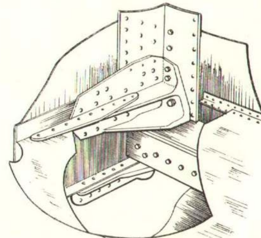
Fig. 13. Longeron—rear spar joint
