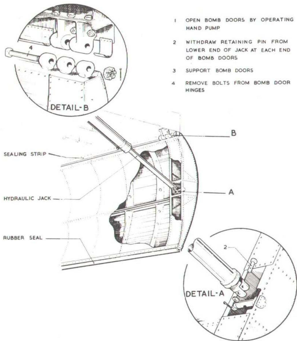
Fig.24. Removal of bomb doors
