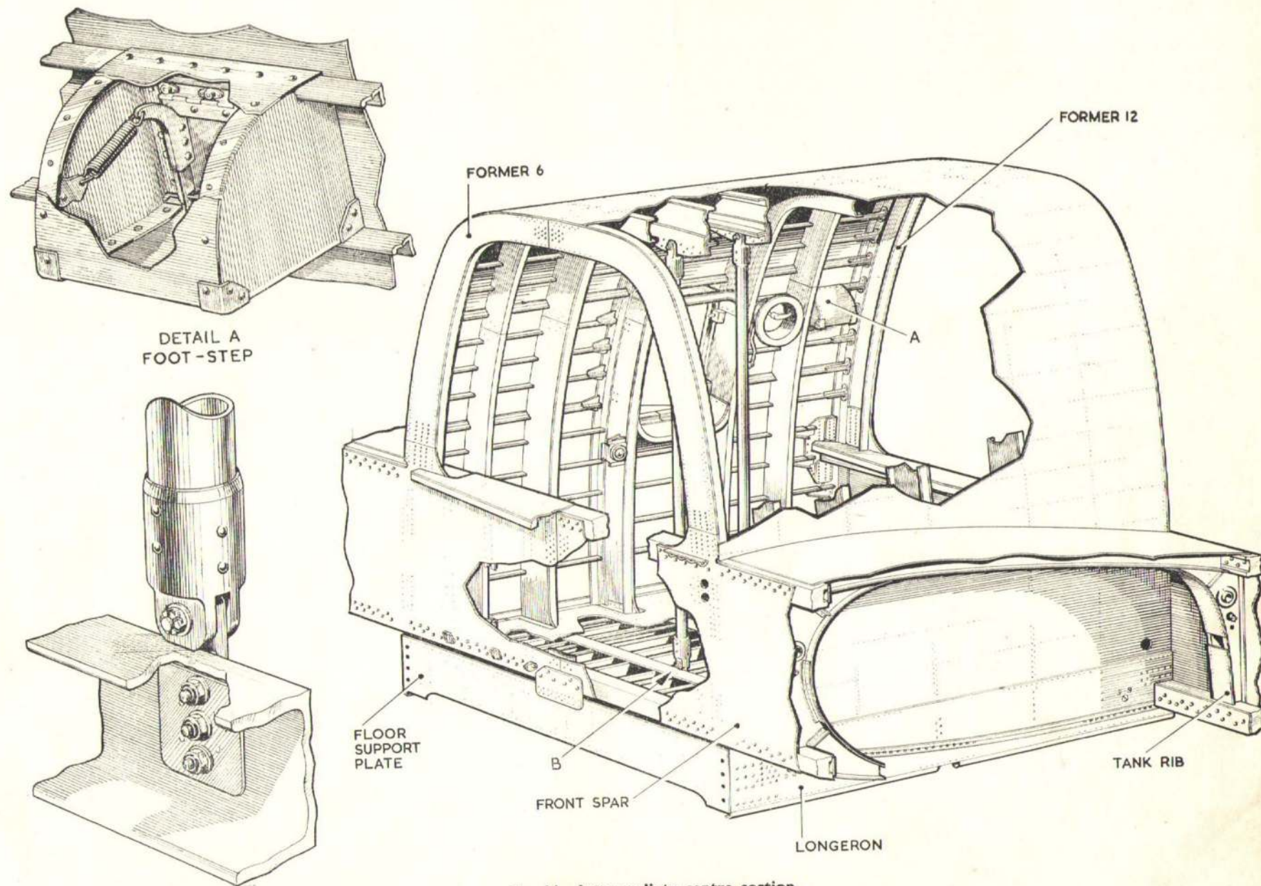
Fig. 14. Intermediate centre section
