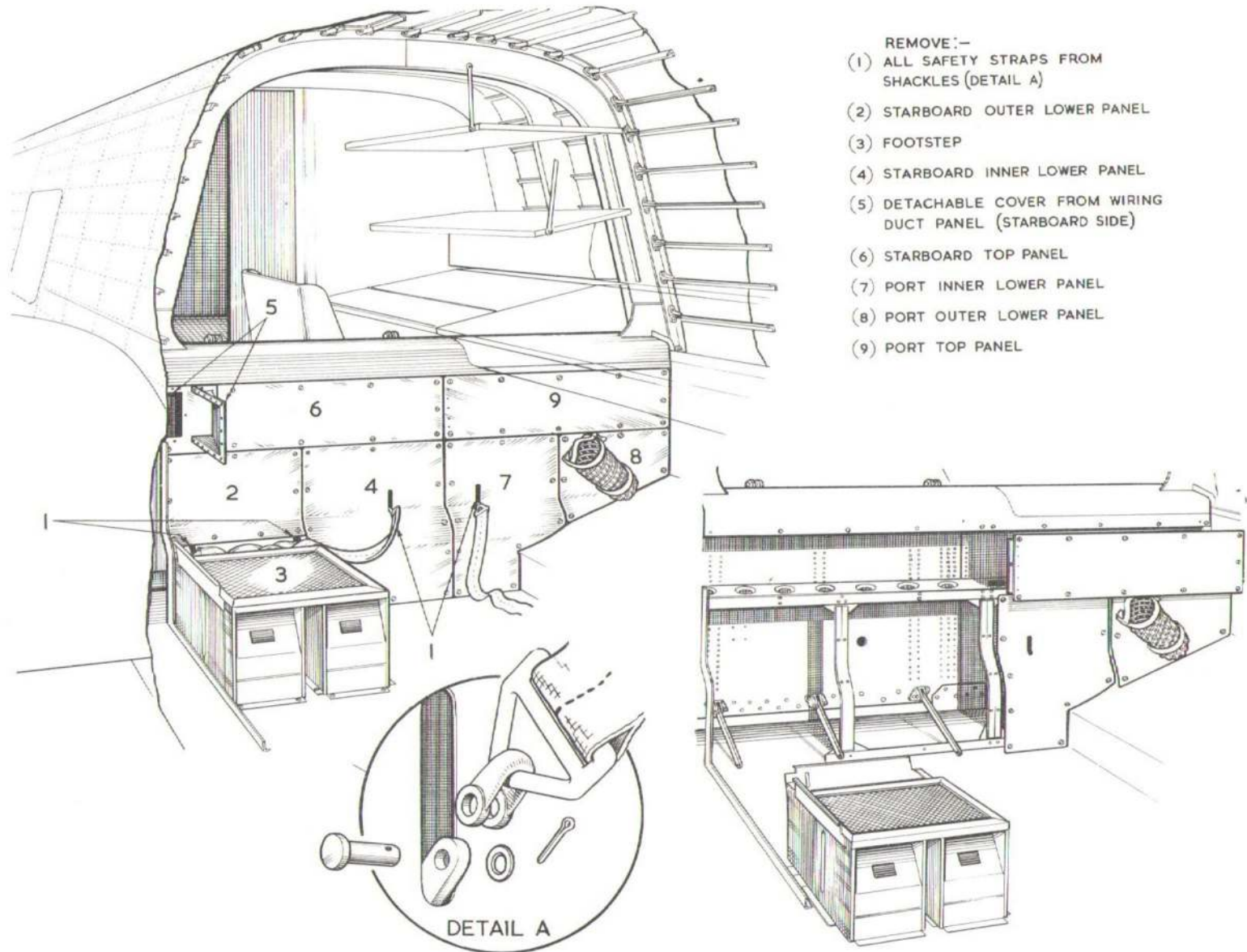
Fig.25. Removal of front spar covers.
