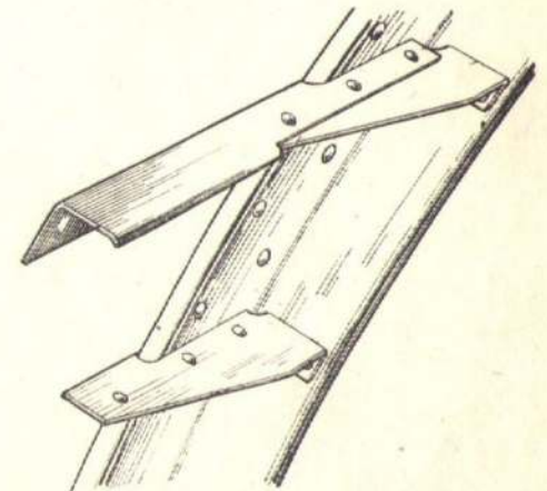
Fig. 4. Stringer—double former joint
