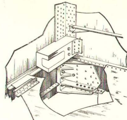
Fig. 12. Longeron—front spar joint
