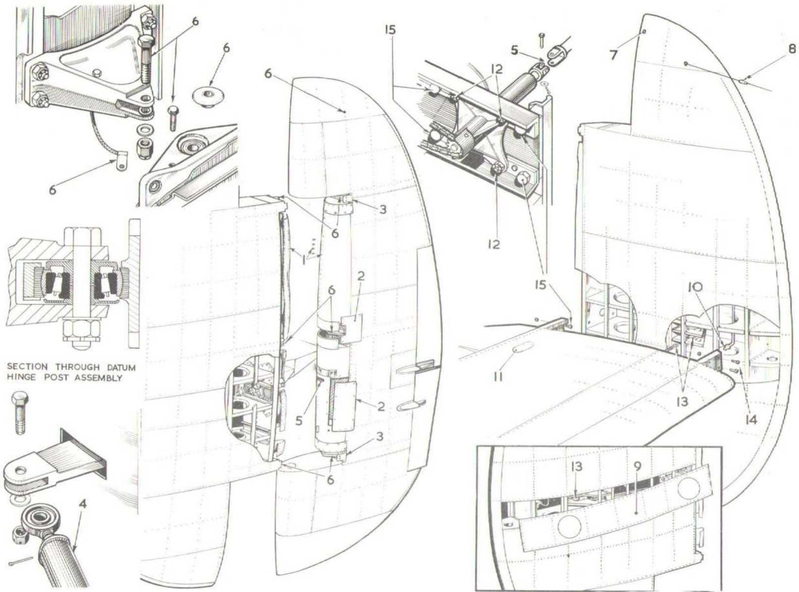
Fig. 4. Removal of rudder and fin RESTRICTED
