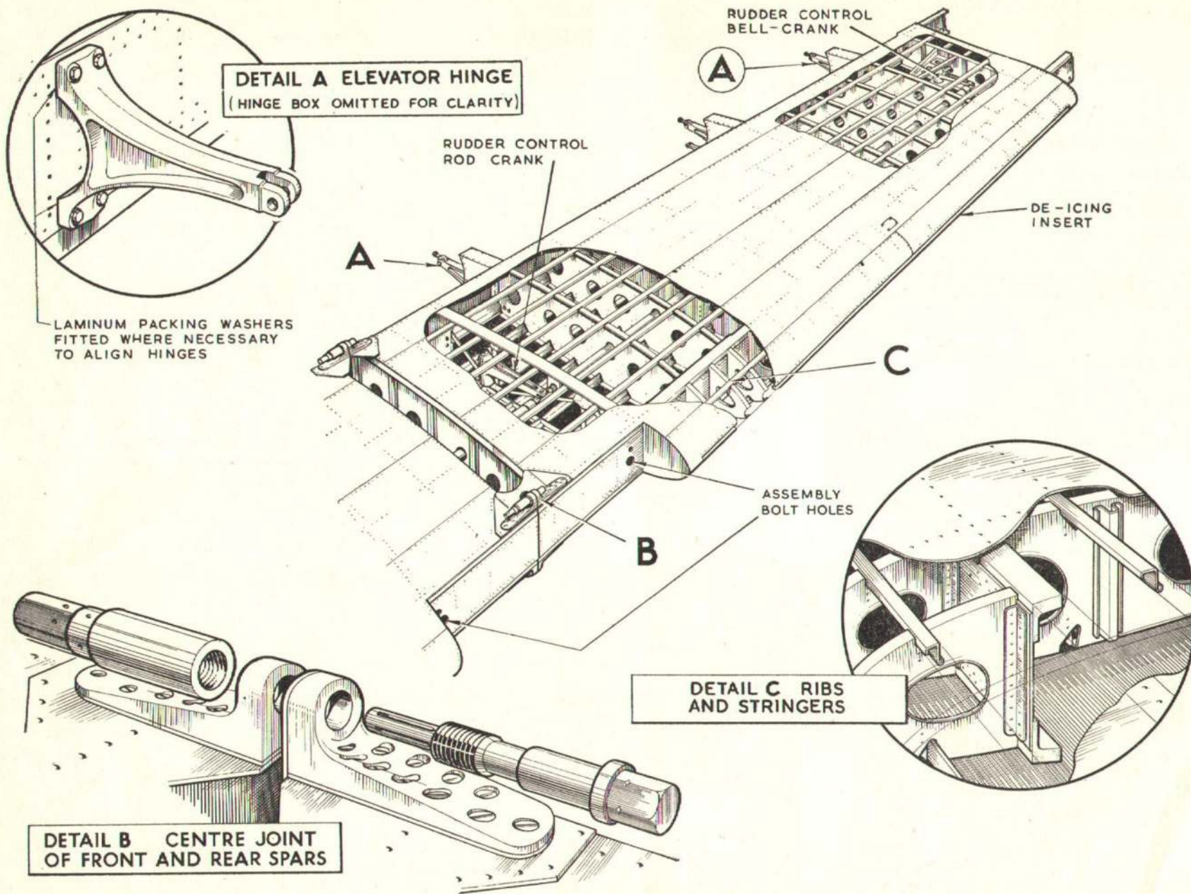
Fig. 1. Tail plane
