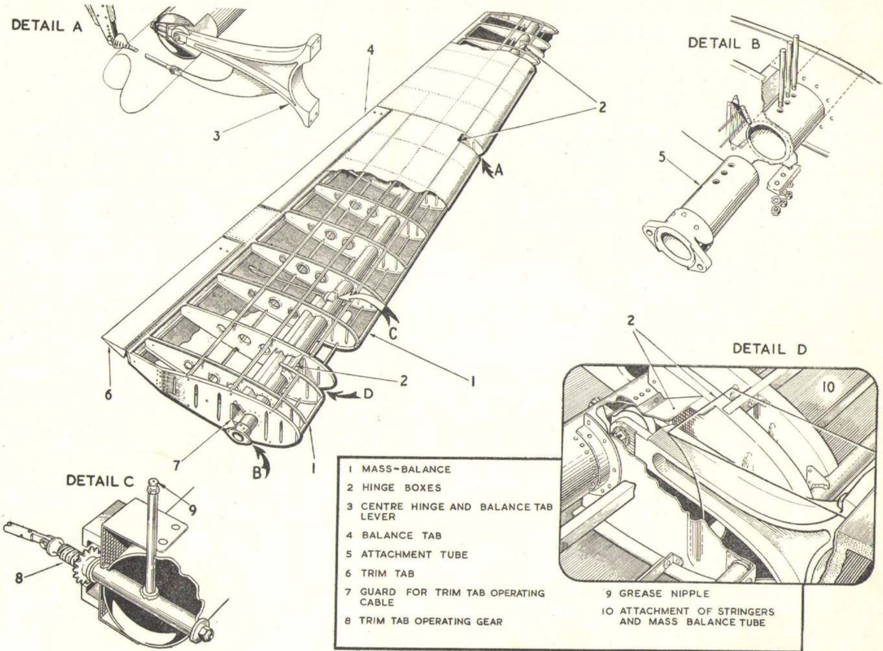
Fig. 3. Elevators
