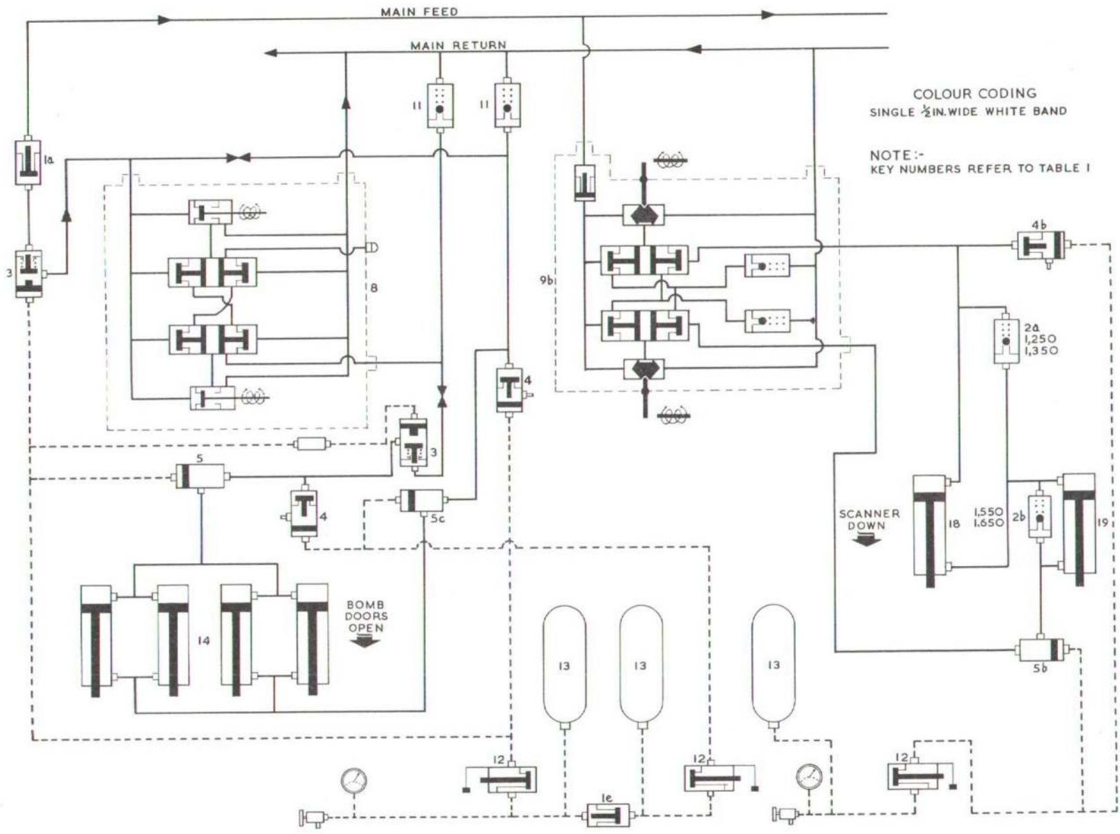
Fig.13. Hydraulic diagram (3) bomb doors and scanner (Amendment to piping) RESTRICTED
