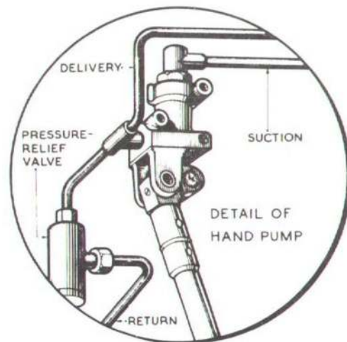
Fig.1. Hand pump
