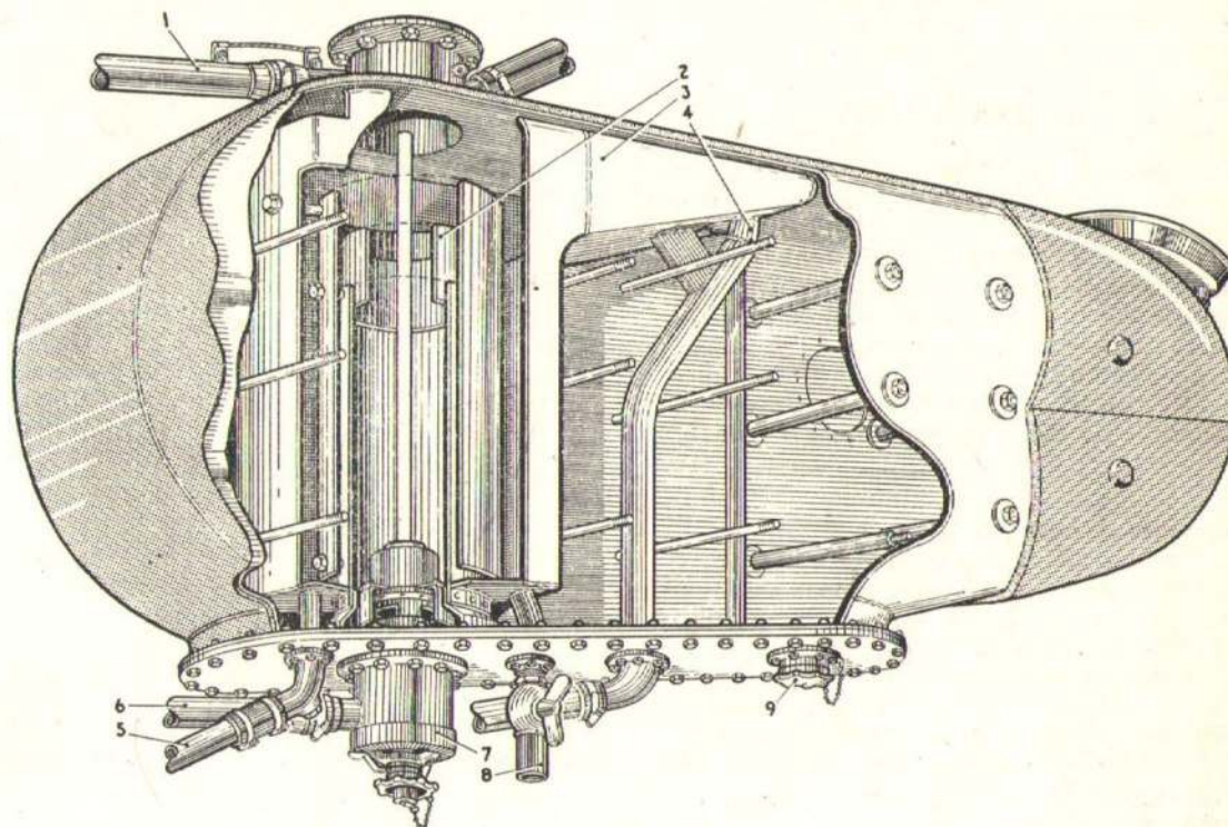
Fig. 1. Oil tank—inboard
