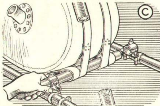
Fig. 10. Removal of outboard oil tank
