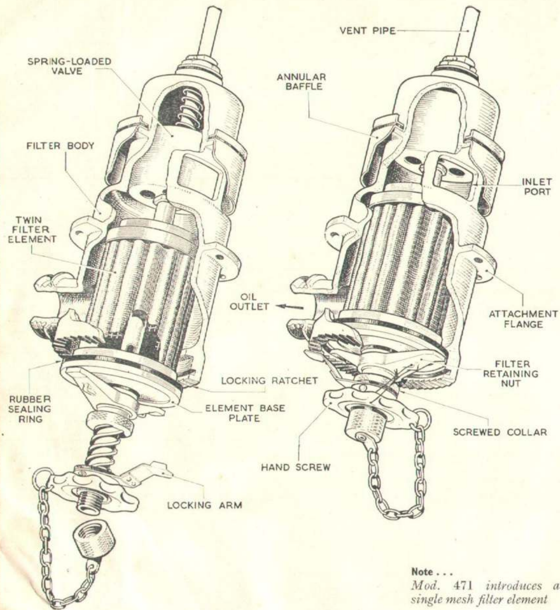
Fig. 4. Oil filter unit
