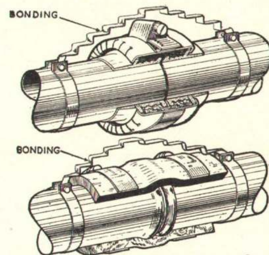
Fig. 7. Typical oil pipe connections
