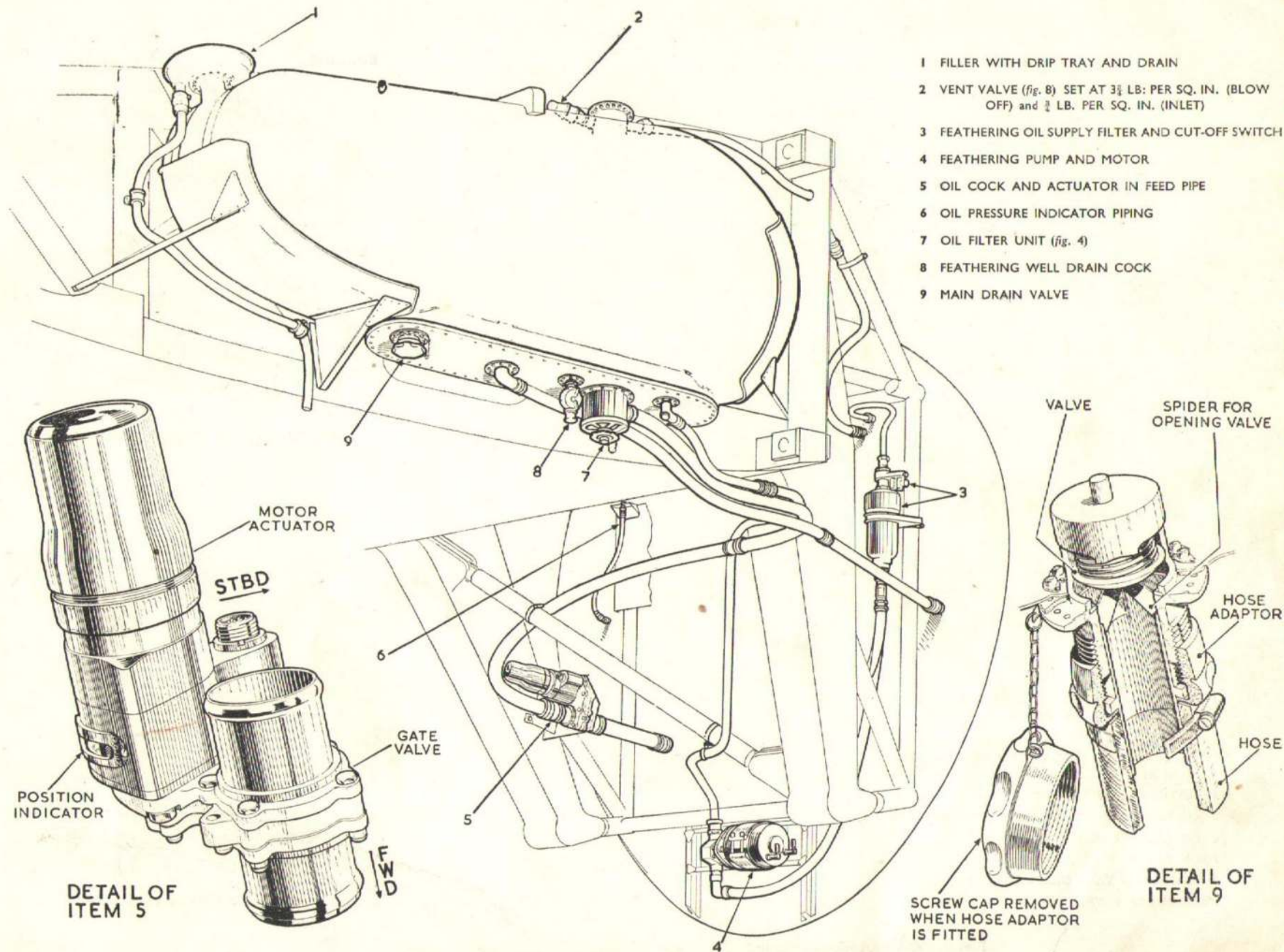
Fig. 5. Oil system—inboard
