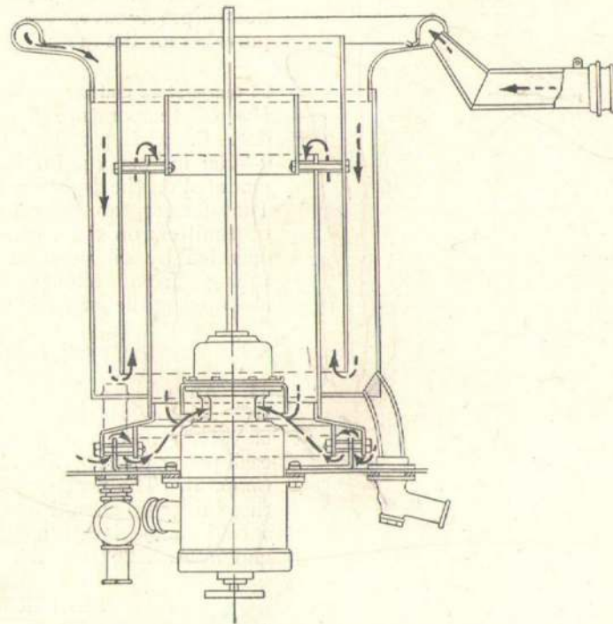
Fig. 3. Tank oil movement
