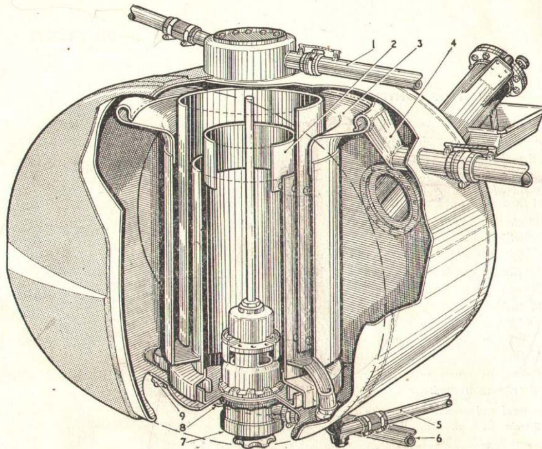
Fig. 2. Oil tank—outboard
