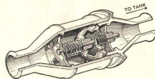
Fig. 8. Section of vent valve
