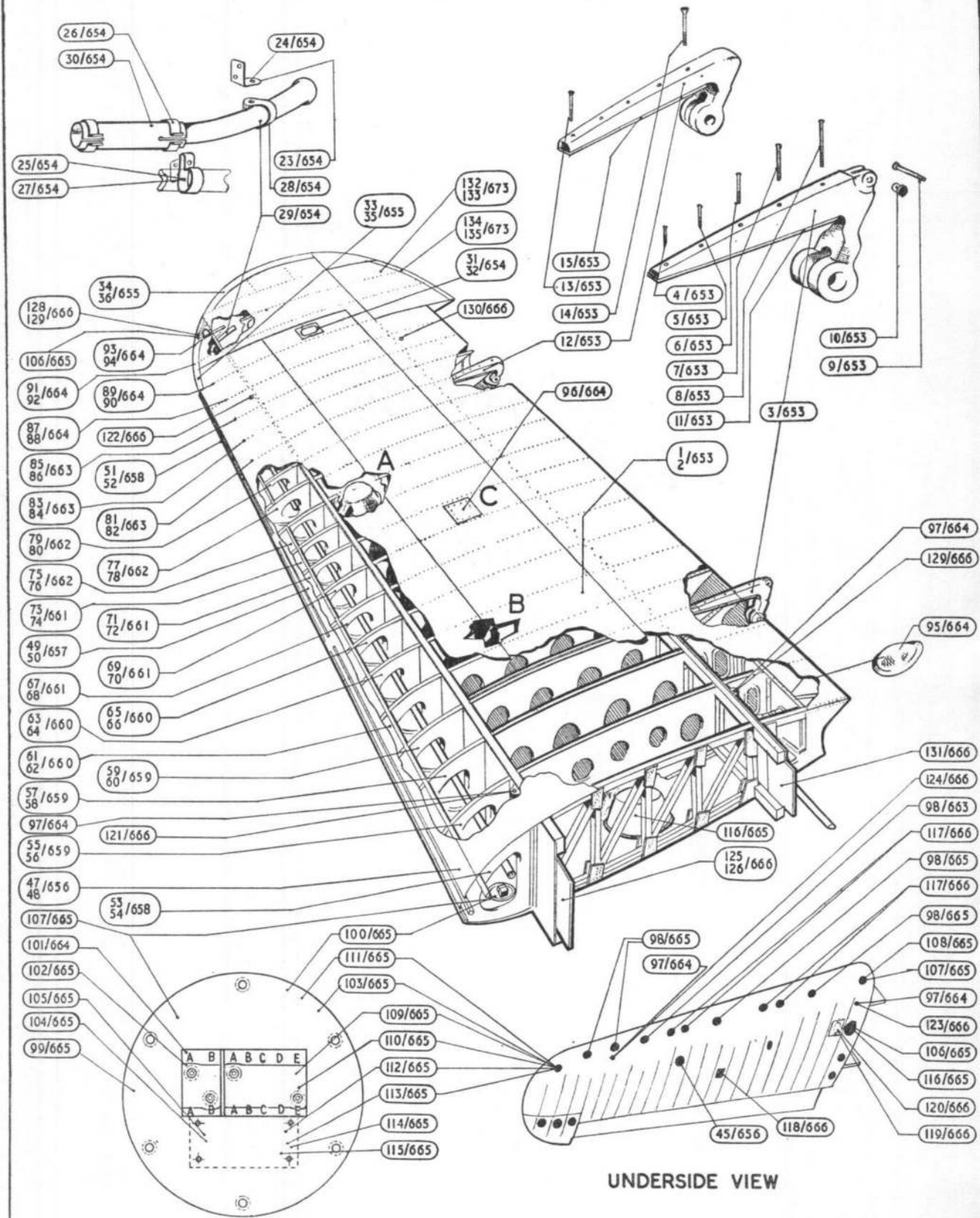
OUTER MAIN PLANE (I)
