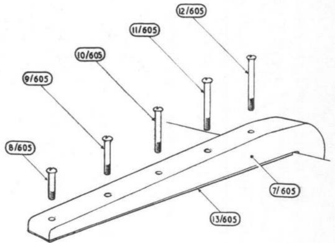
AILERON HINGE AT A
