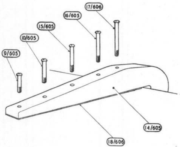
AILERON HINGE AT B
