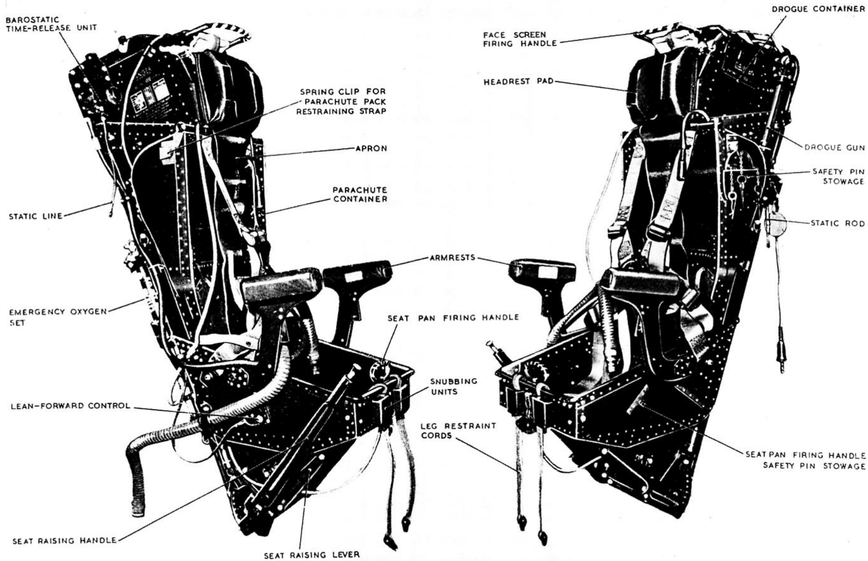
Fig. 1. Ejection seat, Type 3L/1, Mk. 1
