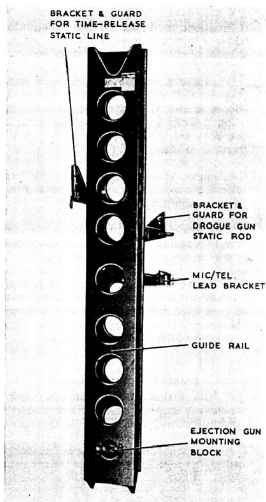
Fig. 6. Guide rail
