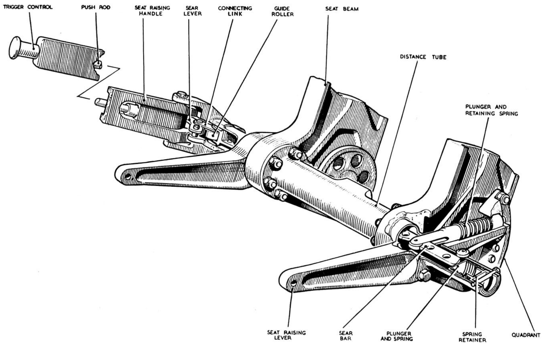
Fig. 4. Details of seat raising mechanism
