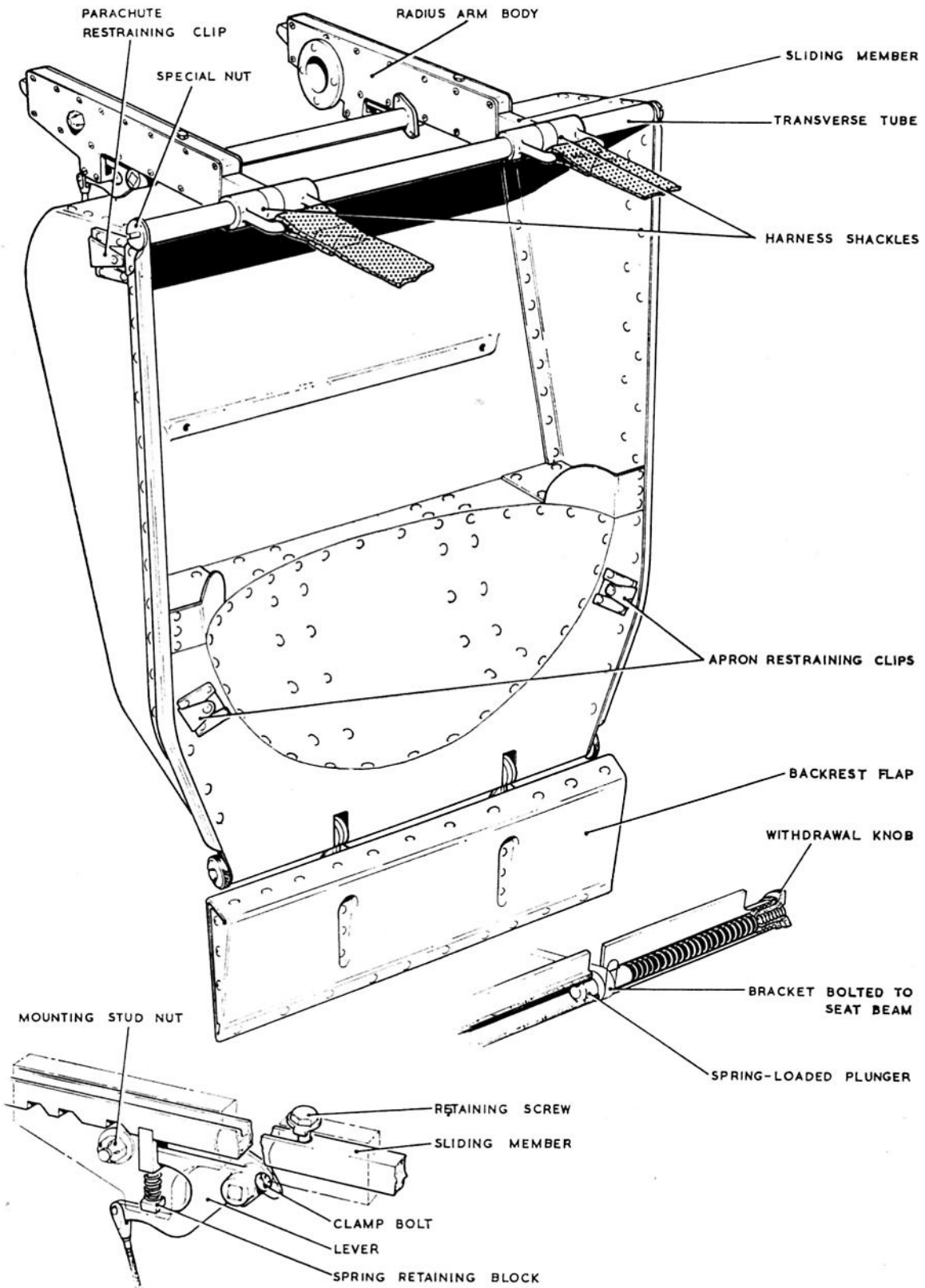
Fig. 5. Details of parachute container control
