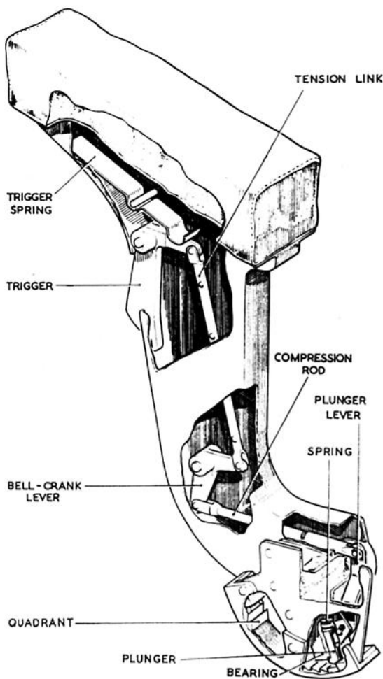
Fig. 3. Details of armrest
