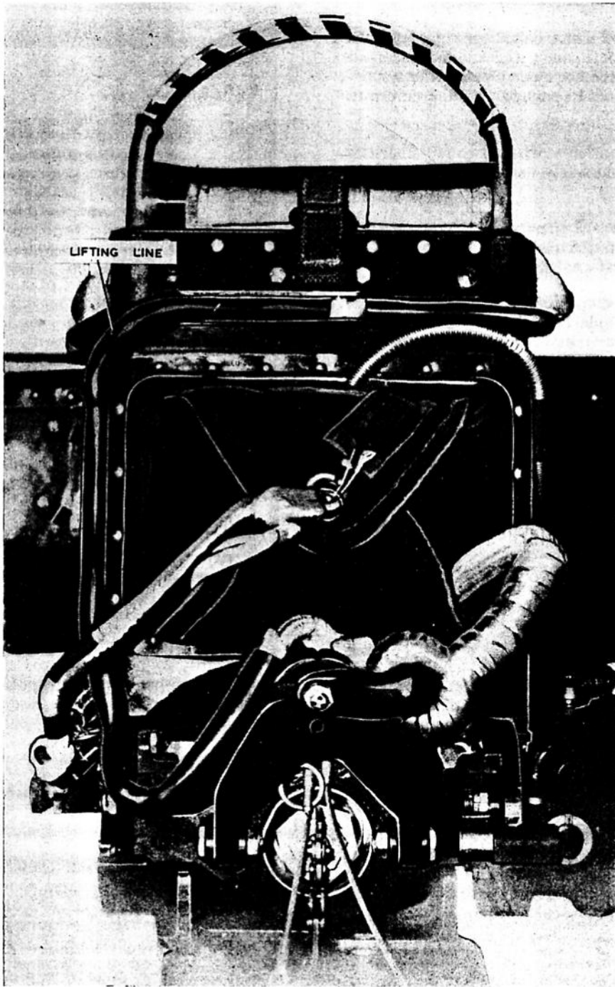
Fig. 7. Fitting the lifting lines
