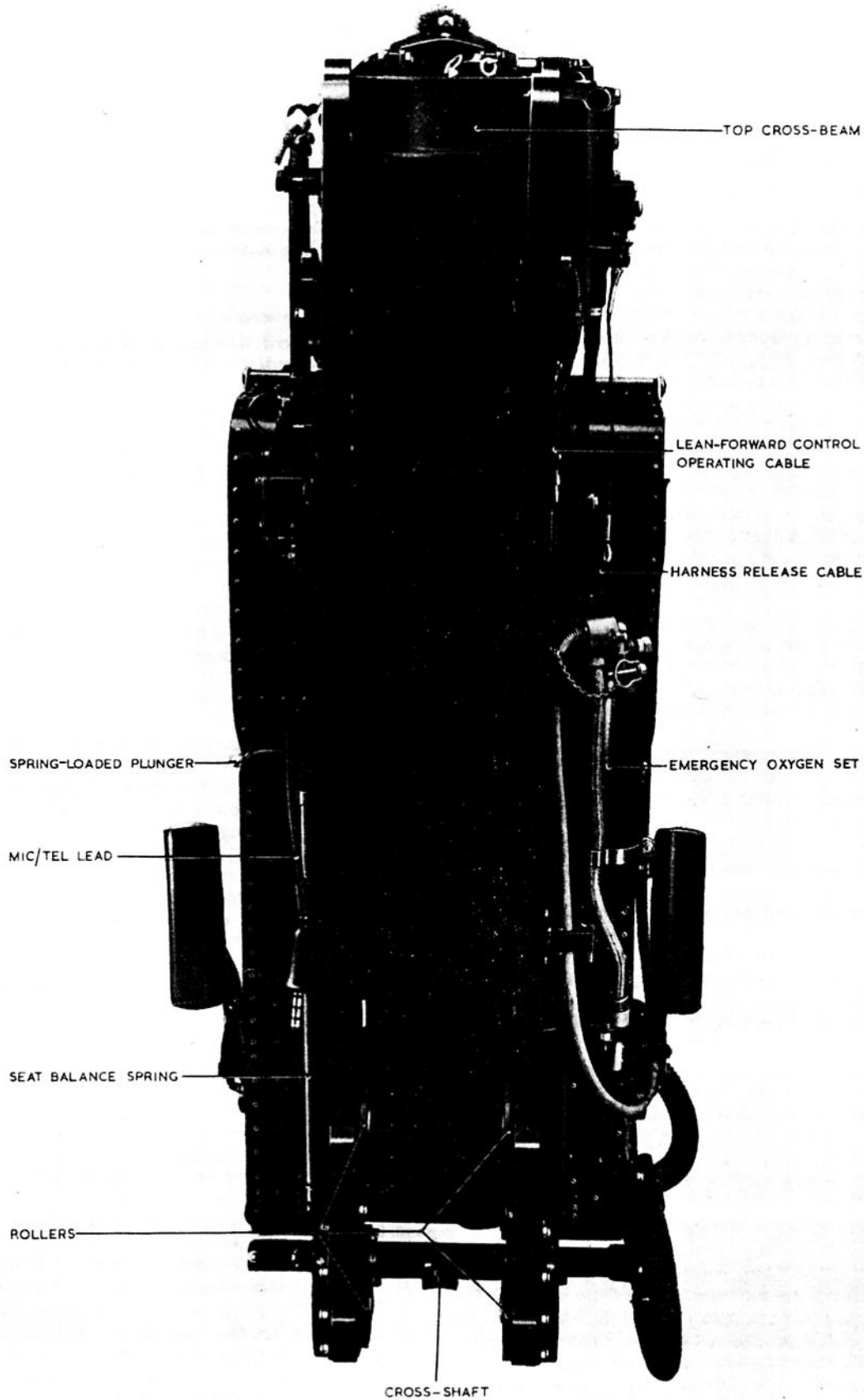
Fig. 2. Seat structure
