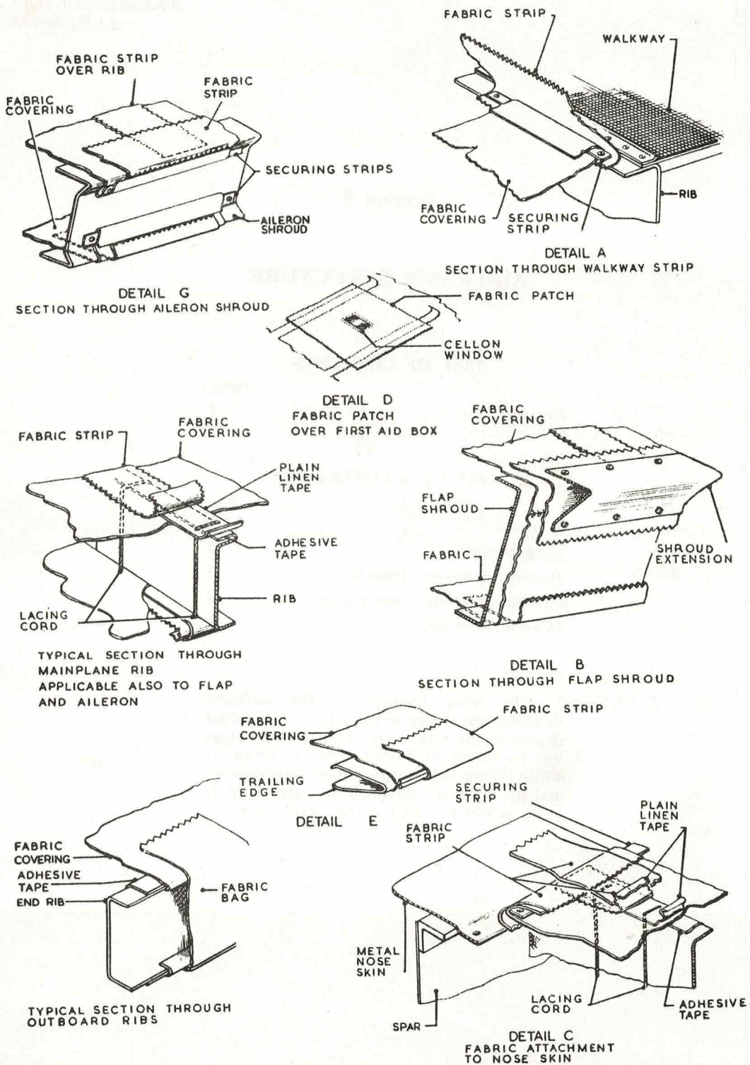
Fig. 1. Wing covering details
