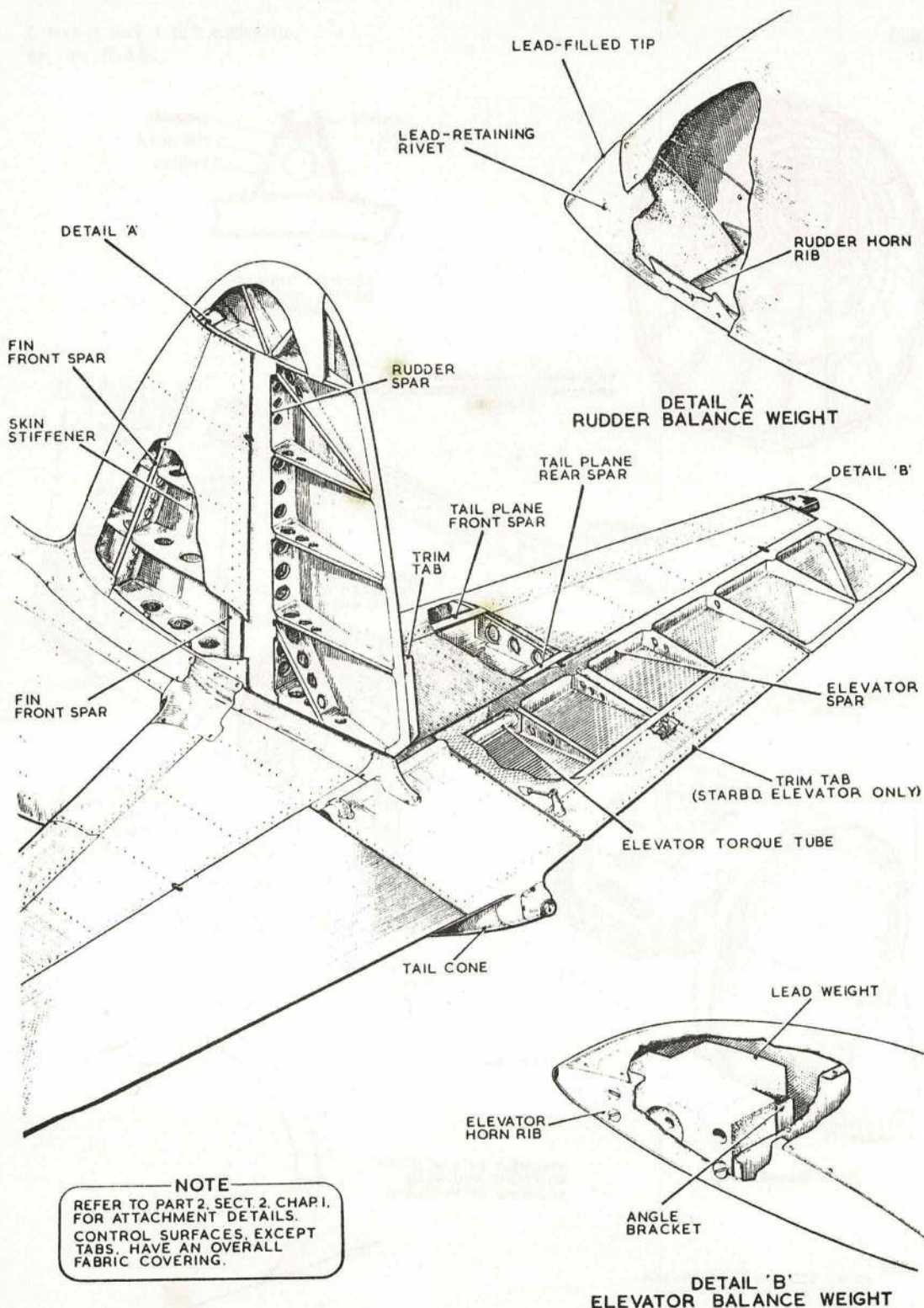
Fig. 5. Tail unit structure
