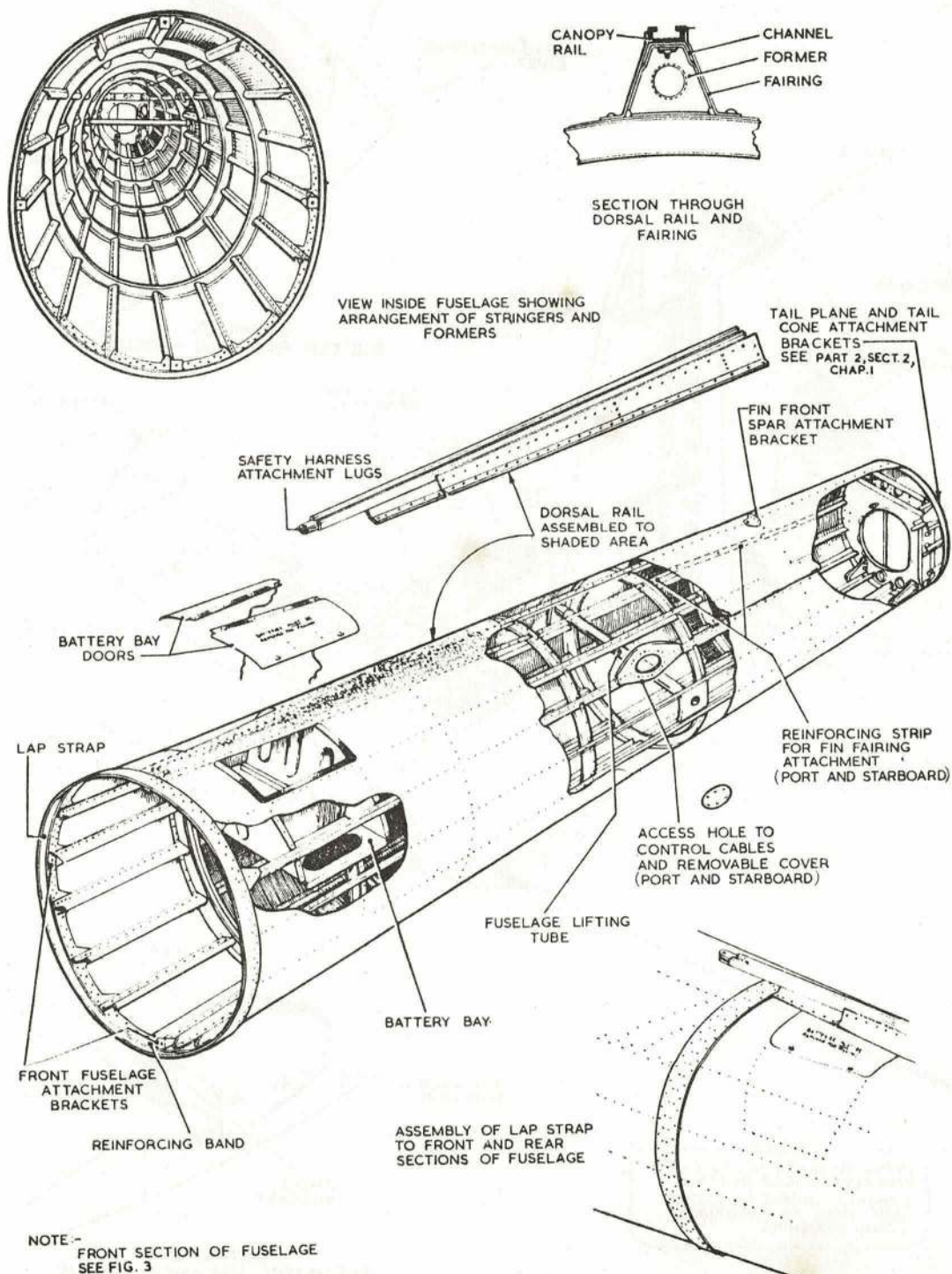
Fig. 4. Fuselage structure—rear section
