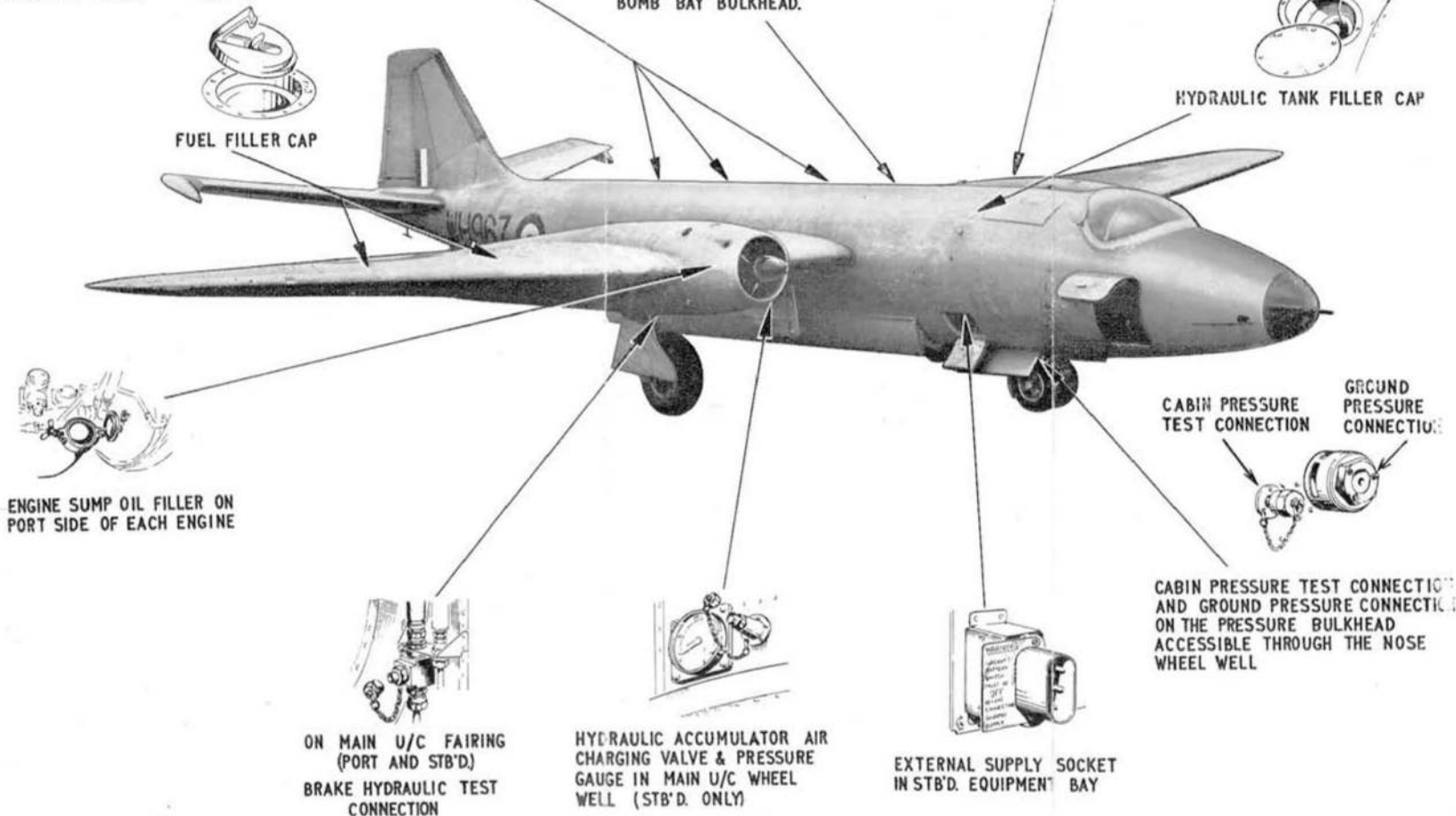
HYDRAULIC ACCUMULATOR (BRAKES) AIR CHARGING VALVE AND PRESSURE GAUGE ON REAR FACE OF FORWARD BOMB BAY BULKHEAD.
