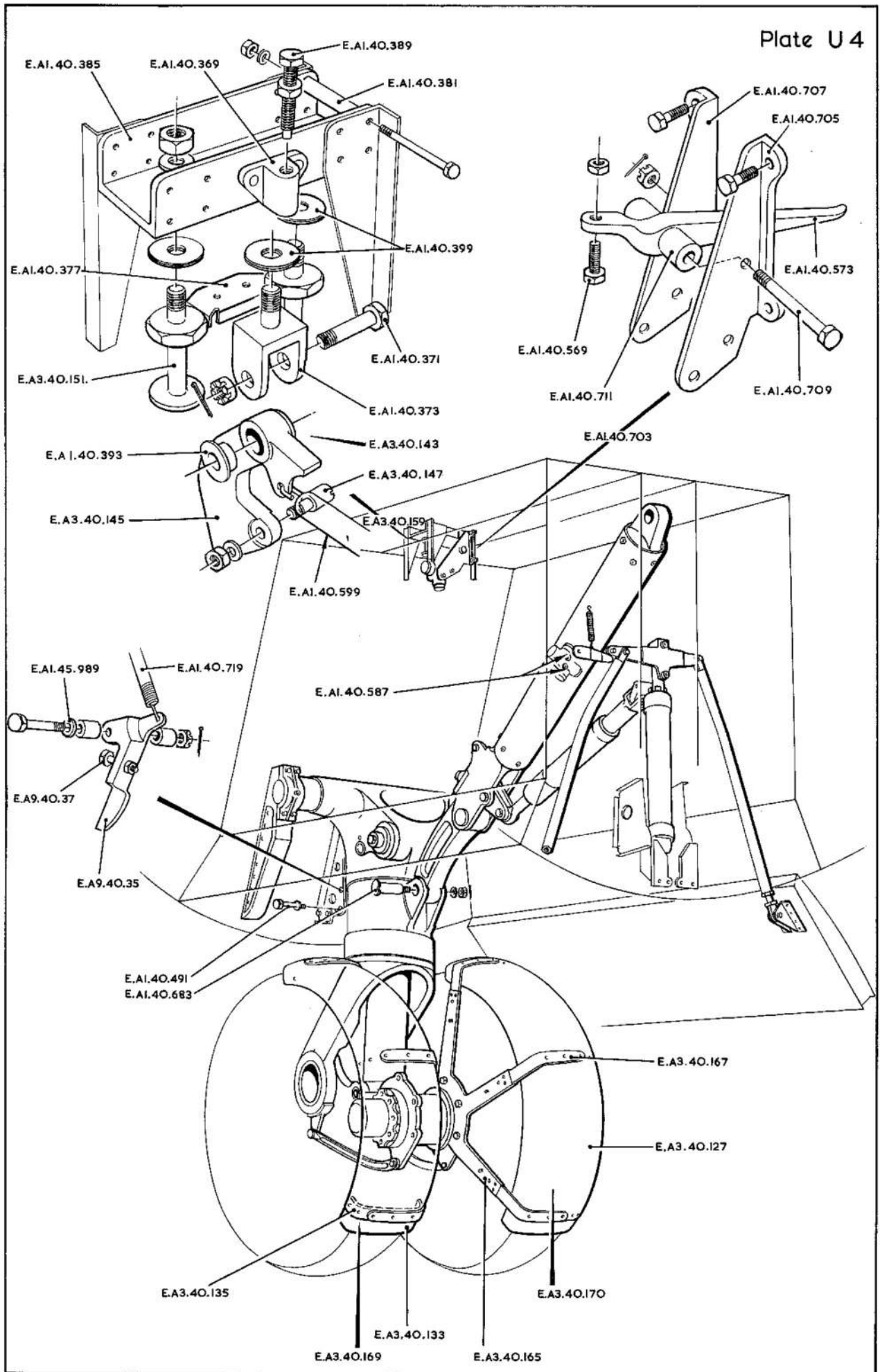
NOSE UNDERCARRIAGE
