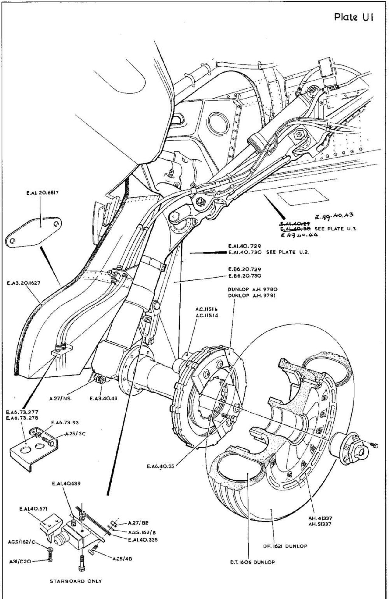
MAIN UNDERCARRIAGE
