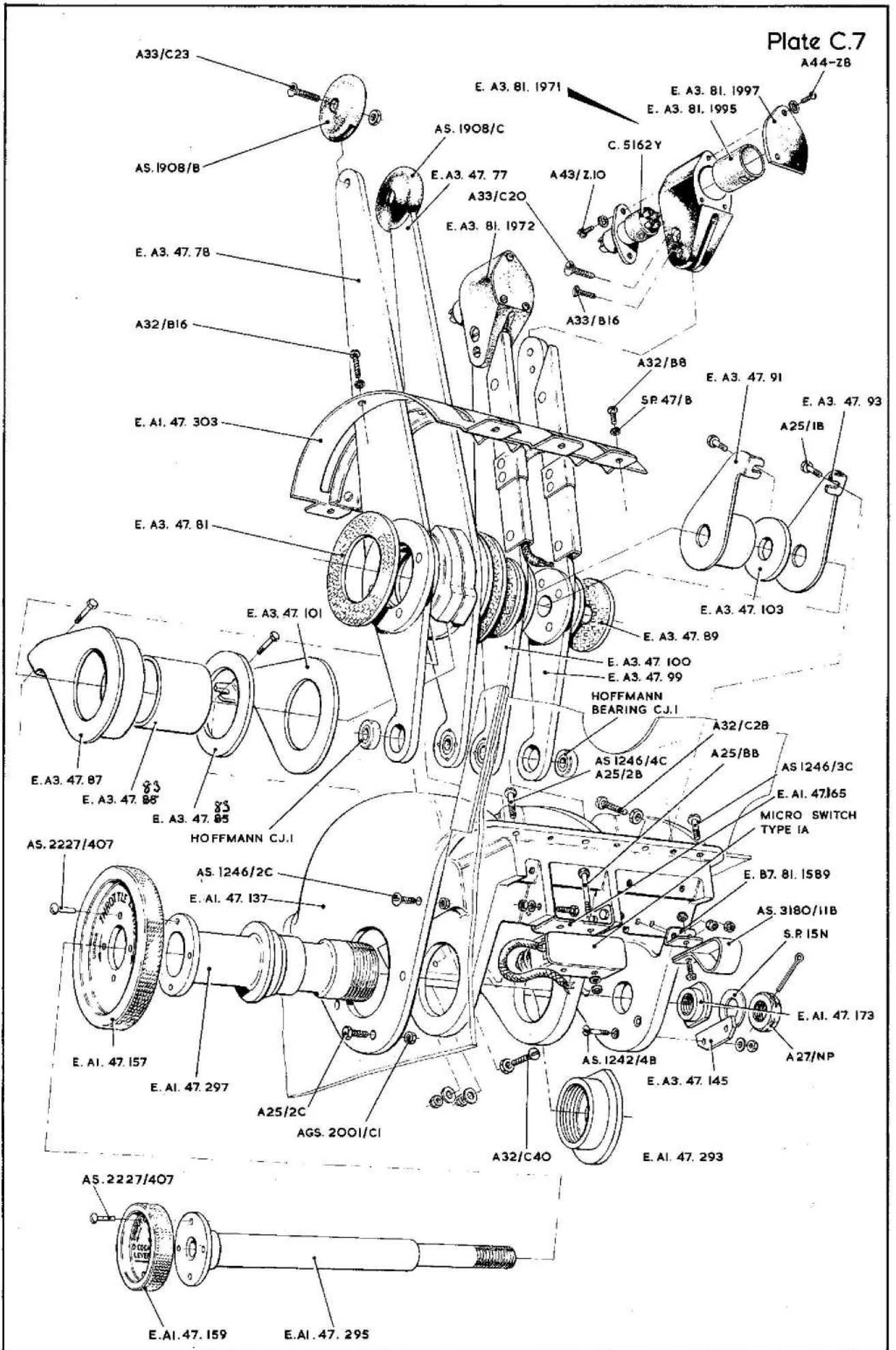
PILOTS THROTTLE BOX
