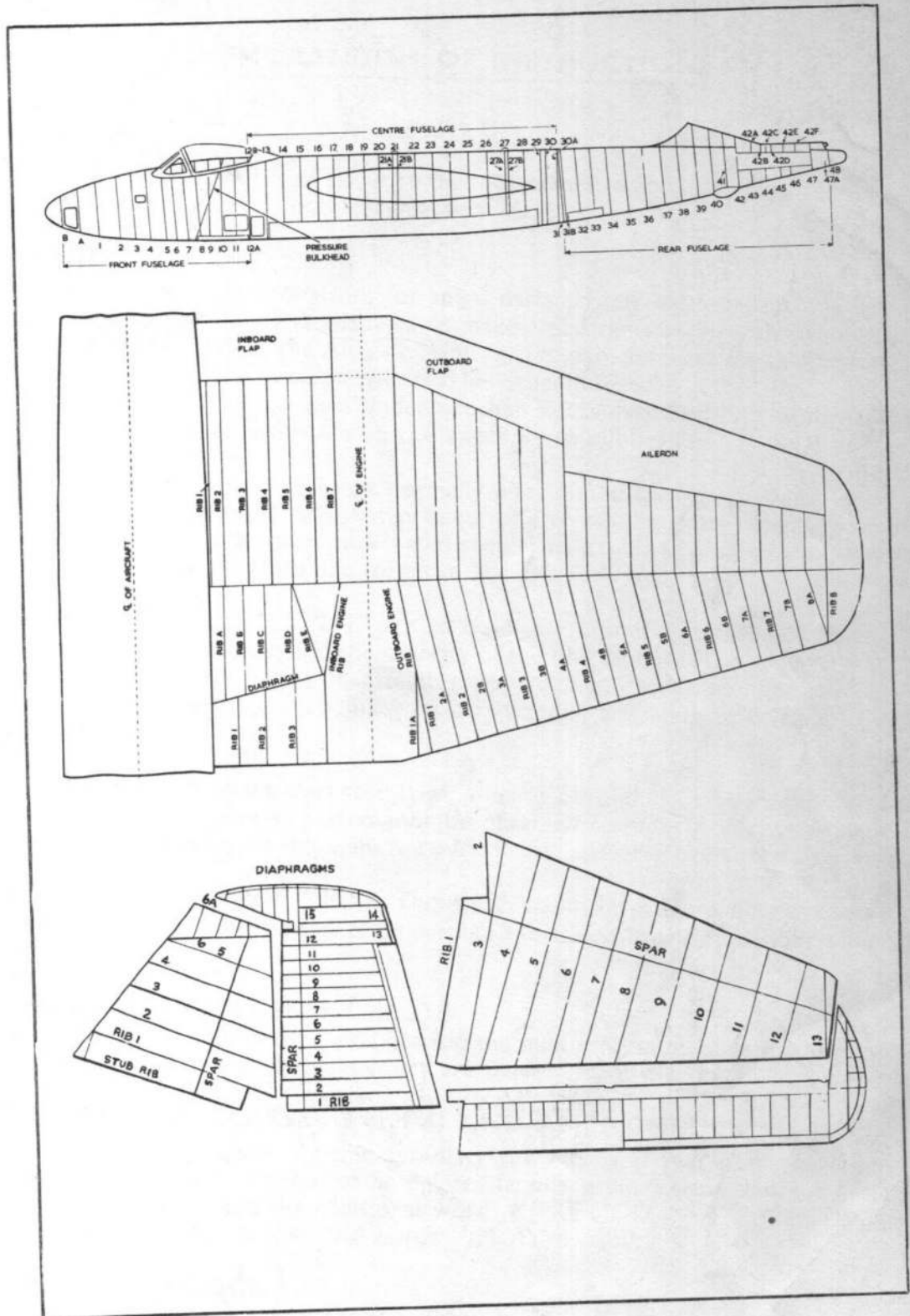
KEY DIAGRAM OF RIB AND FRAME POSITIONS
