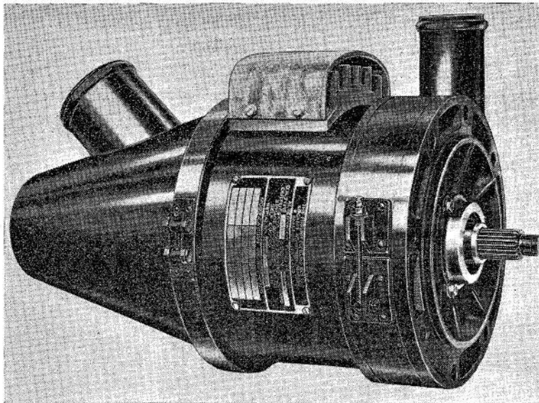
Fig. 1. Generator, Type 163
