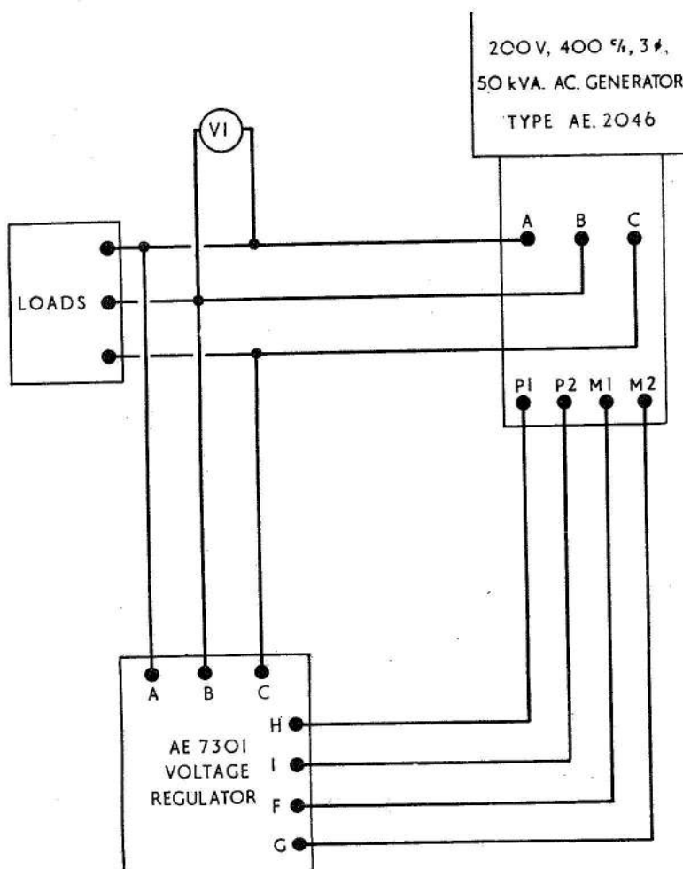
Fig. 5. Test circuit
