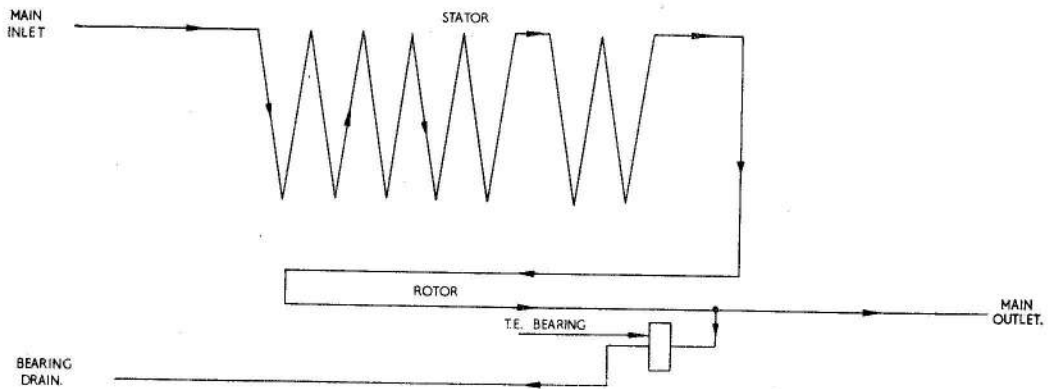
Fig. 3. Oil circuit
