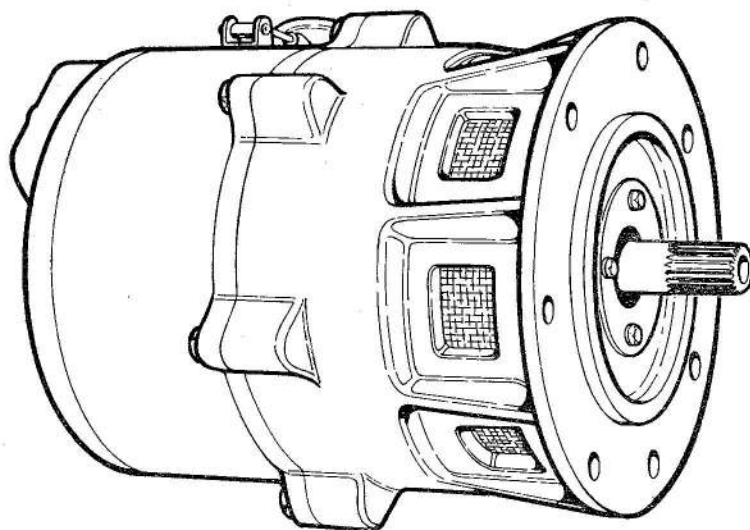
Fig. 1. General view of Type N0504 generator
