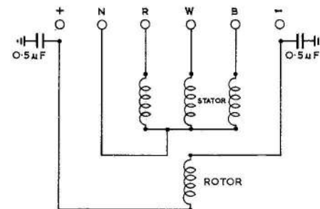
Fig. 3. Circuit diagram
